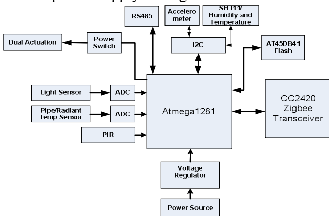
Figure 1: Block diagram of the WSN mote
