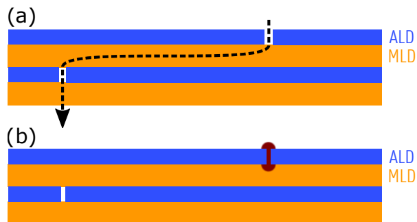
Figure 1: Conceptual explanation of the use of ALD-MLD layer structures as effective water barrier coatings thanks to (a) longer moisture diffusion pathways upon cracking of the ALD films and (b) slowing down the water transmission through the cracks based on the desiccant effect of the MLD films.
