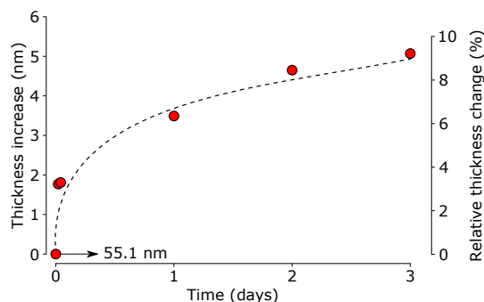
Figure 12: The thickness evolution of GL-grown magnesicone film thickness with a starting thickness of a 55.1 nm, as stored in ambient laboratory conditions. After only 3 days of exposure, the film thickness increased as much as 9.2%. The dashed line is a guide to the eye.
