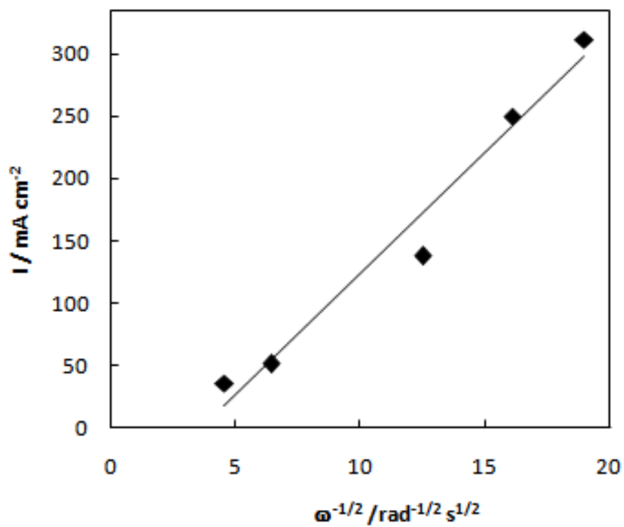
Figure 6. Levich plot for low potential wave for NPG-coated Au disc in 1 M NaOH containing 20 mM AB at 10 \text{ mV s}^{-1} .
