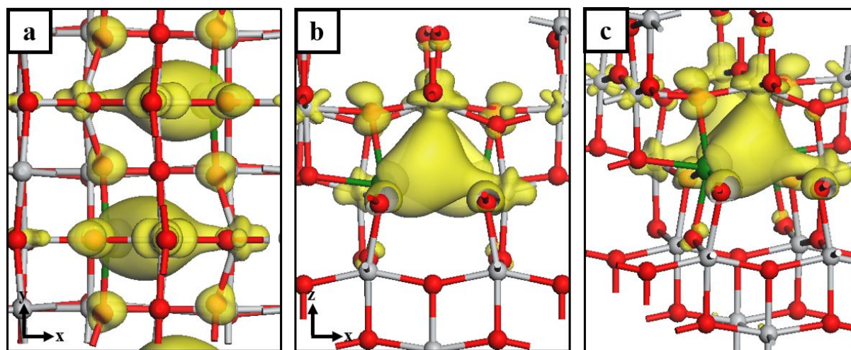
8 9 10 11 12 13 14 15 16 17 18 19 20 21 22 23 24 25 Fig. 3 Excess spin density plot showing the localization of electrons after formation of a 26 second, reducing oxygen vacancy in In-doped anatase TiO 2 . Panels (a), (b) and (c) display 27 the geometry in the xy-plane, xz-plane and from an angled view. The yellow isosurface 28 encloses spin densities up to 0.02 electrons/Å 2 29 30 31 32
