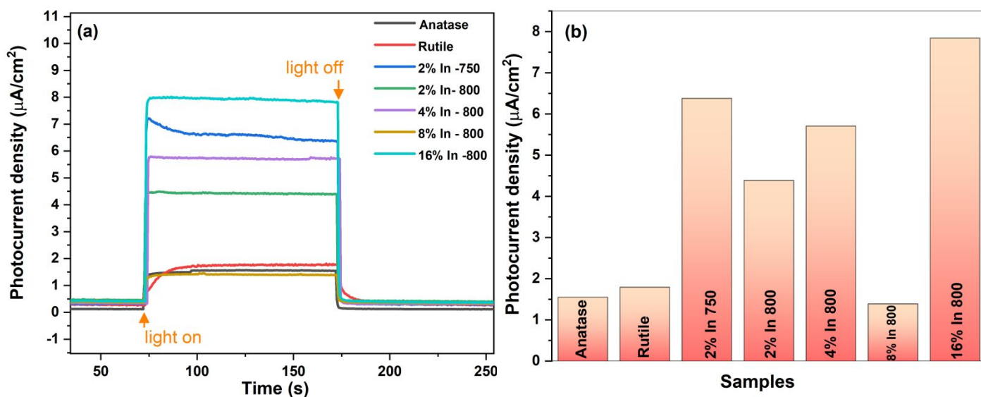
Fig. 12. (a) The photocurrent density of anatase, rutile and various In- \text{TiO}_2 samples at +1.0 V vs SCE, and (b) steady state photocurrent density of anatase, rutile and various In- \text{TiO}_2 samples at +1.0 V.
