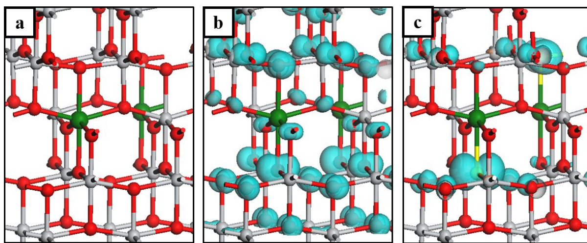
17 18 19 20 21 22 23 24 25 26 27 28 29 30 31 32 33 Fig. 1 Panel (a) shows the positions of In-dopant in the anatase lattice. Panel (b) shows the excess 34 spin density plot for the computational set up with no +U correction on the O 2p states. Panel (c) 35 shows the excess spin density plot for the computational set up with an additional +U correction on 36 the O 2p states and for which the geometry was distorted from symmetry prior to relaxation. Ti is 37 represented by grey spheres, O by red spheres, In by green spheres and the oxygen hole polarons ( O^- ) 38 are highlighted in yellow. The blue iso-surface encloses spin densities up to 0.02 electrons/Å 2 .
