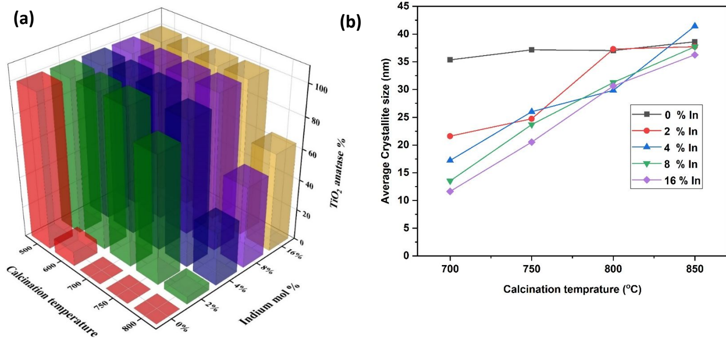
Fig. 8. (a) The anatase phase percentage of In-TiO 2 samples at various calcination temperature (b) the average crystallite size of In-TiO 2 at various calcination temperatures
