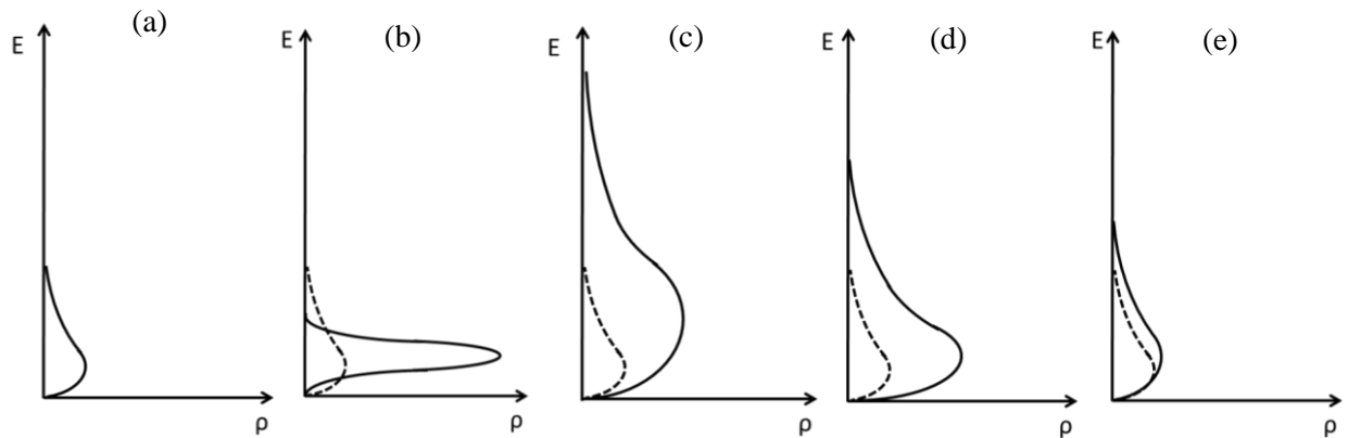
Fig. 2.2.8: Evolution of the electron distribution in the conduction band before and after the arrival of a pump pulse. (a) Initial undisturbed distribution, (b) spectral hole burning, (c) carrier heating, (d) carrier cooling and (e) carrier sweepout from the intrinsic region.
