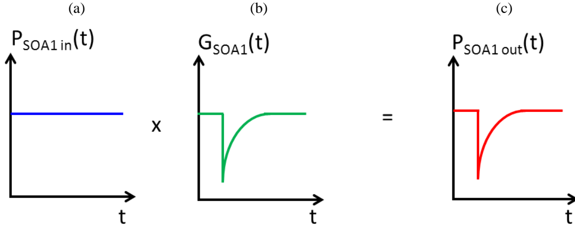
Fig. 2.1.13: (a) CW probe input to SOA1, (b) gain dynamics of SOA1 in response to the pump pulse and (c) modulated CW probe output from SOA1.
