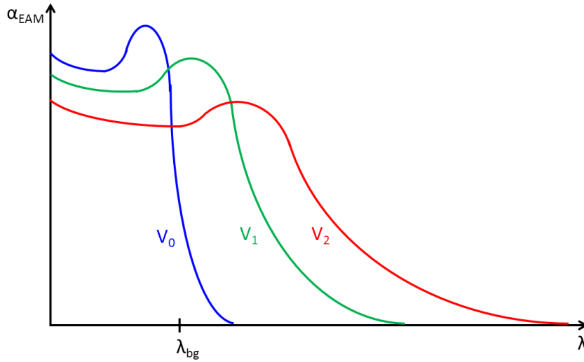
Fig. 2.2.4: Absorption spectrum for an MQW EAM with no applied reverse bias (blue line) and nonzero applied reverse bias (green line and red line). Note that V_0=0V and |V_2|>|V_1| .
