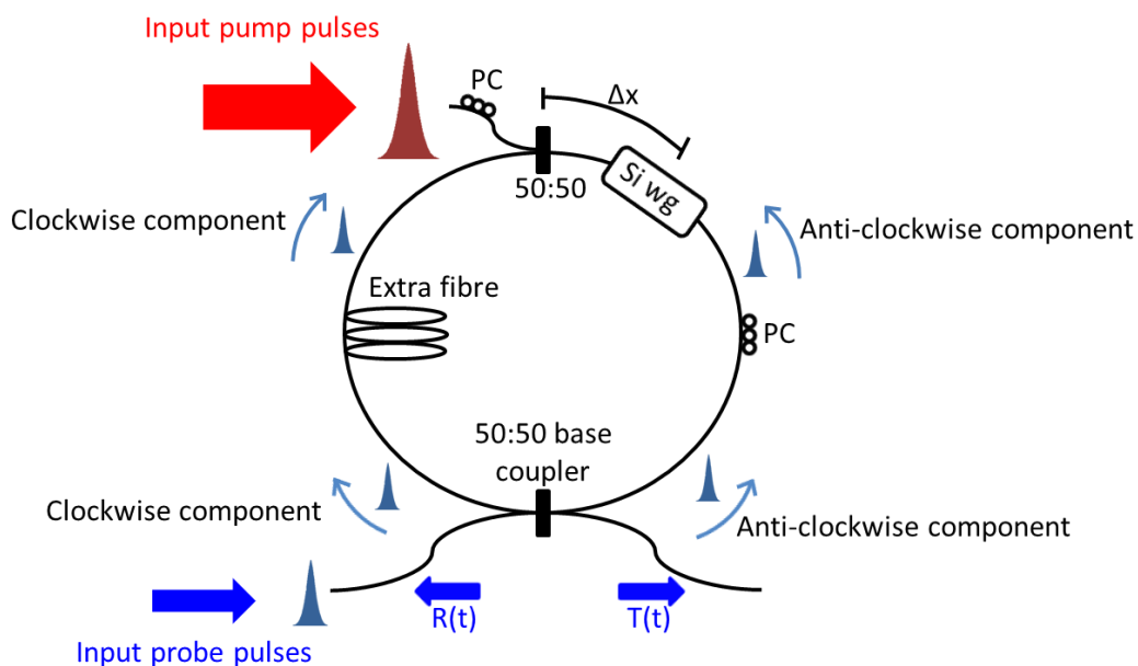
Fig. 5.2.3: Schematic diagram of TOAD loop test-bed.
