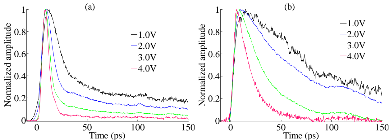
Fig. 6.3.2: Amplitude evolution for (a) EAM A0220 and (b) EAM 05045 normalized relative to the maximum change in transmission at each given reverse bias.
