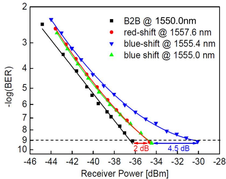
Fig. 5.5.4: BER vs received power for B2B, red-shifted and blue-shifted signals at 80\text{Gb.s}^{-1} .
