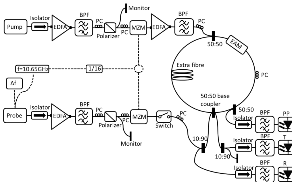
Fig. 6.2.5: TOAD loop system for measuring carrier dynamics in the EAM under test.
