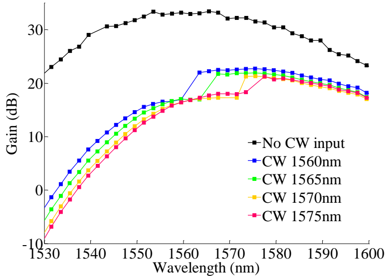
Fig. 3.5.1: Power gain spectra for SOA 03429 with a moderate power (-3.5dBm) CW input beam and with no CW input beam at wavelengths close to the small signal gain peak (1565nm).
