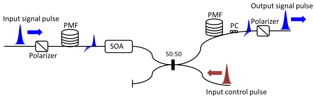
Fig. 2.1.18: Illustration of the operation of the UNI switch configuration.
