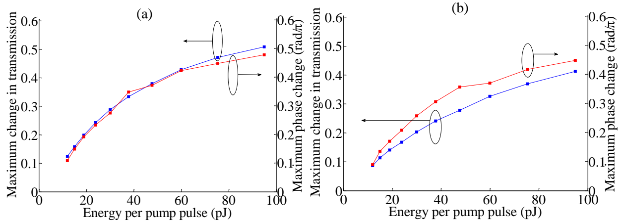
Fig. 5.3.7: Maximum phase change and maximum change in transmission as a function of energy per pump pulse for (a) 3.6mm long Si nanowire and (b) 4.9mm long Si nanowire.
