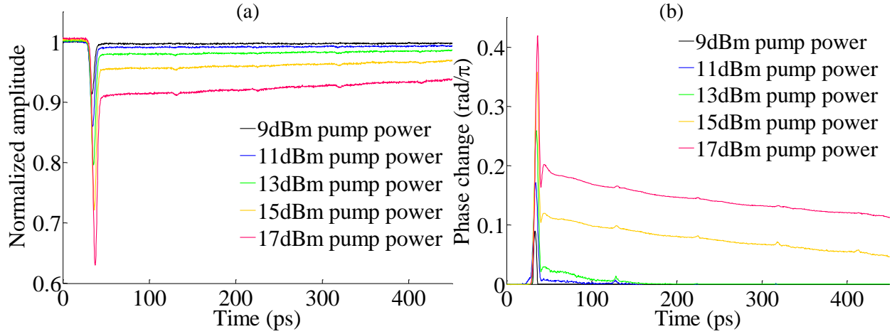
Fig. 5.3.3: (a) Amplitude and (b) phase dynamics of 4.9mm long Si nanowire, with probe input power of -27dBm and pump input power varied from 9dBm to 17dBm at the input to the chip.
