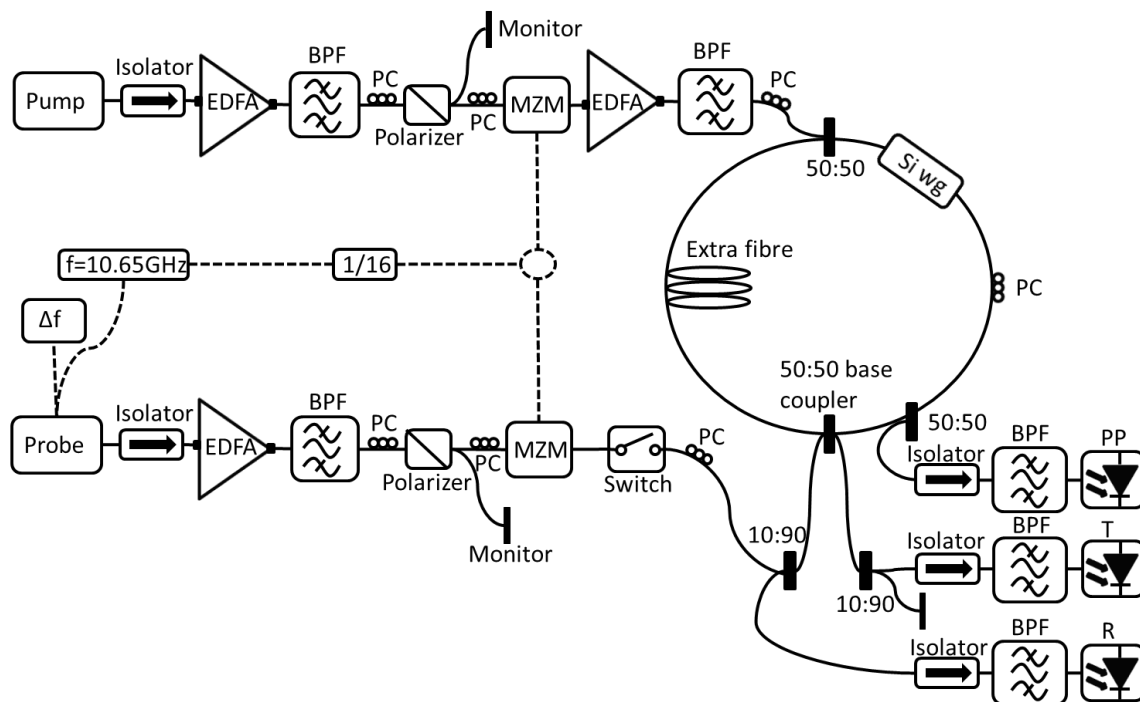
Fig. 5.2.2: TOAD loop system for measuring amplitude and phase dynamics of a Si nanowire placed inside the interferometric loop (Si wg = silicon waveguide/nanowire).
