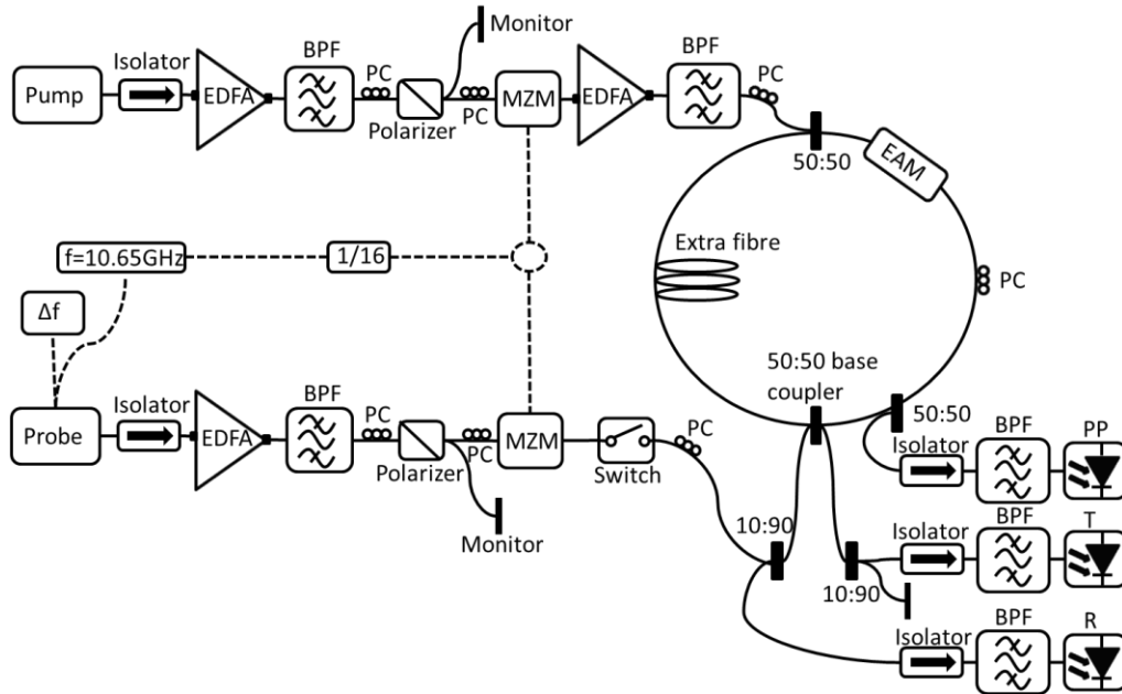
Fig. 6.2.5: TOAD loop system for measuring carrier dynamics in the EAM under test.
