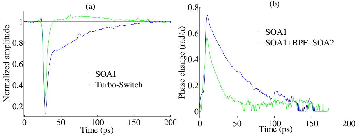
Fig. 4.3.20: (a) Amplitude and (b) phase evolution of SOA1 at a current bias of 400mA and the entire Turbo-Switch configuration at a current bias of 400mA for both SOAs.
