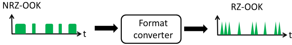
Fig. 2.7.3: Diagram illustrating the principle of NRZ-OOK to RZ-OOK format conversion.
