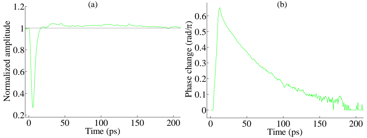
Fig. 4.3.11: (a) Normalized amplitude and (b) phase evolution for CSES configuration with current bias of 300mA (SOA1), 200mA (SOA2) and EAM reverse bias of 2.2V.
