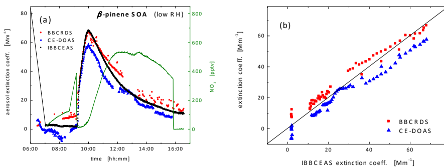
Fig. 3. (a) Time profile of the aerosol extinction coefficient following \text{NO}_3 oxidation of \beta -pinene under dry conditions (20 June). Changes to the chamber composition occurred at: 06:27–06:37 (80 ppbv \text{NO}_2 ), 06:50 LT (15 ppbv \text{O}_3 ), 08:40 LT (80 ppbv \text{O}_3 ), and 9:09 (15 ppbv \beta -pinene). (b) Correlation plots of the aerosol extinction coefficients retrieved by the BBCRDS and CE-DOAS instruments against those from the IBBCEAS measurements. The 1 : 1 line is shown as a solid line.
