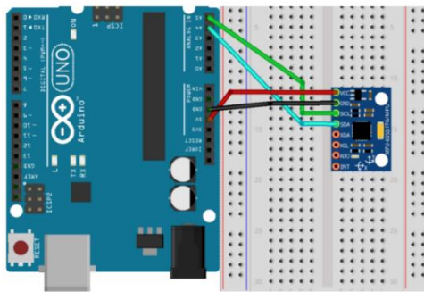
Figure 4. 26 Connection Inertial measurement sensor to Arduino Uno WiFi (20)
