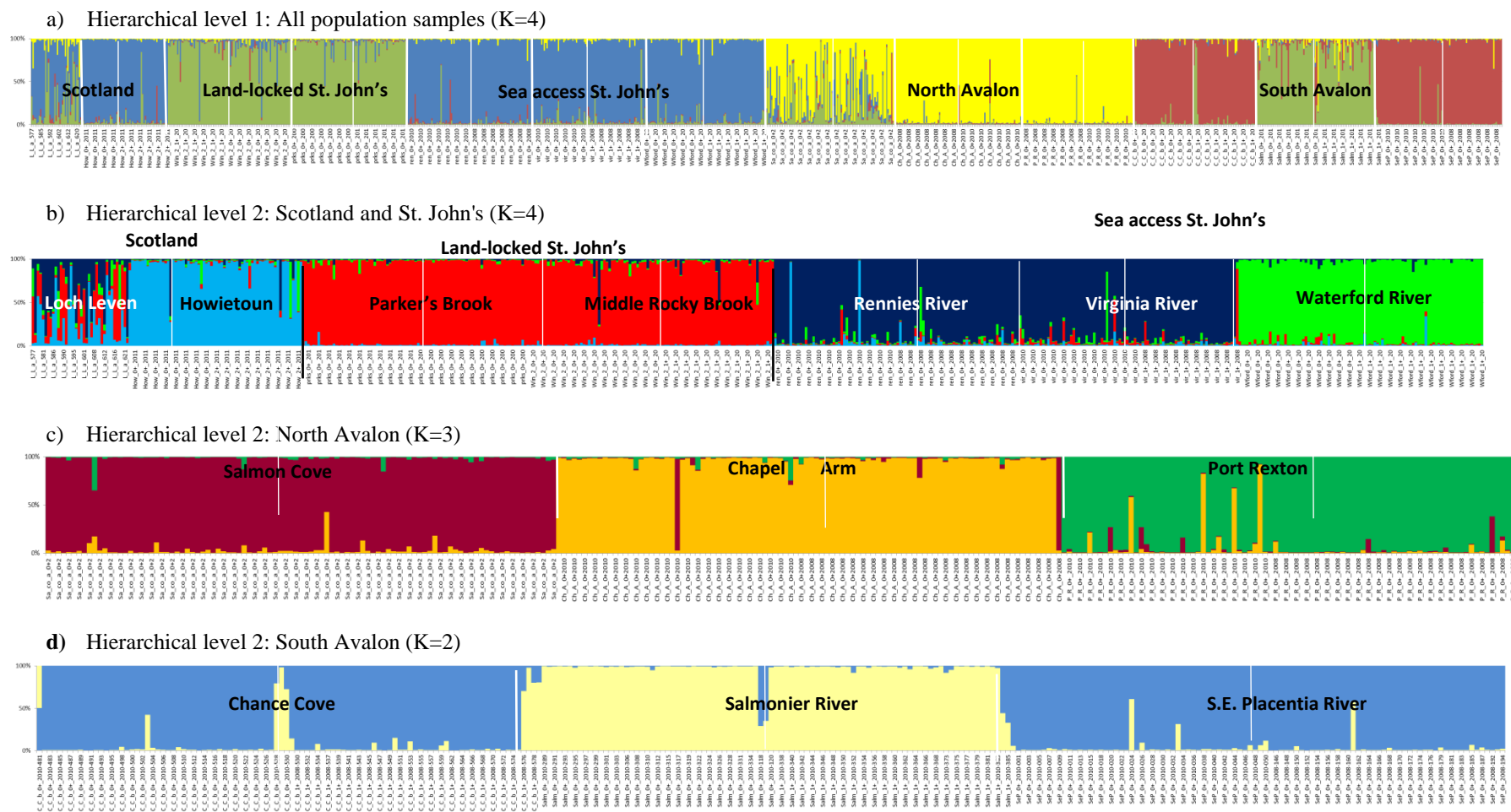
Figure 5: Bar plots of STRUCTURE simulations at two hierarchical levels. Each bar represents an individual fish. Y-axis = proportion of each fish attributed to each cluster, estimated from the colour of the bars. Colours in a) relate to the same groups as shown in Figures 3 and 4, but colours in b), c) and d) are independent.
