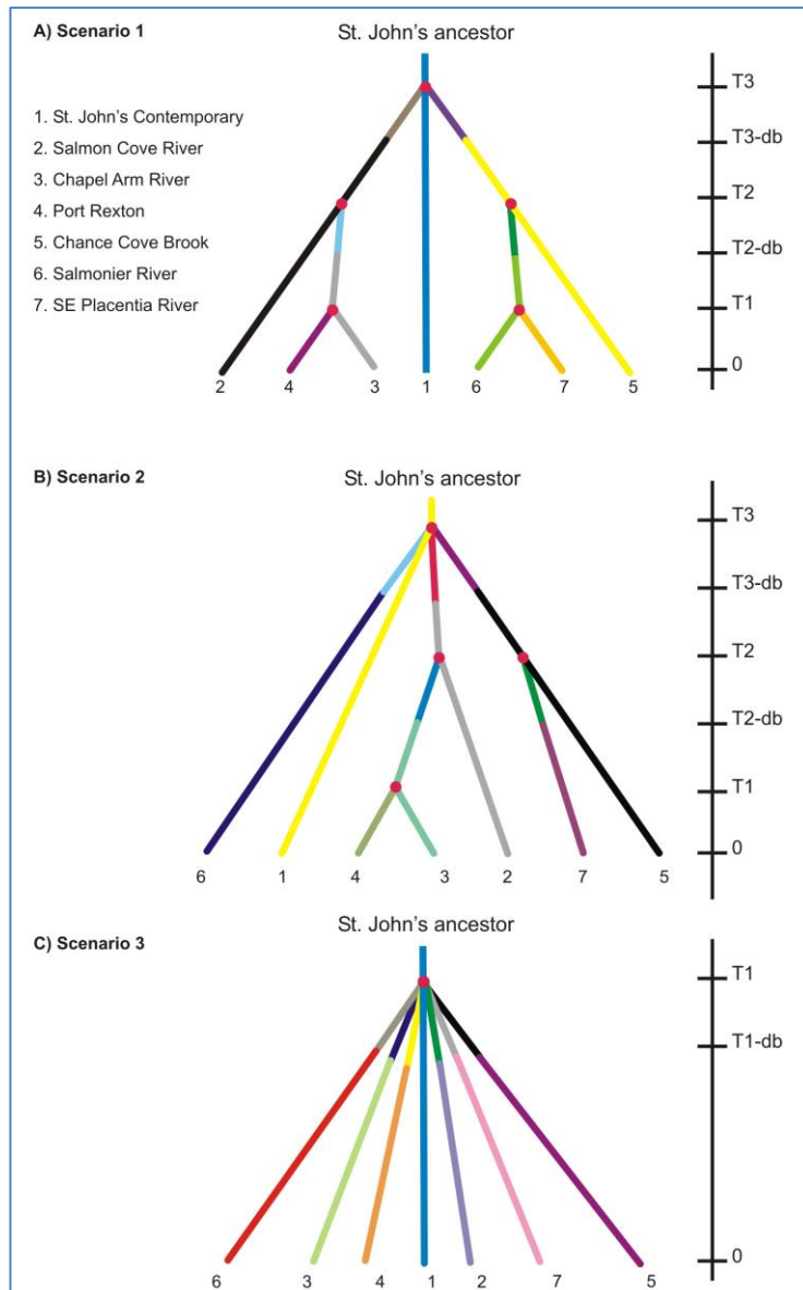
Figure 6. Alternative scenarios (see text for details) related to the origin(s) and/or possible colonisation patterns of S. trutta in Newfoundland outside St. John's using the ABC approach, implemented in DIYABC (Cornuet et al. 2010). Times of lineage origins are indicated back in time by T1 , T2 and T3 , while 0 indicates present/contemporary time. Here, time is measured in terms of number of generations ('time' in the figure represents evolutionary time). It is important to note that when a new population is formed from individuals migrating from an ancestral population, there is an initial size reduction (noted in the graph by "-db" and distinct colours). This is because new populations generally start with a few immigrants (i.e. founder effect).
