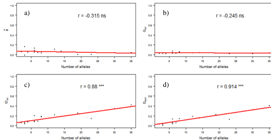
Figure 5: Correlation assessment of locus estimators a) F_{ST} (Weir and Cockerham, 1984), b) G_{ST} (Nei and Chester, 1983), c) G'_{ST} (Hedrick, 2005) and d) D_{est} ( D_{Jost} unbiased estimator, Jost, 2008), with locus polymorphism (total number of alleles), returned from the corPlot function in the DiveRsity software programme (Keenan et al. , 2013). Red lines represent the line of best fit and r values are Pearson product moment correlation coefficients. Both G'_{ST} and D_{est} provide a suitable fit to the data.
