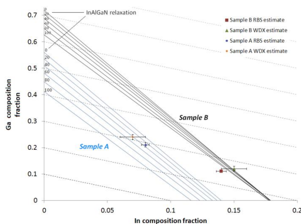
Figure 3: [0002] \omega -2 \theta XRD fitting parameters that give compatible results for sample A (solid blue lines) and sample B (solid black lines), with different InAl(Ga)N relaxation values considered. Constant Al content contour lines are also shown (dashed lines)
