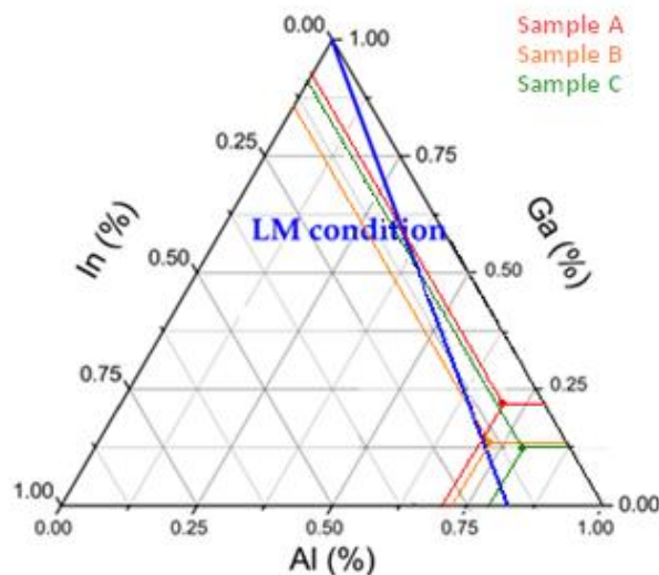
Figure 4: Quaternary map of samples A, B and C, showing the compositions of InAlGaIn lattice matched to GaN
