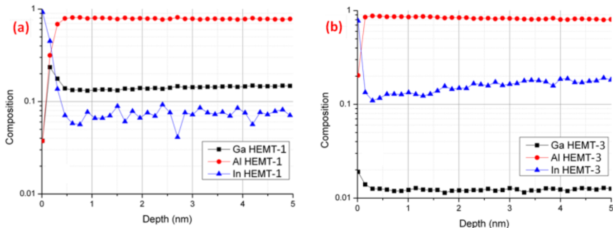
Figure 5: SIMS profiling of InAlN HEMT barrier layers without (a) and with (b) MOVPE reactor conditioning (HEMT-1 and HEMT-3 respectively).
