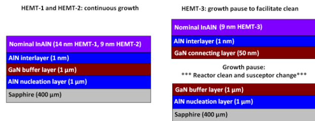
Figure 2: Schematic of the HEMT layers grown in this series. HEMT-1 and HEMT-2 were grown continuously while HEMT-3 included a growth pause so the reactor could be cleaned and susceptor changed.
