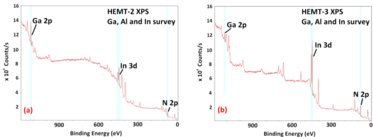
Figure 6: XPS profiling of InAlN HEMT barrier layers without (a) and with (b) MOVPE reactor conditioning (HEMT-2 and HEMT-3 respectively).
