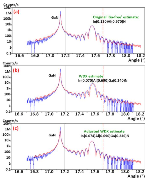
Figure 1: \omega -2 \theta [0002] XRD scans of sample A using a Ga-free InAlN layer (a), WDX composition values (b) and WDX values adjusted visually (c). This method is sensitive to changes in composition down to 0.1%.
