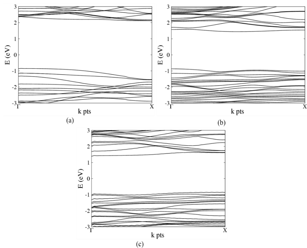
Figure 6: One-dimensional band structure for 10 Å diameter Germanium wires along [100] with different surface terminations (a) \text{-H} (b) \text{-NH}_2 and (c) \text{-OH} . Result from hybrid DFT (HSE06) calculation.
