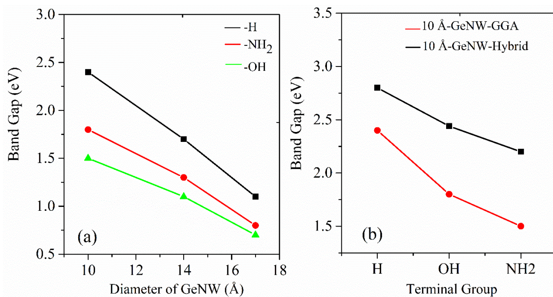
Figure 5: Computed band gap as a function of the diameter for (100) oriented Germanium nanowires for the surface terminations studied in this paper. (a) GGA-PBE results. (b) GGA-PBE and HSE06 results for 10 Å diameter nanowires.
