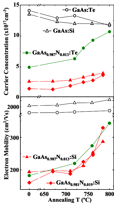
FIG. 2. (Color online) Free carrier concentration, n , and electron mobility, \mu , for GaAs(N):Si and GaAs(N):Te as a function of annealing- T . With increasing annealing- T , \mu increases for both films, while n increases substantially (minimally) for GaAsN:Te (GaAsN:Si) films.
