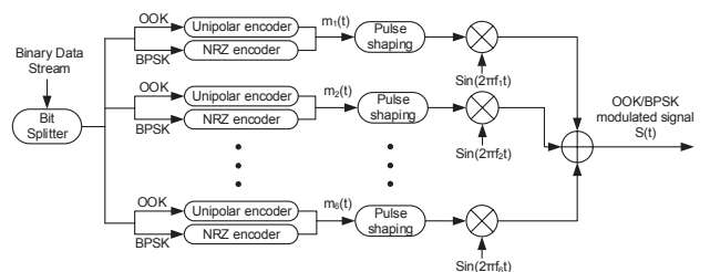
Fig. 5: Schematic diagram of the multi-channel on-off keying (OOK) and binary shift keying (BPSK) modulator.
