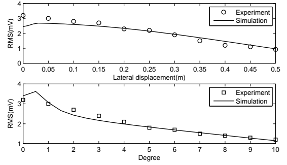
Fig. 14: Comparison of experimental signal RMS values with theoretical predictions with different: (a) lateral displacements and (b) oblique angles at a transducer separation of 5 m.
