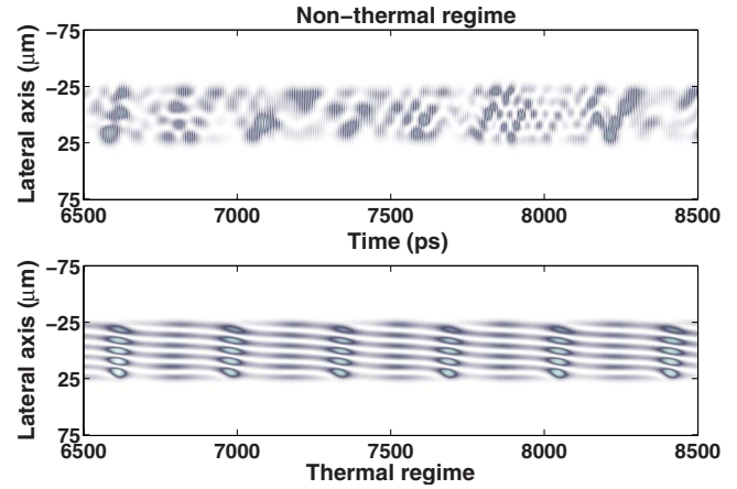
FIG. 20. (Color online) Time-resolved near field (6.5–8.5 ns after laser switch on) for positively detuned ( \Omega=0.1 ) inhomogeneously broadened gain medium ( \sigma_D=3 ) for both thermal and nonthermal regimes. Negative detuning gives qualitatively similar profiles.
