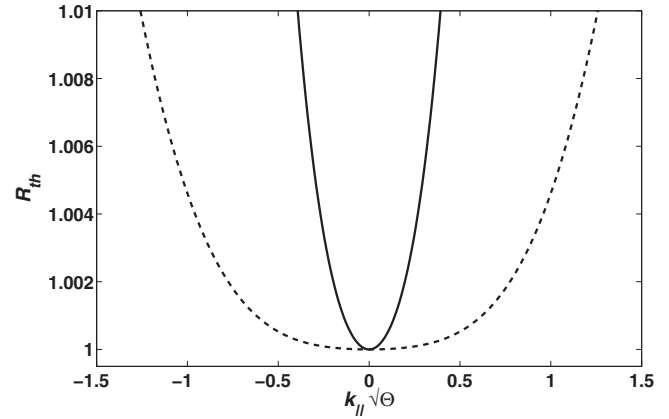
FIG. 3. Neutral stability curve for negative detuning ( \Omega=-0.1 ). Homogeneous ( \sigma_D=0 , solid line) and inhomogeneous broadening ( \sigma_D=3 , dashed line).
