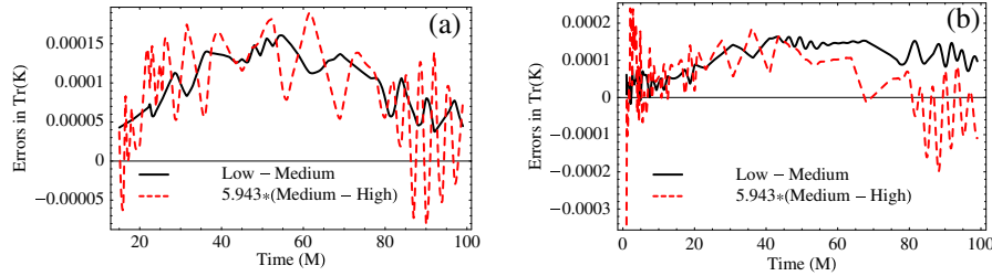
FIG. 13 (color online). Convergence of K at the horizon, for simulations with initial lapse (a) \alpha = \psi^{-2} , and (b) \alpha = 1 . The \alpha = \psi^{-2} simulations are not convergent at early times, while the \alpha = 1 simulations lose clean convergence after about 50M .
