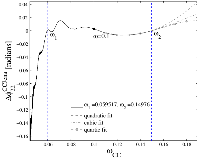
FIG. 2 (color online). Comparison between Caltech-Cornell and Jena actual numerical data: the phase difference \Delta\phi_{22}^{\text{CCJena}} = \phi_{22}^{\text{CC}} - \phi_{90M}^{\text{Jena}} is shown versus Caltech-Cornell GW frequency \omega_{\text{CC}} .
