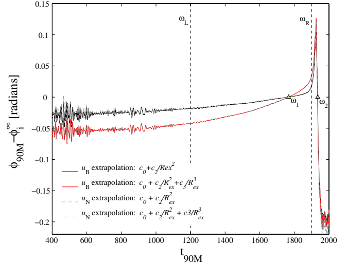
FIG. 1 (color online). Differences between the phase extracted at R_{\text{ex}} = 90M , and the phase extrapolated to infinity based on two choices of the retarded time and on two choices of the extrapolating polynomial, as described in the text. The choice of retarded time makes little difference to the result.
