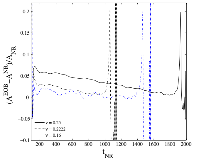
FIG. 9 (color online). Fractional EOB-NR differences in the gravitational wave (metric) amplitudes, A \equiv |\Psi_{22}| , versus NR time for different mass ratios.
