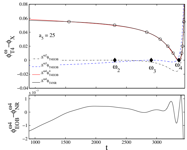
FIG. 4 (color online). Top panel: near-perfect agreement between T4-EOB and T4-NR phase differences when a_5 = 25 , \bar{a}_{\text{RR}} = 27.9197 , and v_{\text{pole}} = 0.51563 . Here NR refers to the published results of the Caltech-Cornell inspiral simulation. The corresponding EOB-NR phase difference (bottom panel) is of the order of 10^{-3} radians over the 30 GW cycles of the Caltech-Cornell inspiral simulation.
