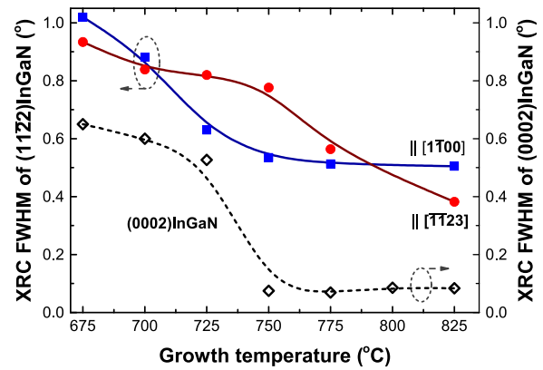
FIG. 3. The on-axis XRC FWHM values of the (0001) InGaN layers ( \diamond ), and the (11\bar{2}2) InGaN layers scanned along [1\bar{1}00] ( \blacksquare ) and [\bar{1}\bar{1}23] ( \bullet ) grown at different temperatures.
