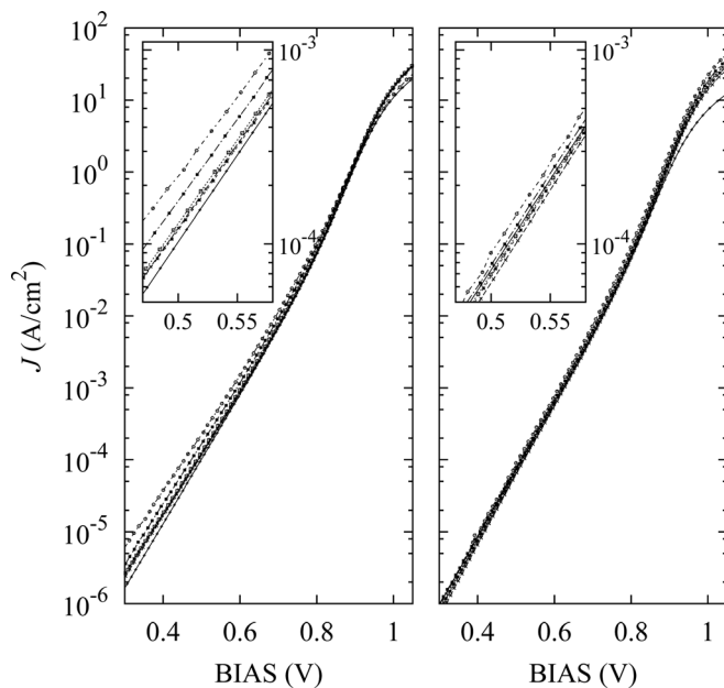
FIG. 1. Current density J of different size diodes as a function of voltage for samples A (left) and C (right). Solid lines at the bottom are for the largest size diodes (500 \mu m diameter) and the size decreases regularly upwards (200 \mu m, 150 \mu m, 100 \mu m, 50 \mu m, 20 \mu m). Insets show around 0.5 V in detail.
