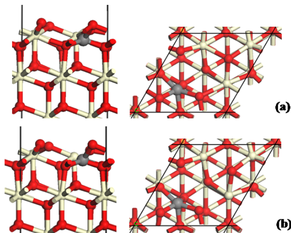
Fig.2 The relaxed CeO 2 (111) surface in a (2x2) surface supercell doped with Pd. (a) DFT-PW91+U, (b) HSE06. The black lines show the edge of the supercell. Pd is the dark coloured, large sphere
