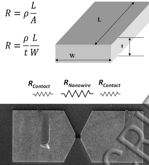
Figure 3 : A schematic of a conductive track of length L , width W , thickness t , along with the resistance components in the 2 contact pad test structure investigated in this work.
