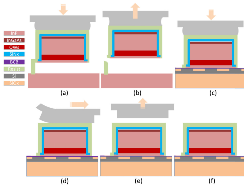
Fig. 5. Transfer printing of the III-V coupons: (a) Laminating the PDMS stamp to the released coupon on the source substrate, (b) Picking up the III-V coupon by rapidly lifting up the stamp, (c) Laminating the III-V coupon against photonic target substrate with a slight overdrive, (d) Applying a shear force to detach the III-V coupon from the stamp, (e) Lifting up the stamp, (f) The transfer printed III-V coupon on the target photonic circuit.
