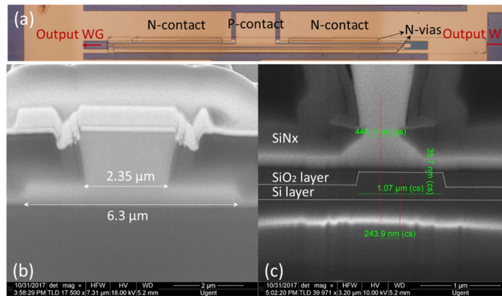
Fig. 8. (a) Top-view microscope image of a transfer-printed DFB laser, (b) FIB cross section image in the middle of the DFB laser, (c) FIB cross section image near the III-V/Si taper tip, showing a misalignment of less than 250 nm.
