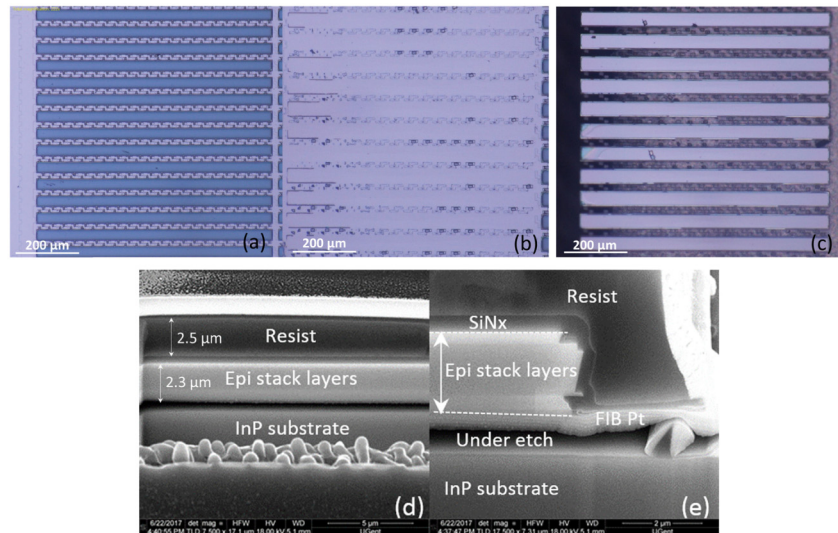
Fig. 4. The released coupon arrays patterned on the native InP substrate, (a) Dense coupon array, (b) Surface of the InP substrate after picking an array of coupons, (c) Bottom surface of the coupons, (d) Focused ion beam (FIB) cross section image of a released coupon, (e) Zoom-in image of the cross section.
