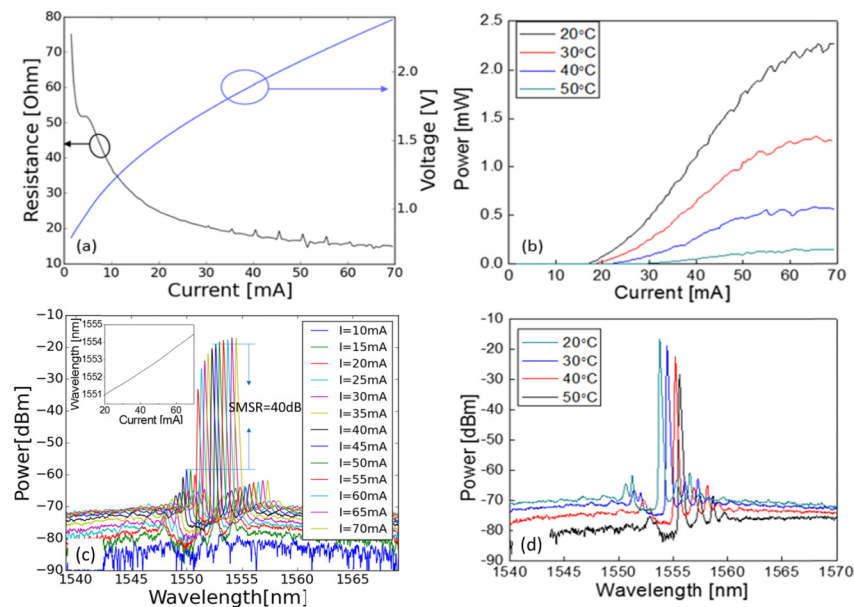
Fig. 9. Performance of the fabricated DFB laser. (a) V-I curve and differential resistance, (b) P-I curve at different temperatures, (c) Superposition of the output spectra at different bias currents, the inset shows the laser wavelength evolution as a function of current (d) Wavelength shift as a function of the stage temperature.
