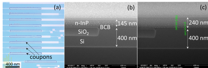
Fig. 6. (a) Array of printed III-V coupons on a silicon photonic target substrate (before photoresist encapsulation removal). (b) Cross section image at end of the coupon; (c) Cross section image in the middle of the coupon.
