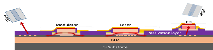
Fig. 2. Schematic of an integrated photonic circuit built on a passive SOI waveguide circuit based on transfer printing combining different III-V epitaxial layer stacks densely integrated together.
