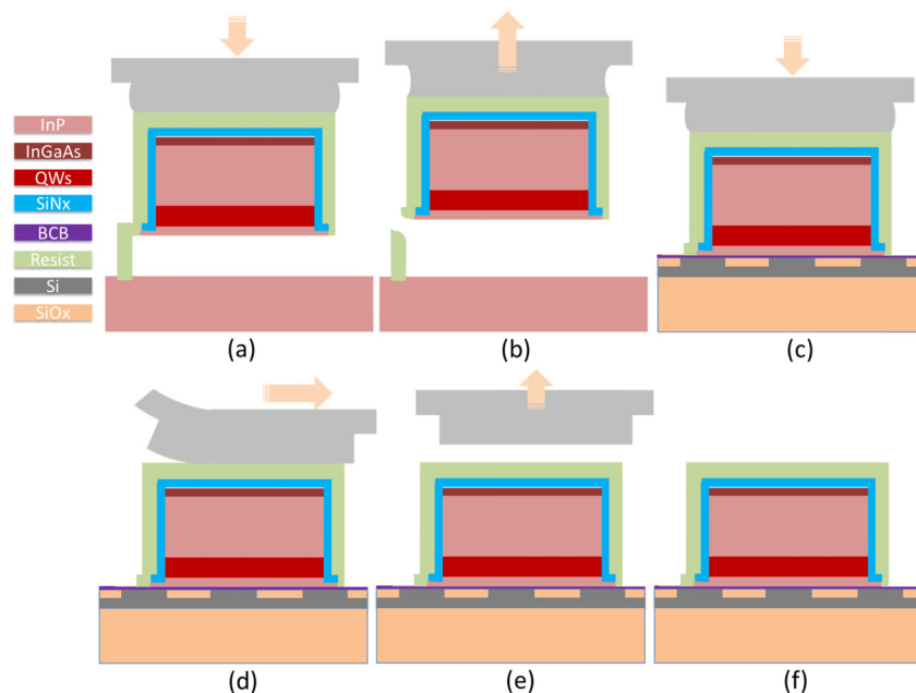
Fig. 5. Transfer printing of the III-V coupons: (a) Laminating the PDMS stamp to the released coupon on the source substrate, (b) Picking up the III-V coupon by rapidly lifting up the stamp, (c) Laminating the III-V coupon against photonic target substrate with a slight overdrive, (d) Applying a shear force to detach the III-V coupon from the stamp, (e) Lifting up the stamp, (f) The transfer printed III-V coupon on the target photonic circuit.
