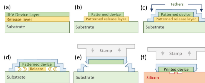
Fig. 1. Micro-transfer-printing concept, illustrating the release, picking and printing of a single coupon/device. The concept can readily be extended to massively parallel printing, by using a properly structured stamp.
