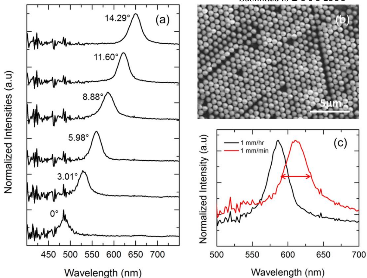
Figure 3. (a) Angle resolved scattering from the 2D PhC formed from 2.5 wt% PMMA spheres with 4 mg ml -1 SDS dip coated at a slow rate (~1 mm/hr). Light was incident at 45°. (b) SEM image of the top surface of the 2D PhC. (c) Scattering at an angle of 8.88° for light incident at 45° for samples formed at fast rate with 5 wt% spheres and 8 mg ml -1 SDS (red), and for a sample formed at the slow rate where the concentrations of spheres and SDS are halved (black).
