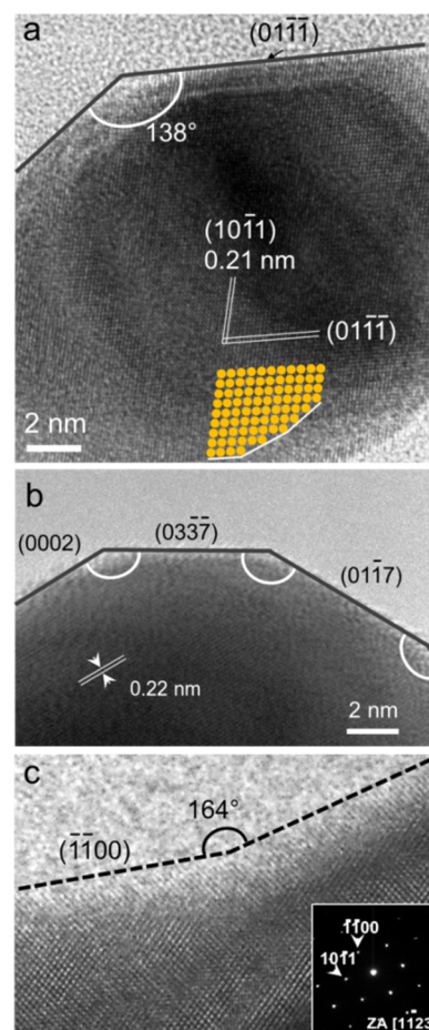
Fig. 3 HRTEM images of (a) a single Re NP and (b,c) the edges of high-index NP facets of similar single crystal Re NPs. (Inset) electron diffraction pattern of hexagonal Re, space group P63/mmc and cell parameters a = 0.276 nm and c = 0.445 nm.
