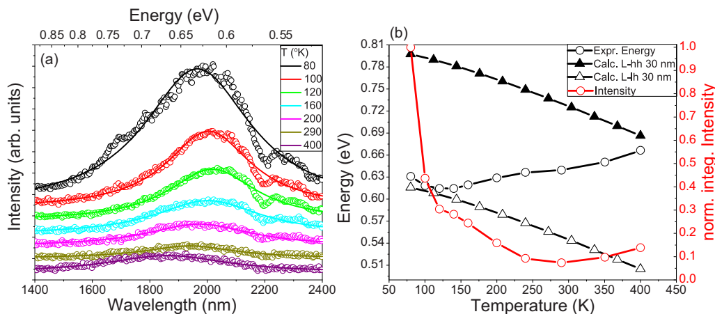
FIG. 3. (a) Photoluminescence spectra of Ge/In 0.24 Ga 0.76 As (sample E) under \epsilon = 1.6\% biaxial tensile strain depending on temperature; (b) experimental (circles) and calculated (triangles) peak energy (black line) and normalized integrated intensity (red line) versus temperature.
