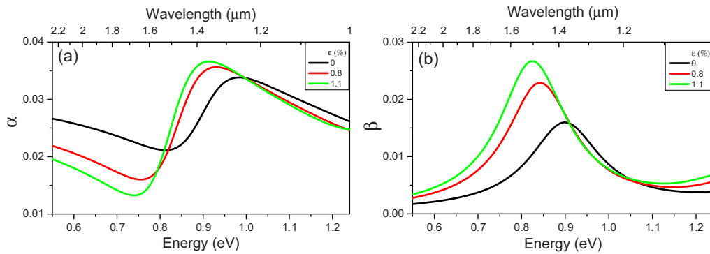
FIG. 12. Calculated (a) \alpha and (b) \beta Seraphin-Bottka coefficients in Ge at 80 K and at 0%, 0.8%, and 1.1% biaxial tensile strain.
