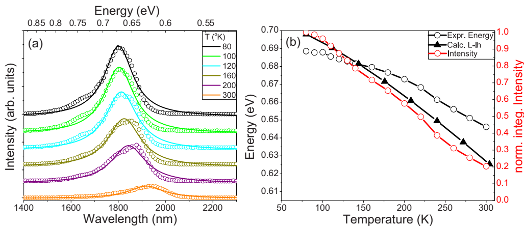
FIG. 2. (a) Photoluminescence spectra of GaAs/Ge/In 0.16 Ga 0.84 As/GaAs (sample C) under \epsilon = 0.95\% biaxial tensile strain depending on temperature; (b) experimental (circles) and calculated (triangles) peak energy (black line) and normalized integrated intensity (red line) versus temperature.
