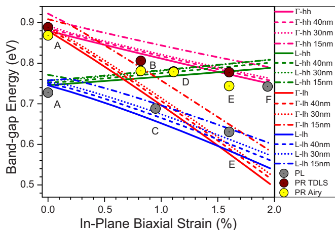
FIG. 8. Theoretical band-gap-strain dependence for Ge calculated using a 30 \times 30 \mathbf{k} \cdot \mathbf{p} model taking into account quantization-induced band-gap enhancement at decreased \epsilon -Ge layer thicknesses for 40-, 30-, and 15-nm quantum wells. Experimental peaks given by PL and PR data are shown as circles over theoretically predicted transitions from \Gamma and L valley to light (lh) and heavy (hh) holes.
