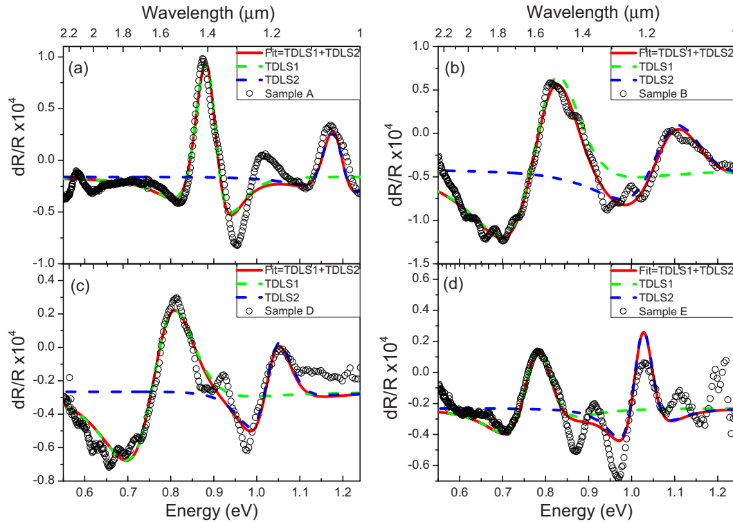
FIG. 6. Photorefectance spectrum of Ge under \varepsilon : (a) sample A, 0%; (b) sample B, 0.82%; (c) sample D, 1.11%; (d) sample E, 1.6% biaxial tensile strain at 80 K, fitted with two TDLS functions. Open circles correspond to the experimental data, red lines are the fit including two TDLSs, depicted in green and blue, respectively.
