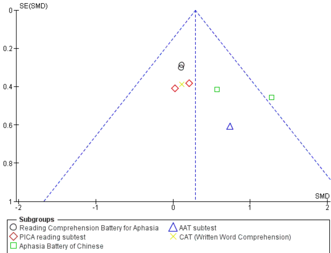
Figure 4. Funnel plot of comparison: I SLT versus no SLT, outcome: I.3 Receptive language: reading comprehension.
