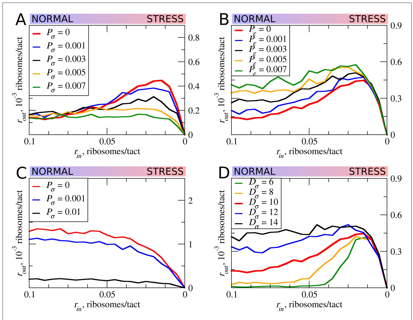
Figure 6. The effect of the size of scanning ribosomes ( D_\sigma ) and probability of spontaneous ribosome dissociation ( P_\sigma ) on stress resistance. Other parameters of the simulations; t_{\sigma>\varepsilon}=0.8 ; L=100 ; m_\sigma=0.3 ; m_\varepsilon=0.3 . (A, B) Absolute changes in the density of ribosomes downstream of a uORF under a scenario in which scanning (A) or elongating (B) ribosomes could dissociate spontaneously with probabilities P_\sigma and P_\varepsilon , respectively. (C) Same as (B) but scanning ribosomes do not dissociate upon collisions with elongating ribosomes. (D) The absolute changes in the densities of ribosomes downstream of a uORF depending on the size of the scanning ribosomes. Source data for panel (A) are provided in Figure 6—source data 1 , for panel (B) in Figure 6—source data 2 , for panel (C) in Figure 6—source data 3 and for panel (D) in Figure 6—source data 4 .
