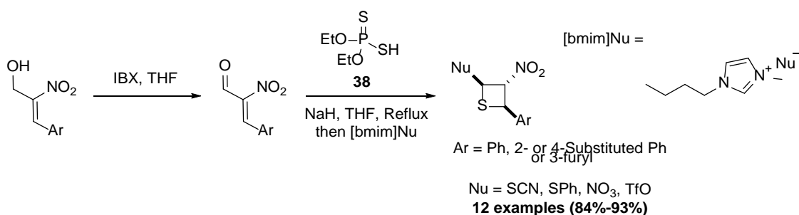
Scheme 20
