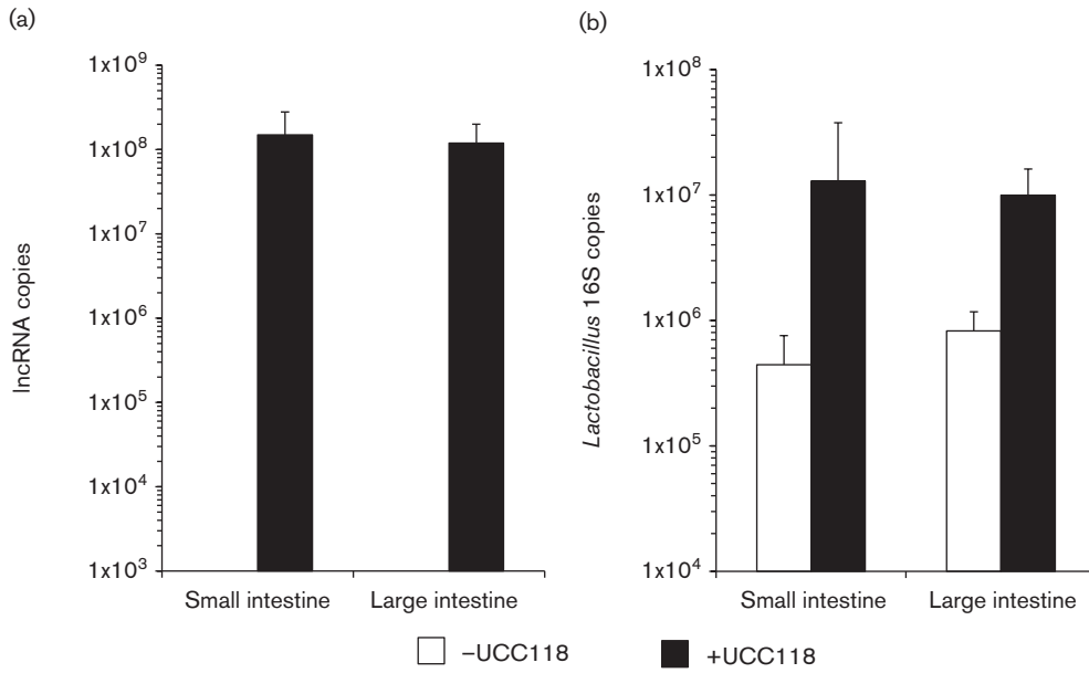
Fig. 4. Expression of L. salivarius UCC118 IncRNA in vivo. (a) The presence of the IncRNA was quantified by RT-qPCR in both small and large colonic contents in mice ( n=4 in each group) gavaged or not with L. salivarius UCC118. Data are means \pm SD. (b) The lactobacilli level was quantified by qPCR in both small and large colonic contents in mice ( n=4 in each group) after genomic DNA extraction. Data are means \pm SD.
