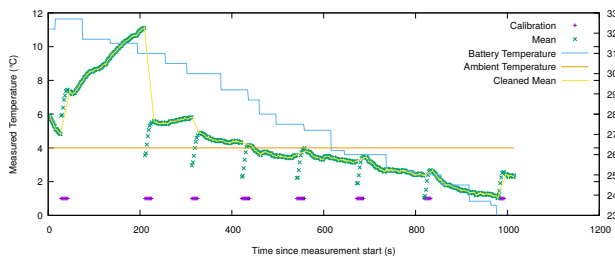
Fig. 4. Thermal calibration while measuring cold water in a smart refrigerator. The temperature measurement is affected by the temperature of the device, as evidenced by the internal battery temperature sensor.
