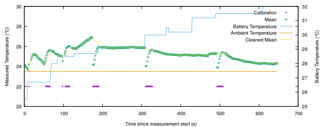
Fig. 5. Temperature measurements of a wall in an ambient temperature of 24°C. The temperature measurement is affected by the temperature of the device, resulting in higher than expected values.
