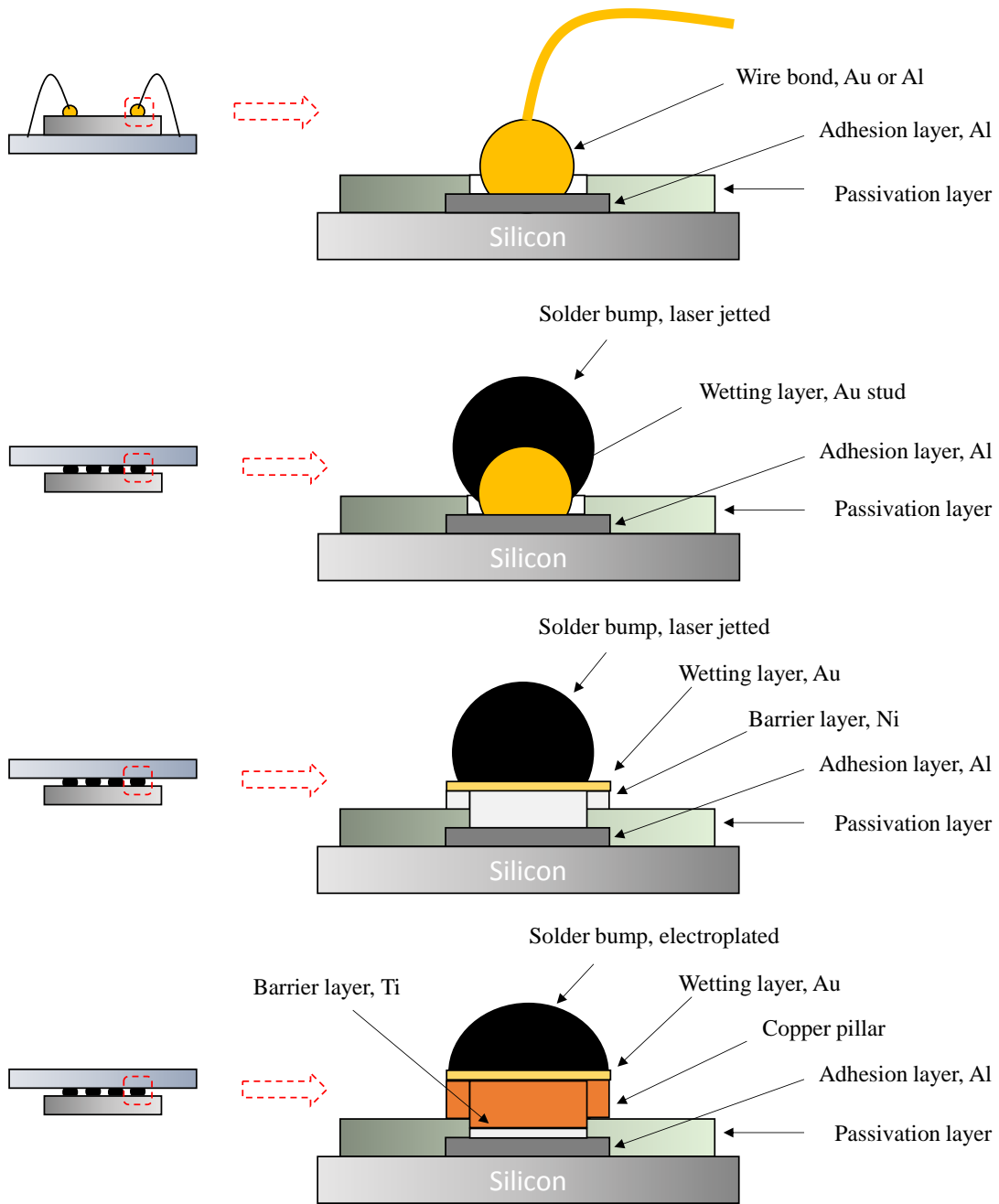
Fig. 6.6. Common electrical interconnects structure and metallization layers on device bond pad.
