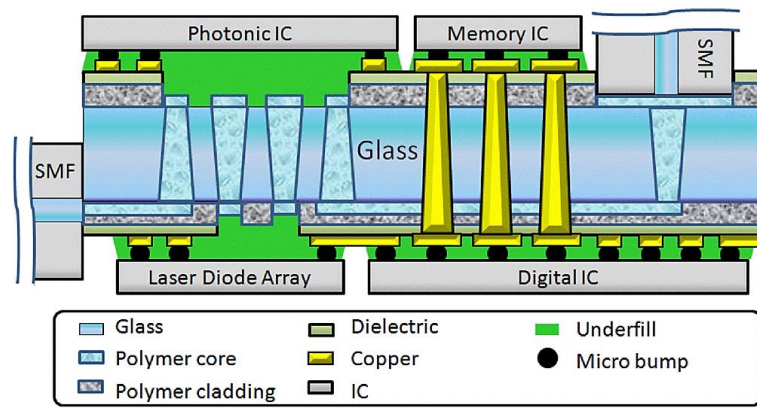
Fig. 1.15. Polymer plugged via to light coupling from [37].
