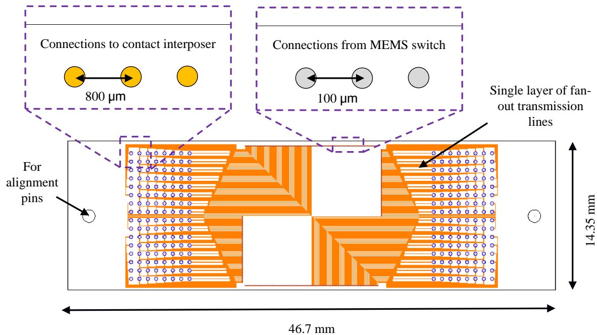
Fig. 3.7. Ceramic interposer design to redistribute 256 electrical bond pads from the MEMS device using single layer metallization with line width and space of 25 \mu\text{m} .
