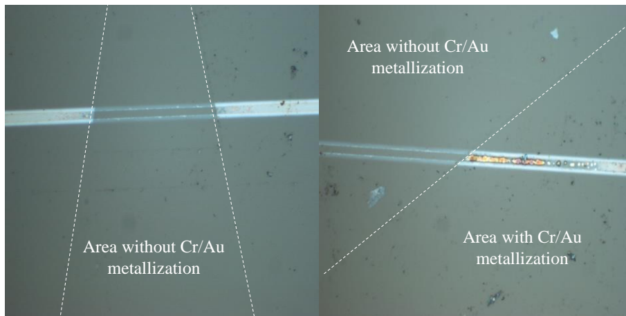
Fig. 5.15. Images of glass interposer post Cr/Au metallization wet etching, showing cloudy/opaque sections of ion-exchanged waveguide in areas covered by the metallization.
