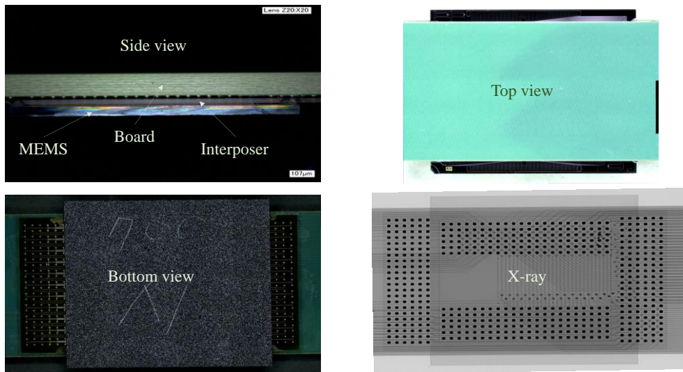
Fig. 3.23. Various optical views and X-ray images of the assembled through glass via MEM switch package.
