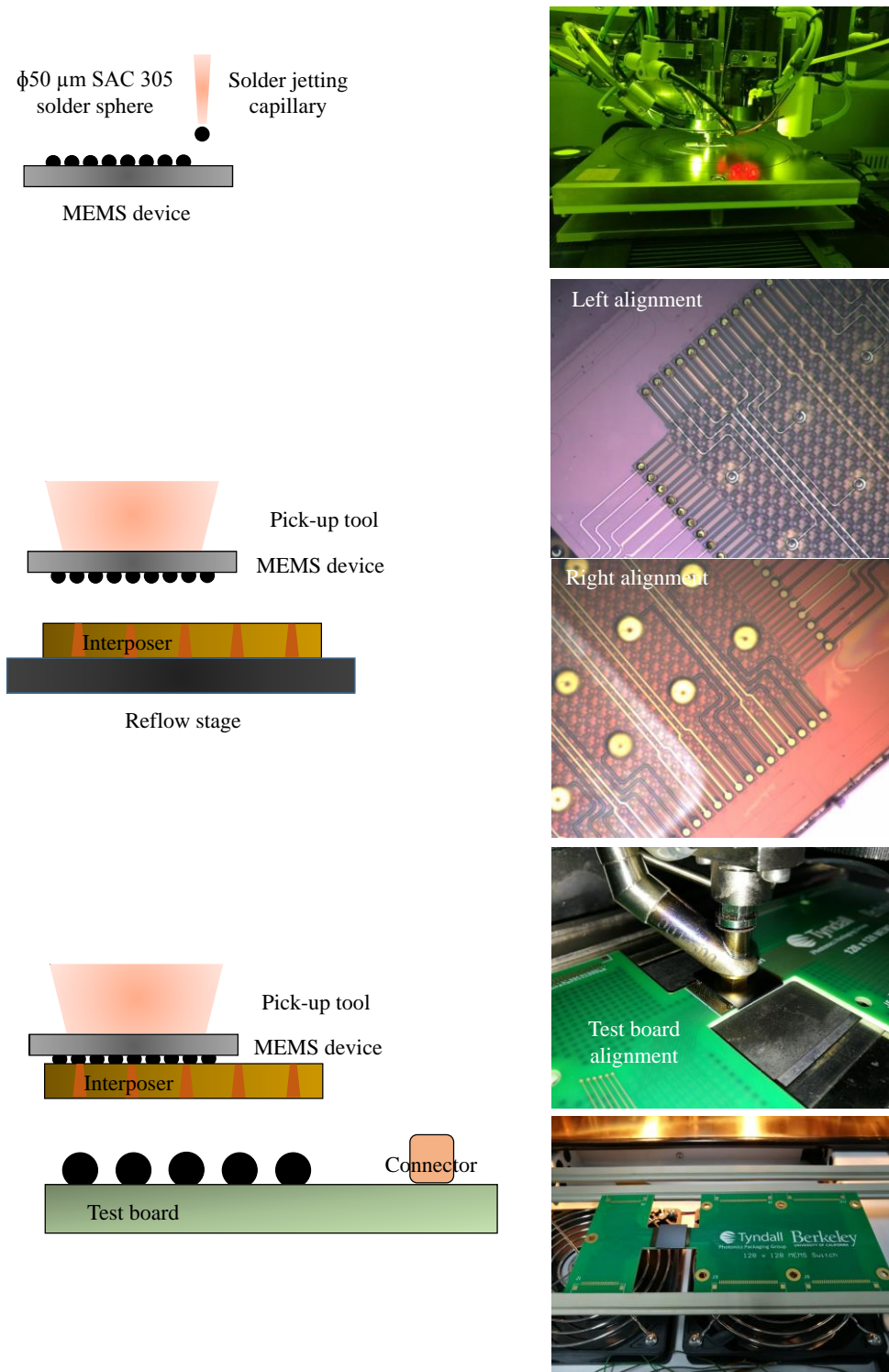
Fig. 3.22. Flip chip assembly processing of Test Vehicle 2b with two-step reflow processing, starting from solder jetting on device (top), followed by device-to-interposer assembly (middle) and finally interposer-to-board assembly (bottom).
