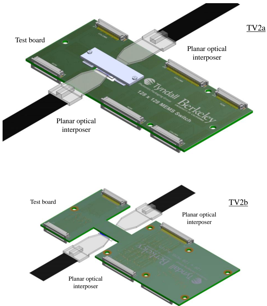
Fig. 3.16. 3-D illustration of the overall test vehicle assembly (optical and electrical) for Test Vehicle 2a – pluggable package (top) and 2b – through-glass-via package (bottom).
