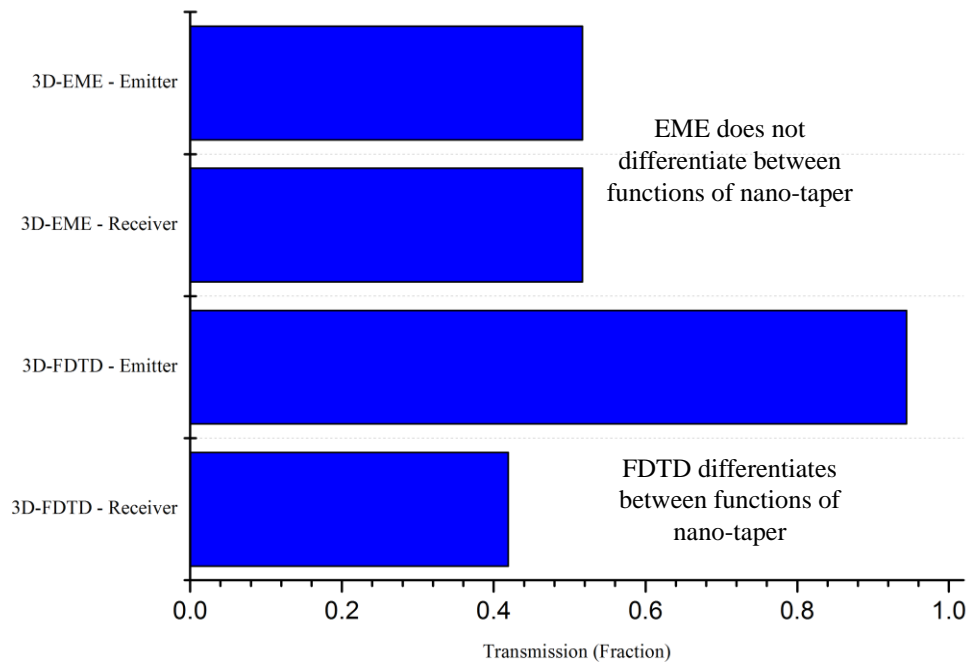
Fig. 5.26. Difference between MODE-EME and 3D-FDTD, using silicon nano-taper design 1 as simulation structure.
