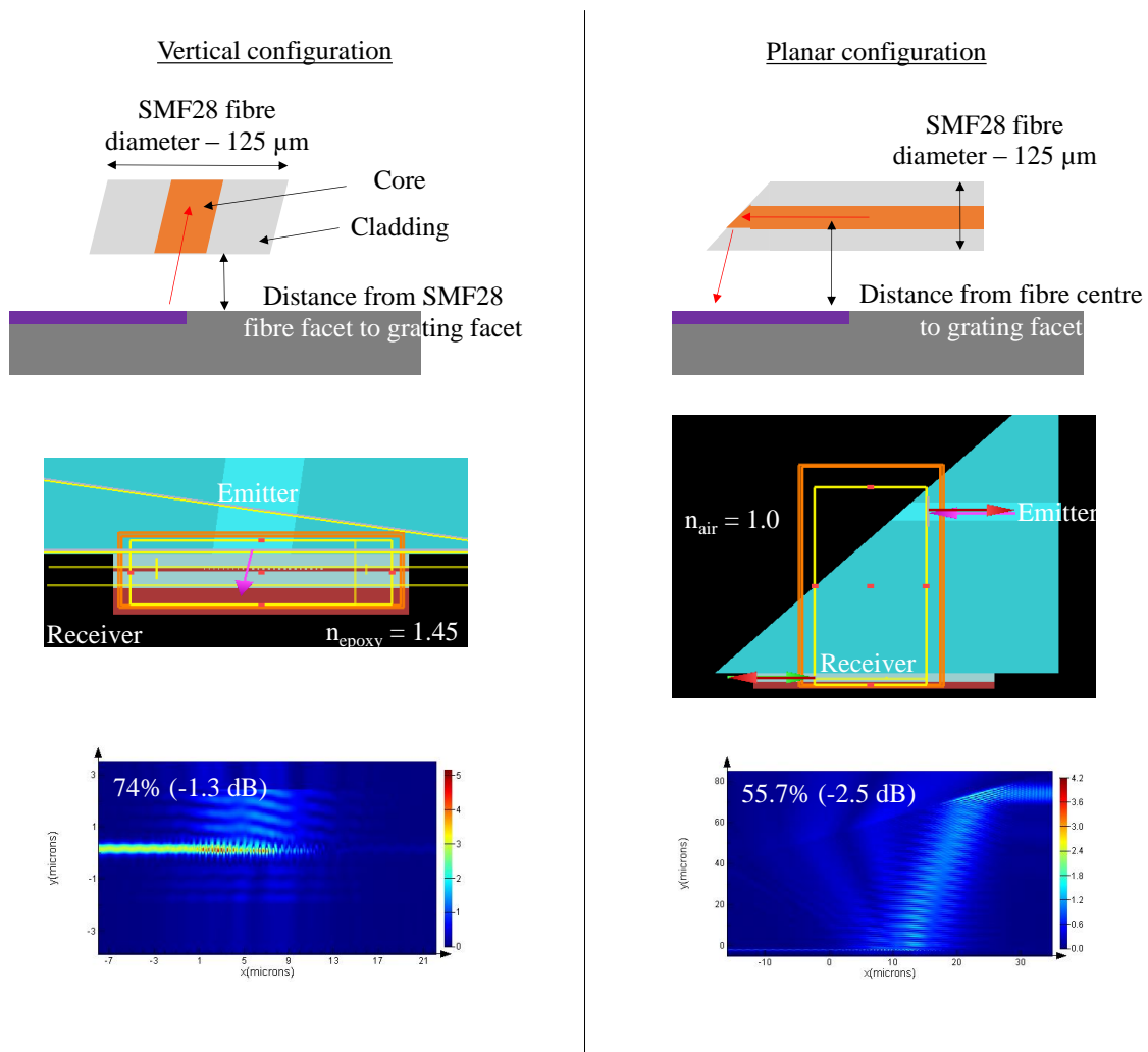
Fig. 1.6. 2D-FDTD simulation of vertical fibre coupling (left) and planar fibre coupling on non-uniform gratings (right).
