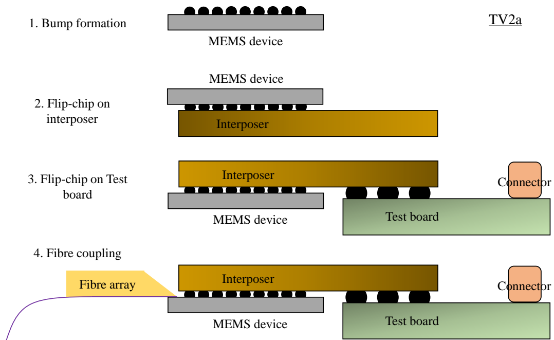
Fig. 3.5. Proposed Test Vehicle 2a (pluggable package) packaging and assembly process flow for the silicon photonic MEMS device. (a) Solder bump formation on MEMS device, (b) flip-chip MEMS device onto interposer, (c) flip-chip assembly onto test board, (d) optical assembly.
