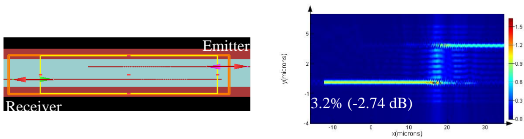
Fig. 4.4. 2D-FDTD simulation showing interaction between two vertically stacked non-uniform gratings at zero gap.
