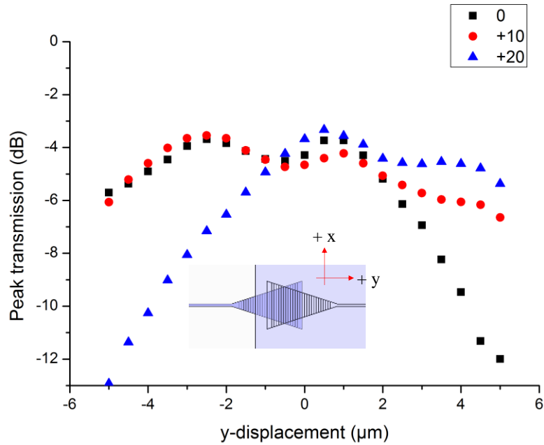
Fig. 4.14. Tolerance scan of coupling along the y-direction (along gratings) at various z-displacements.
