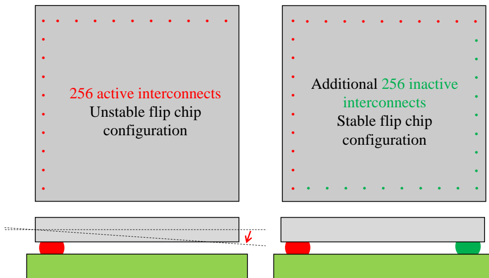
Fig. 3.2. Additional 256 flip chip joints were added for assembly stability. Similar to a chair with only 2 legs, without the additional rows of flip chip joints (in green), the die will be unstable and collapsed from slight handling movements.
