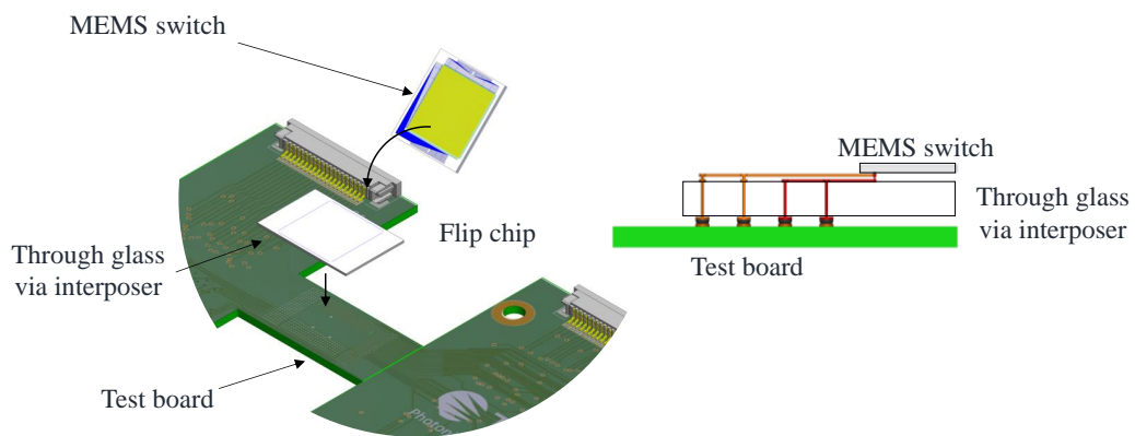
Fig. 3.13. Illustration of the 2.5D silicon photonic MEMS switch assembly with through glass interposer.
