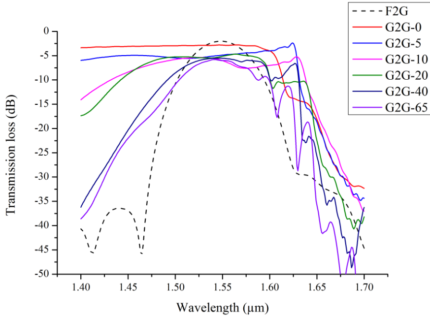
Fig. 4.16. Evolution of transmission losses and bandwidth as gap between the pair of vertically stacked gratings based on 220 nm SOI is increased.
