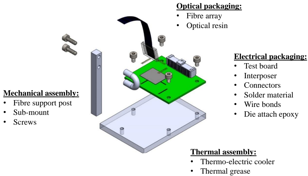
Fig. 1.1. Generic assembly of a silicon photonic package, consisting of thermal and mechanical considerations, in addition to optical and electrical packaging.
