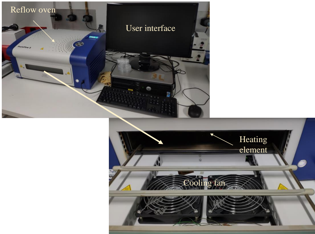
Fig. A5. Inert ( N_2 ) reflow oven by LPKF (Protoflow-S) used for board level reflow. Reflow temperature can reach 320\text{ }^\circ\text{C} thus suitable for AuSn assembly. Can be used as curing oven for underfill and die attach as well.
