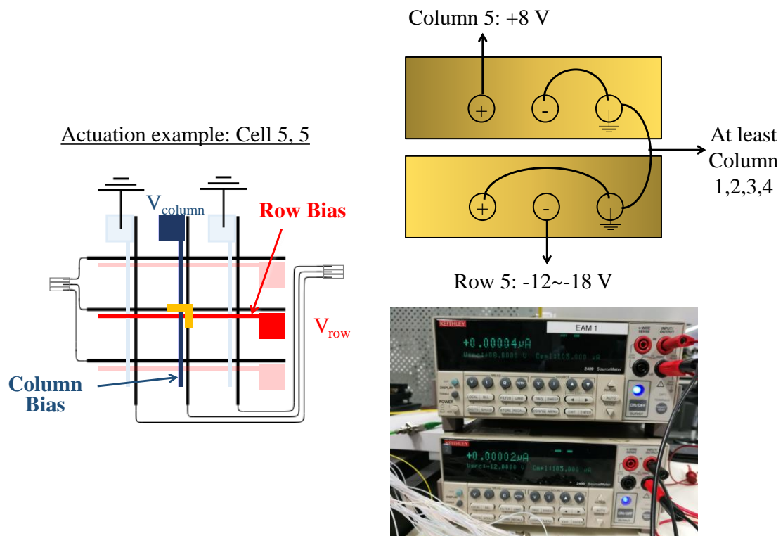
Fig. 3.30. MEMS switch actuation setup and configurations using Test Vehicle 2a.
