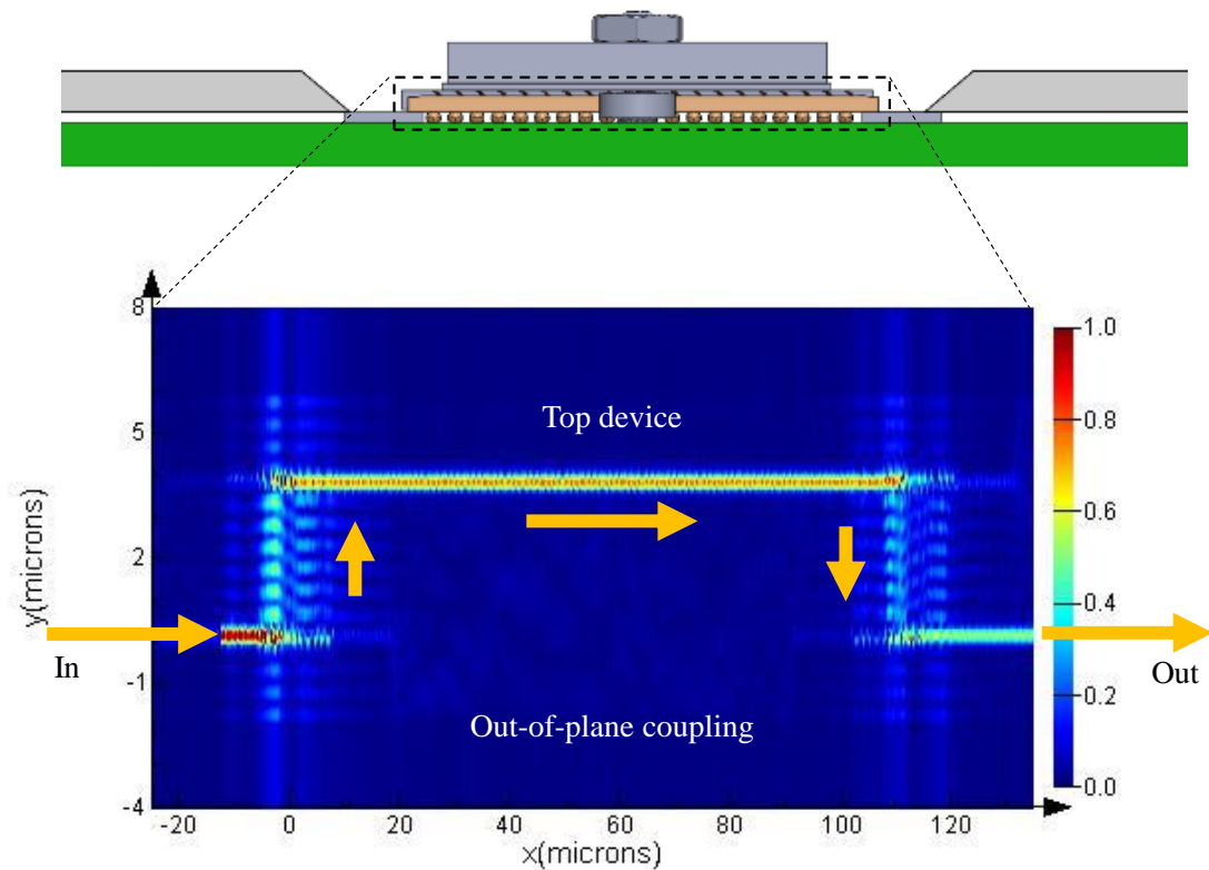
Fig. 4.2. A pair of vertically stacked gratings can interact, allowing broadband transmissions of optical power.
