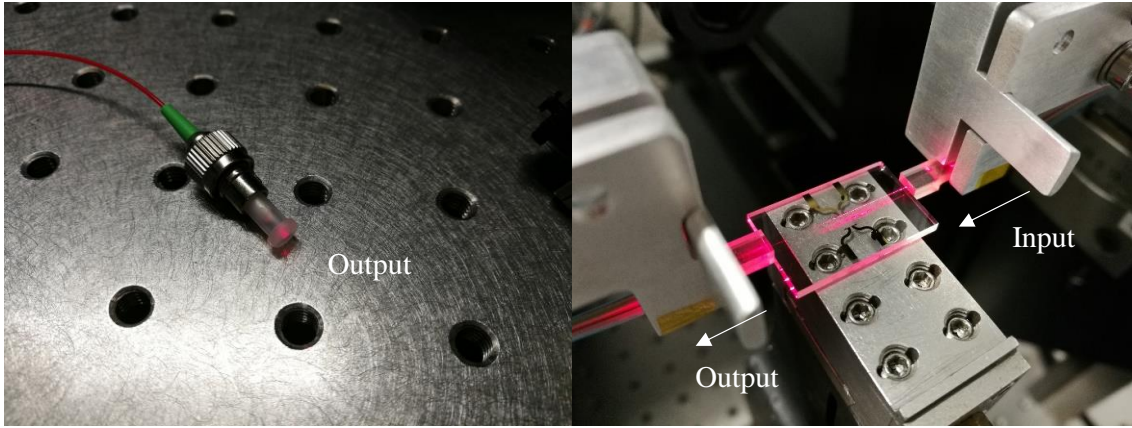
Fig. 5.17. Ion-exchanged waveguide probing using visible red laser. Image shows that light passes through the waveguides without obstruction.
