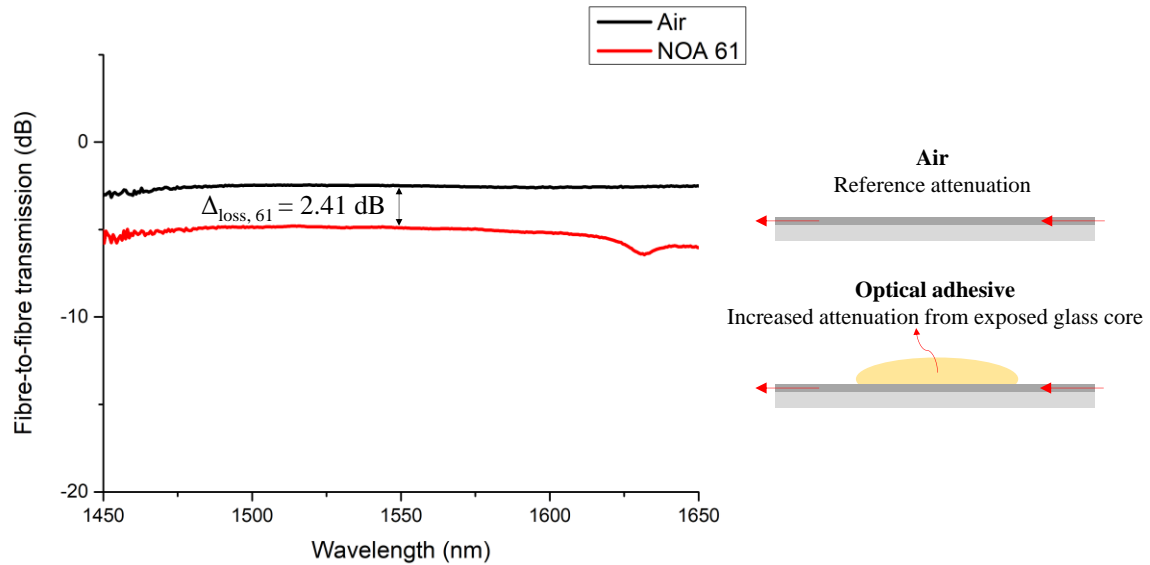
Fig. 5.19. Attenuation response of ion-exchanged glass waveguide with air ( n = 1 ) and optical resin NOA 61 ( n = 1.56 ).
