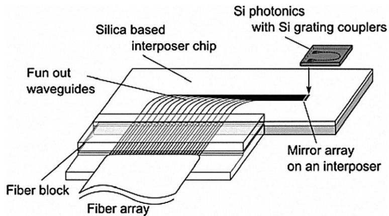
Fig. 1.13. Triplex optical interposer for silicon photonics integration from [35].
