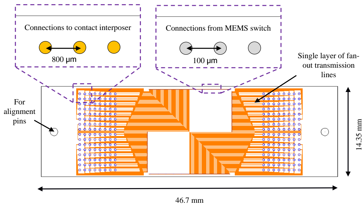
Fig. 3.7. Ceramic interposer design to redistribute 256 electrical bond pads from the MEMS device using single layer metallization with line width and space of 25 μm.
