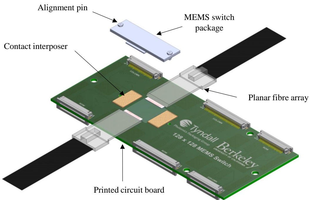
Fig. 4.1. Pluggable optical/electrical packaging concept, using reconfigured Test Vehicle 2a from Chapter 3 as example.
