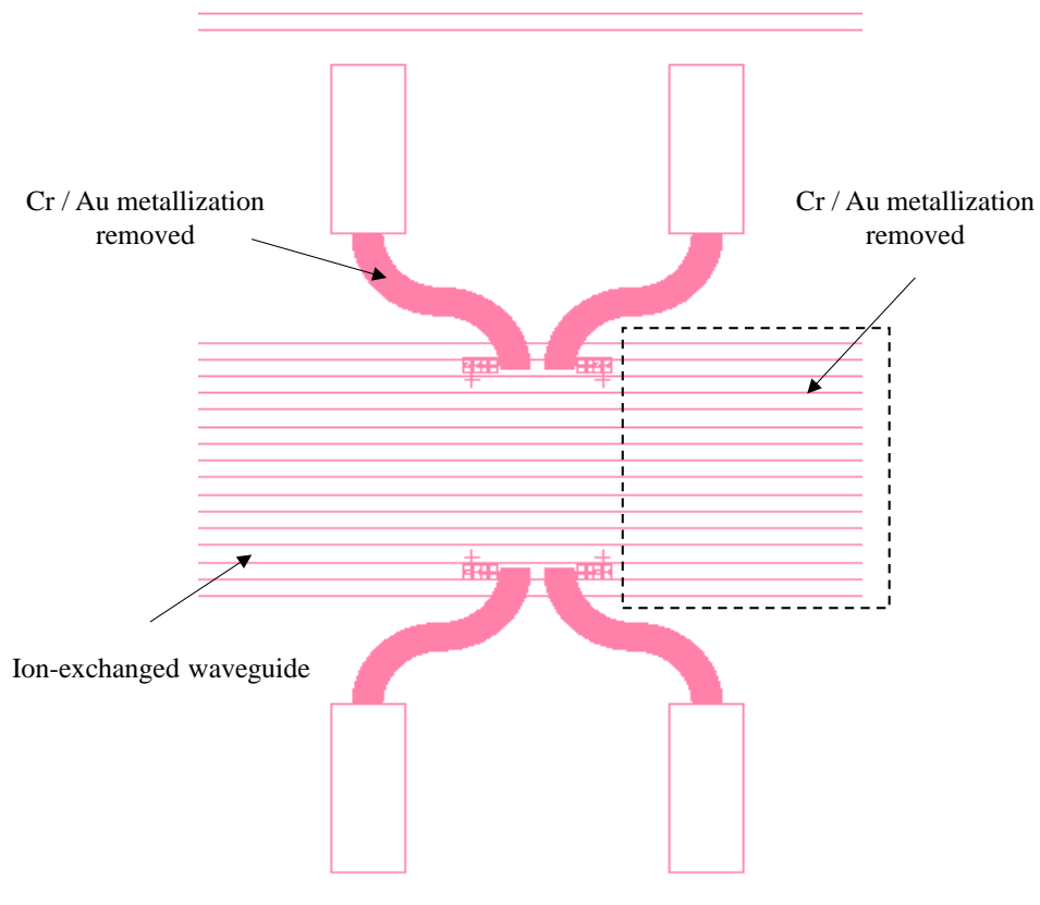
Fig. 5.16. Second design of glass interposer, whereby Cr/Au metallization above ion-exchanged waveguides have been removed.
