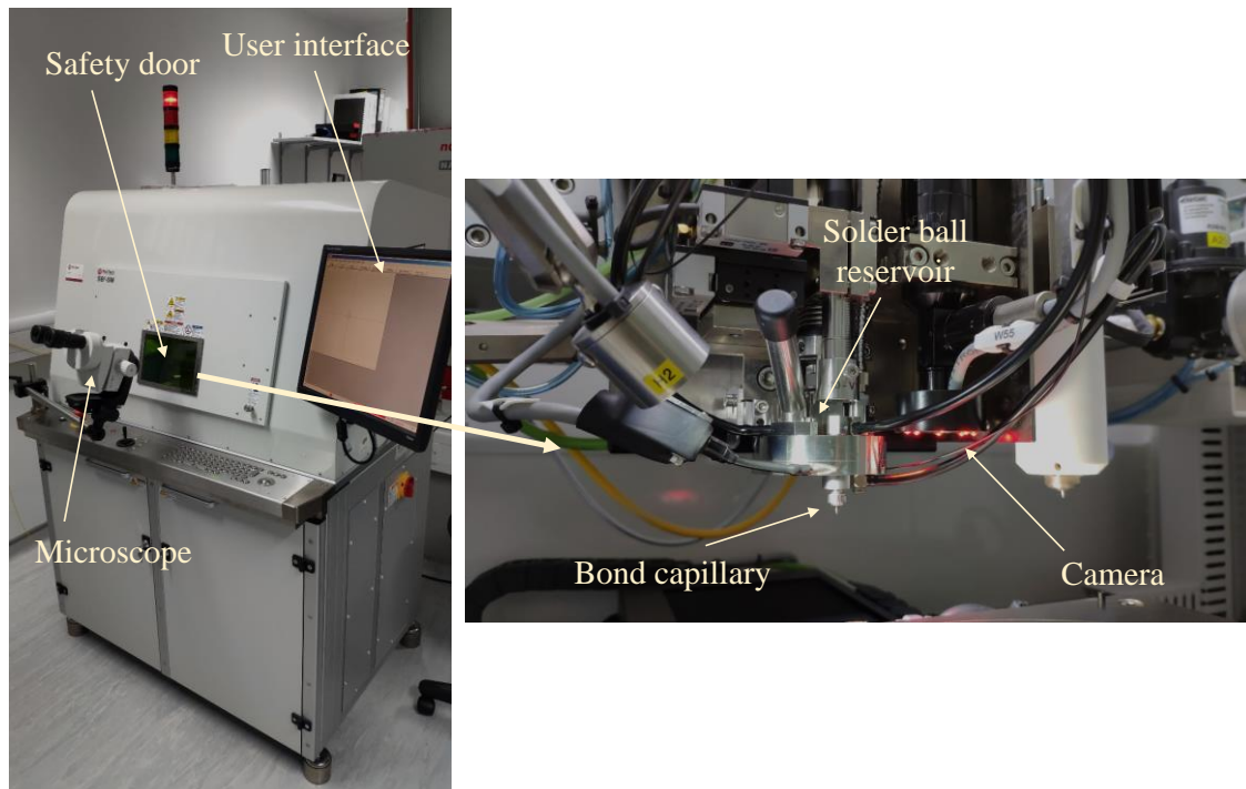
Fig. A3. Solder jetting system by Pactech (SB 2 -SM), used to form solder bumps on device bond pads. The system can currently process only \Phi 50\text{ }\mu\text{m} SAC 305 solder spheres. Operation can be automated with the help of bond map. Bond pad metallization preferably to be Au finishing for better wetting with Sn from SAC 305.
