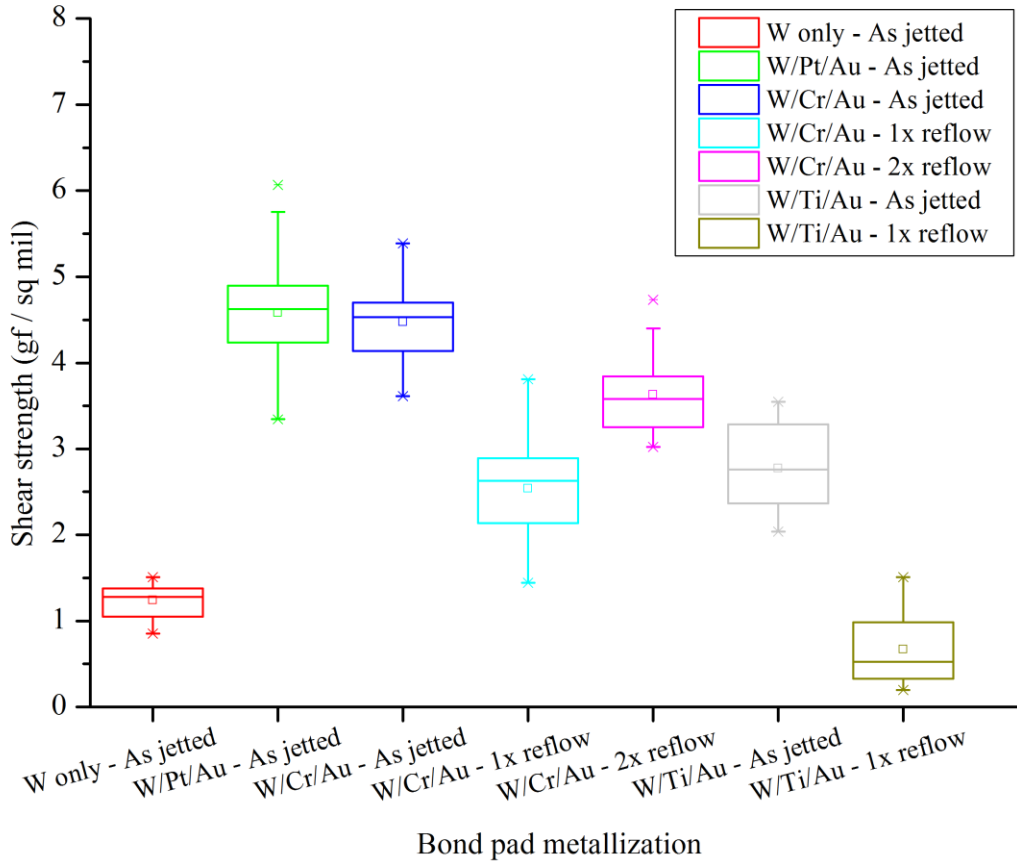
Fig. 3.17. Solder bump shear strength on various bond pad metallization, normalised against bond pad surface area. It can be seen that W/Pt/Au and W/Cr/Au metallization gave the best solder shear strength. The number of solder bump shear performed on all types of bond pad metallization was 20 bumps on 2 samples.
