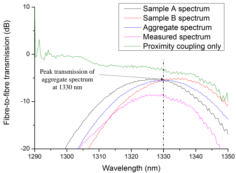
Fig. 4.10. Subtraction of aggregate spectrum (blue) from measured spectrum (pink) to obtain gratings-to-gratings coupling only spectrum (green).
