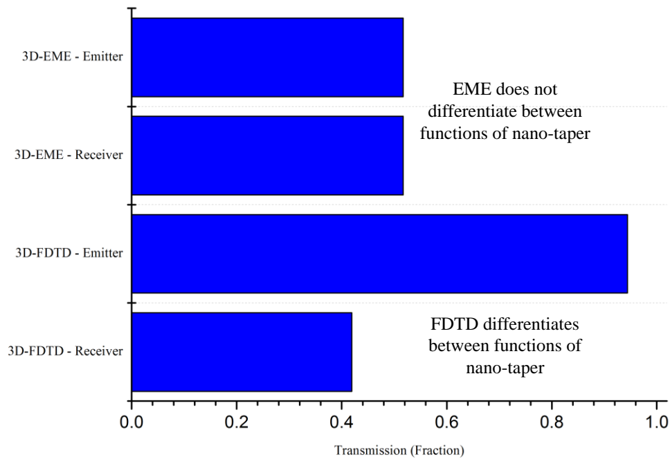
Fig. 5.26. Difference between MODE-EME and 3D-FDTD, using silicon nano-taper design 1 as simulation structure.
