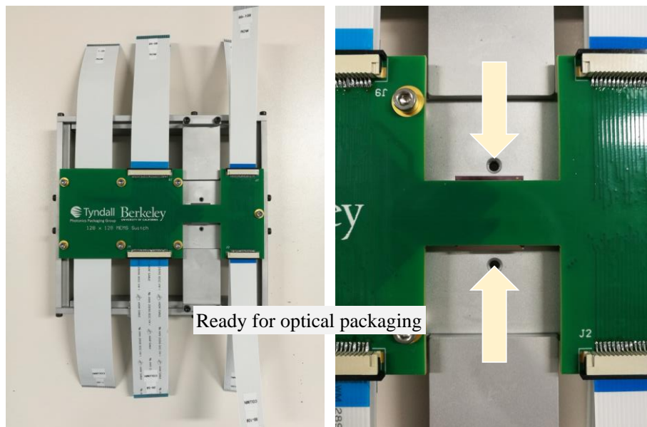
Fig. 3.24. Board level assembly onto mechanical mount, ready for subsequent optical assembly.
