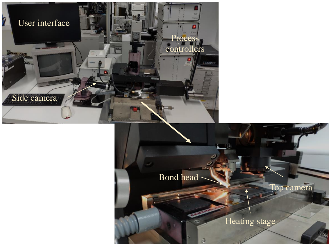
Fig. A4. Flip chip bonder by Finetech (Fineplacer lambda), used for flip chip and thermo-compression bonding of various components. Can go up to 40 N force and 400 °C reflow. Maximum alignment field of view of 2.5 mm x 2.5 mm at highest magnification. Alignment between top and bottom components are based on matching fiducials (alignment marks) on both components.
