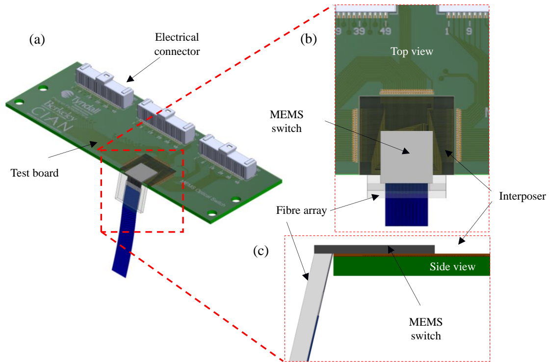
Fig. 2.5. 3-D SolidWorks models showing (a) the expected package assembly, (b) top view of the model showing FA alignment onto device, interposer and PCB and (c) side view of the model showing that only a lidless fibre will be able to couple to the device gratings due to proximity to interposer edge.
