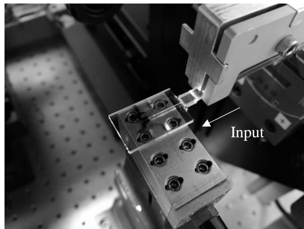
Fig. 5.14. Ion-exchanged waveguide probing using visible red laser. Image taken in monochrome shows that light passes through the waveguides but obstructed by Cr/Au metallization.
