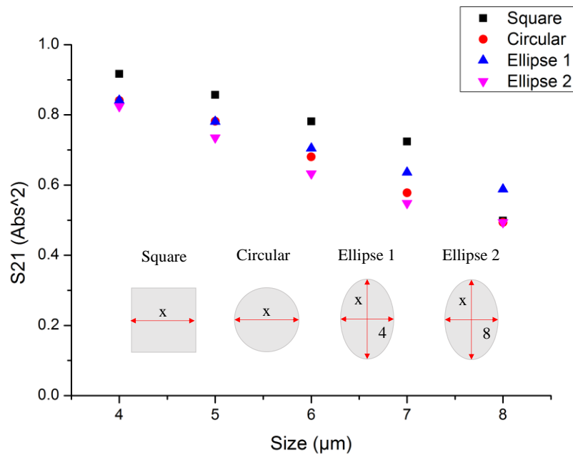
Fig. 5.4. Case (c), effect of glass waveguide size and shape. A square glass waveguide would improve coupling.
