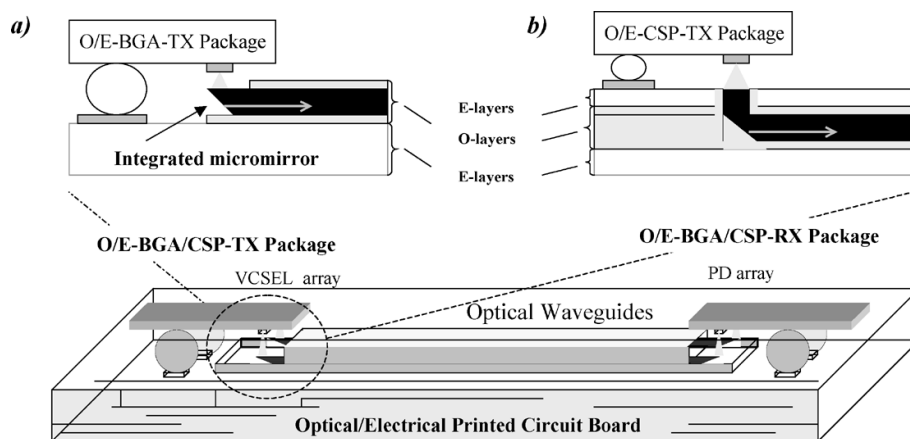
Fig. 1.8. Optical/electrical substrate using polymer waveguide with micro-mirrors from [30].
