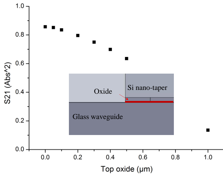
Fig. 5.8. Case (g), effect of oxide thickness on top of silicon nano-taper. Taper should be exposed and no TOX should cover it.
