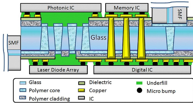
Fig. 1.15. Polymer plugged via to light coupling from [37].
