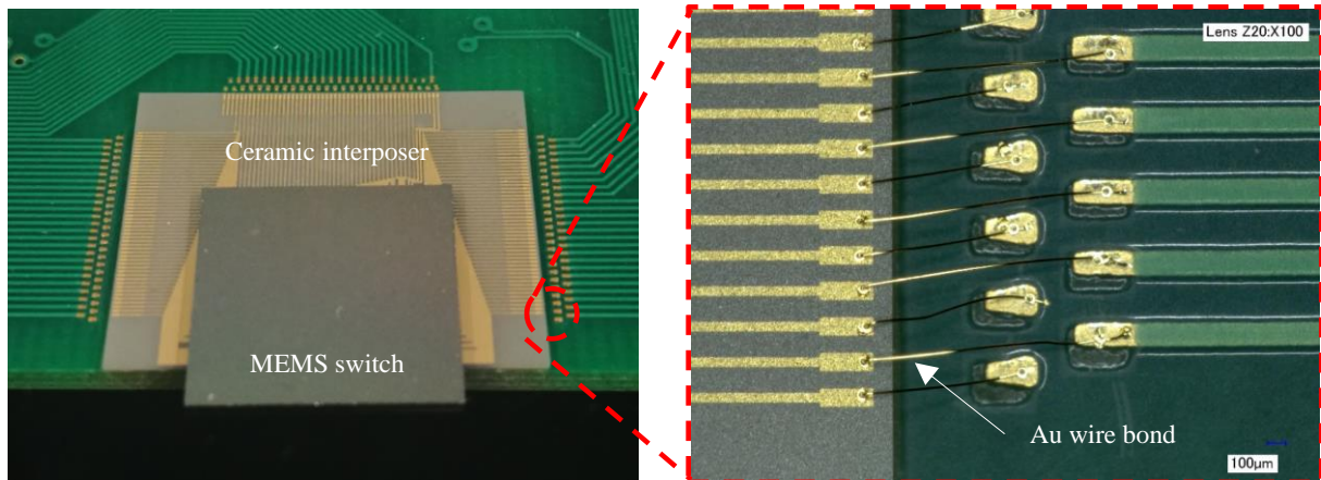
Fig. 2.7. Flip-chip assembly bonded onto PCB (left) and gold wires connecting AlN interposer to PCB (right).
