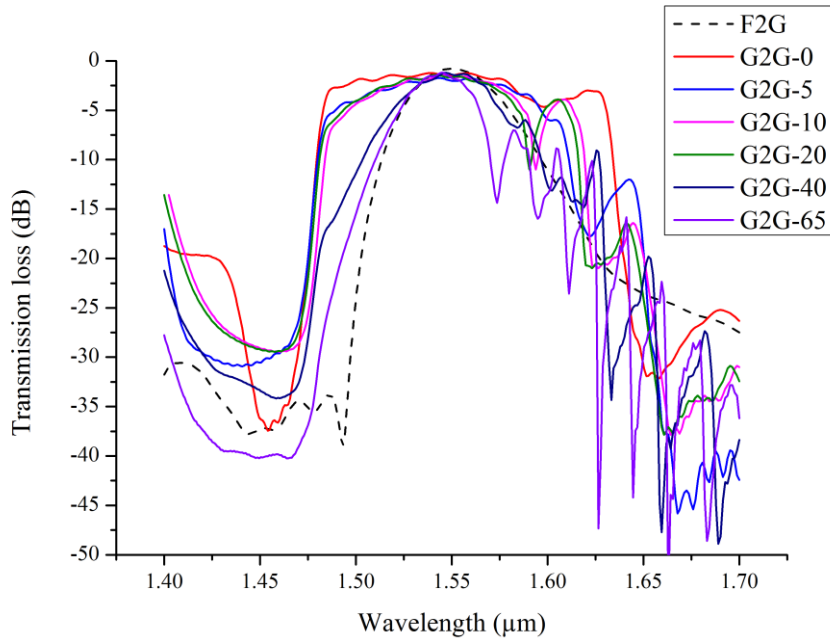
Fig. 4.17. Evolution of transmission losses and bandwidth as gap between the pair of vertically stacked gratings based on 340 nm SOI is increased.
