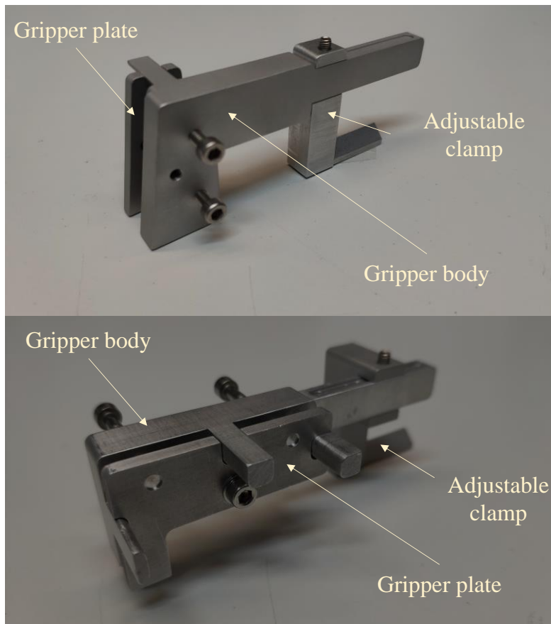
Fig. A7. Two of the fibre array grippers fabricated in this thesis, (a) for vertical fibre coupling and (b) planar fibre coupling.
