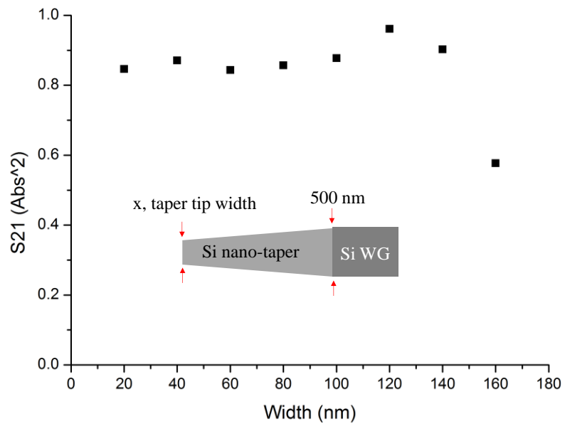
Fig. 5.5. Case (d), effect of silicon nano-taper tip. A clear coupling drop can be seen at taper width of 160 nm.
