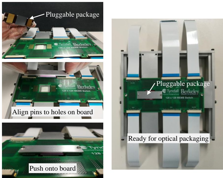
Fig. 3.20. Demonstration of the pluggable package onto test board (counter-clockwise from top left).
