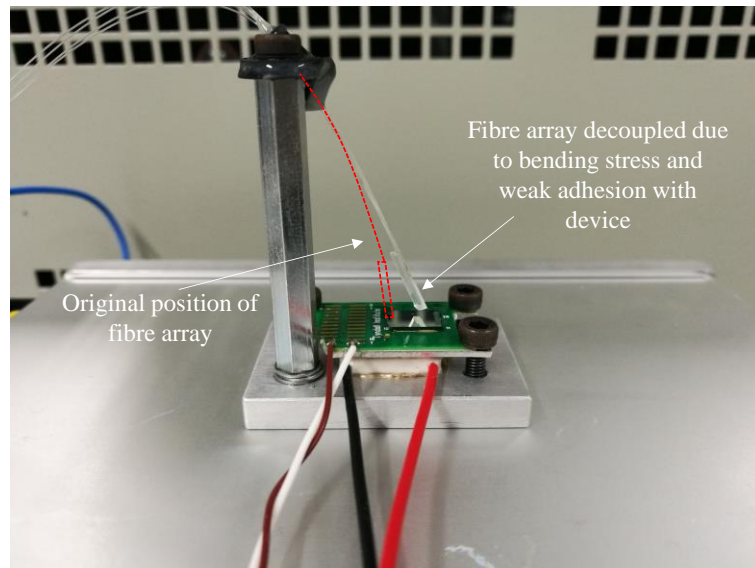
Fig. 1.7. Example of a decoupled vertical fibre array assembly due to bending stress and weak adhesion with device.
