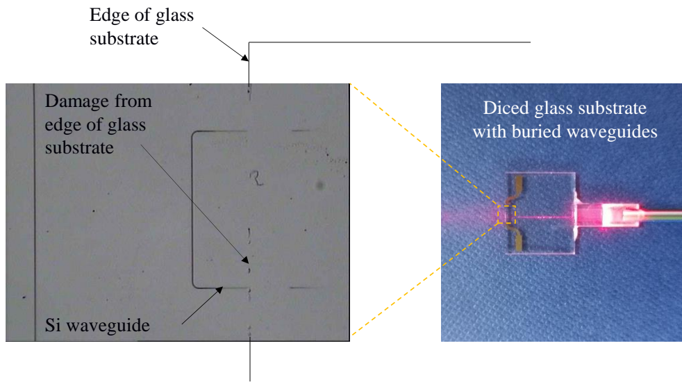
Fig. 5.24. Glass substrate was mechanically diced and polished in the middle to further reduce the contact area with silicon PIC, but caused burr damage on silicon waveguide instead.
