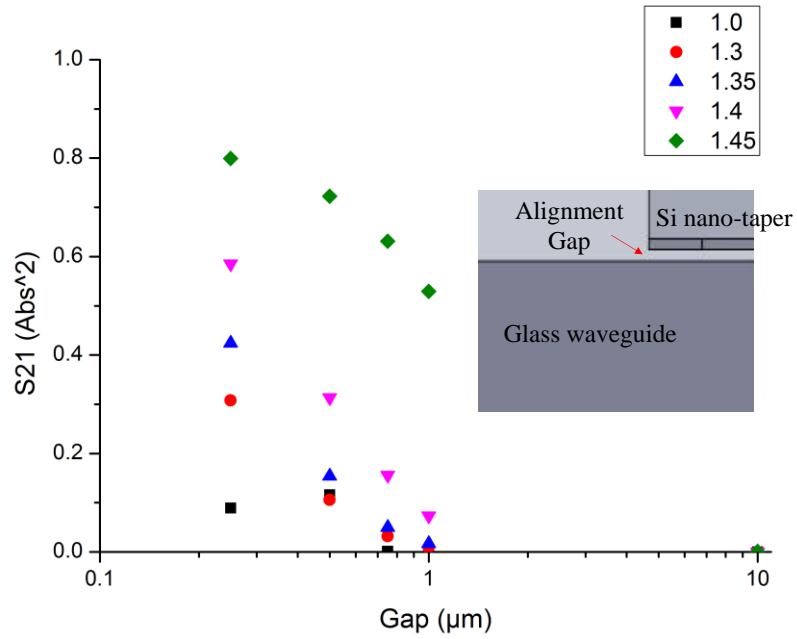
Fig. 5.7. Case (f), effect of assembly gap. Coupling falls drastically with increasing assembly gaps.
