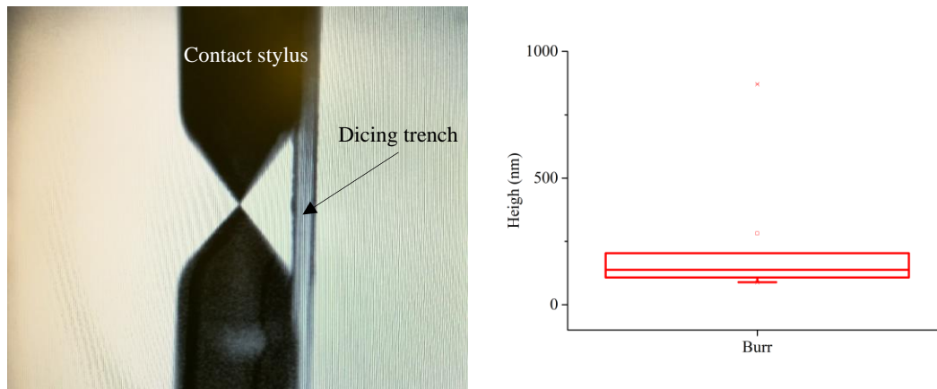
Fig. 5.25. Surface profiling of dicing burr. Graph shows the distribution of burr heights across different dicing trenches.
