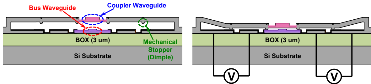
Fig. 2.1. Schematics of MEMS switch unit cell depicting coupler and bus waveguides, the mechanical stoppers and their operating principle during OFF state (left) and ON state (right).
