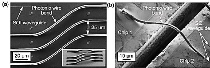
Fig. 1.11. Photonic wire bonds linking two devices from [33].
