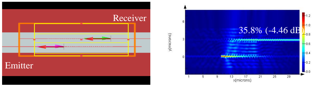
Fig. 4.3. 2D-FDTD simulation showing interaction between two vertically stacked uniform gratings at zero gap.
