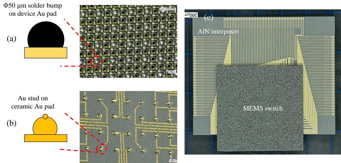
Fig. 2.6. (a) Solder (SAC 305) bumps on switch device and (b) gold (Au) stud bumps on ceramic interposer and (c) flip chip assembly of the device on interposer.
