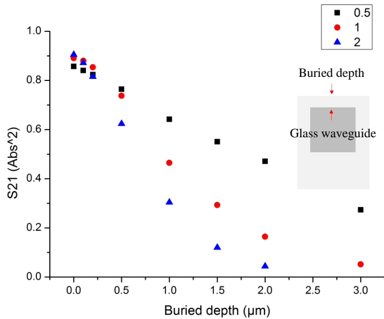
Fig. 5.6. Case (e), effect of buried depth of glass waveguide. Coupling falls drastically with increasing buried depth.
