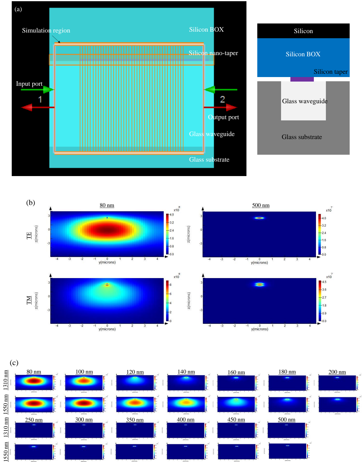
Fig. 5.1. (a) Simulation model, (b) TE-/TM-mode at start/end of taper and (c) TE-mode transfer at various taper width.
