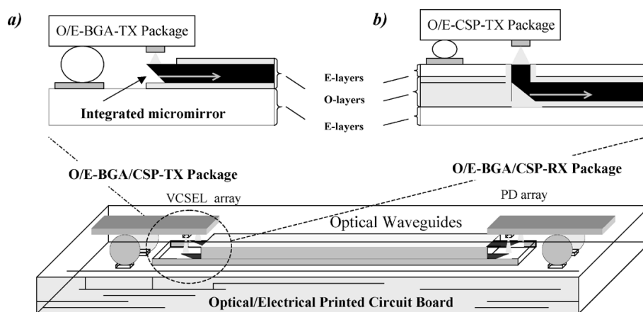
Fig. 1.8. Optical/electrical substrate using polymer waveguide with micro-mirrors from [30].
