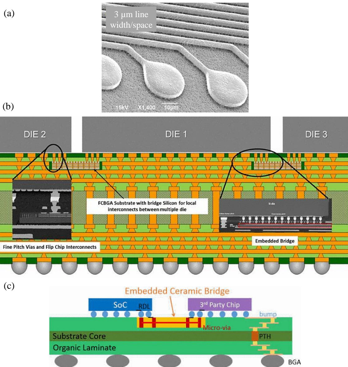
Fig. 1.4. Examples of interposer technologies. (a) Fine metallization lines on organic interposers from [13], (b) EMIB approach from [16] and (c) embedded ceramic concept from [20].
