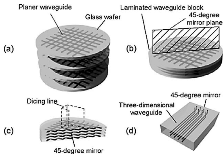
Fig. 1.12. Illustration of 3-D waveguides fabrication through lamination of planar polymer waveguide on glass from [34].
