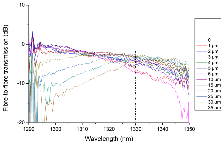
Fig. 4.11. Gratings-to-gratings coupling spectrums of various z-displacement from zero gap to 35 \mu\text{m} .
