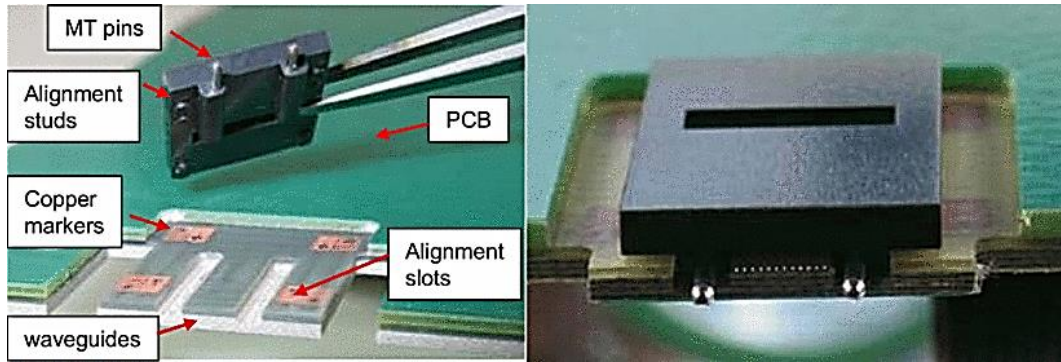
Fig. 1.9. Butt coupling concept of polymer waveguide within organic substrate from [31].
