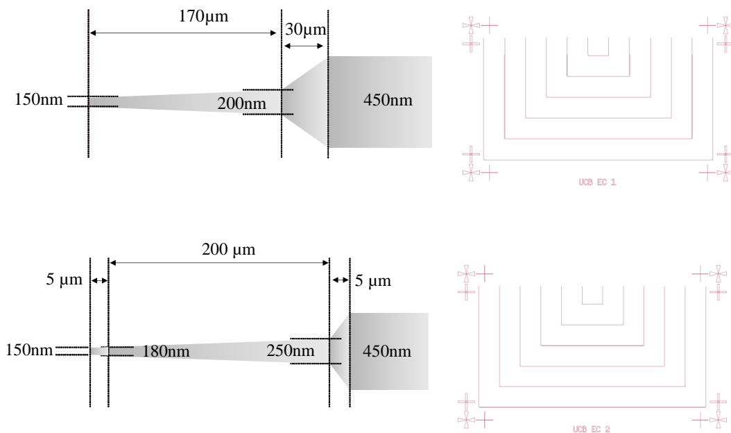
Fig. 5.12. Silicon nano-taper designed to match ion-exchange waveguide coupling on substrate.
