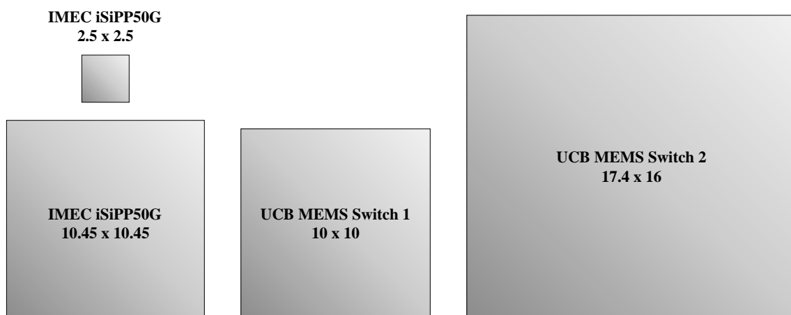
Fig. 1.17. Size comparison of the test devices from UC Berkeley that were used to develop packaging design and components in this thesis versus standard devices from MPW foundries such as IMEC.
