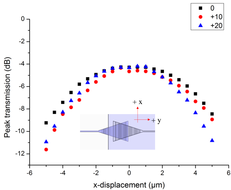
Fig. 4.13. Tolerance scan of coupling along the x-direction (across gratings) at various z-displacements.
