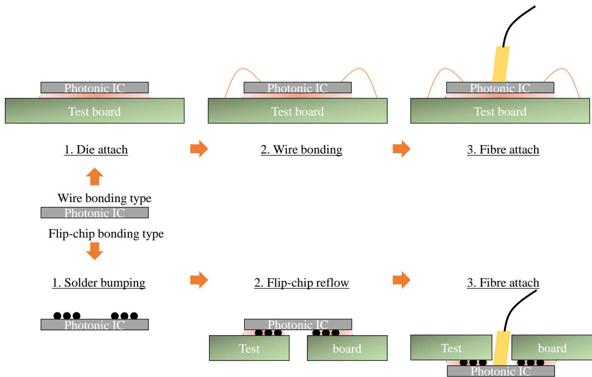
Fig. 1.2. Generic packaging sequence for silicon photonic devices. Note that fibre attach is always the last component to be assembled.
