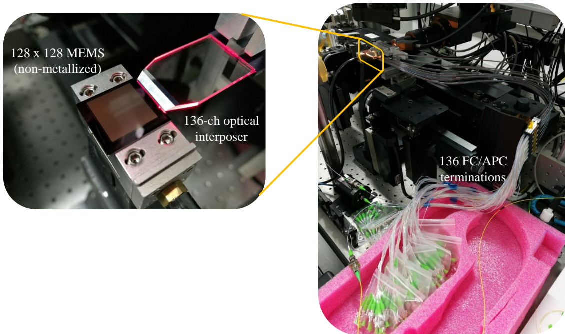
Fig. 3.28. Shunt transmission measurement of the MEMS switch device using the optical interposer.
