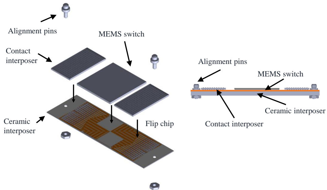
Fig. 3.9. Illustration of the pluggable package assembly with the contact interposers and alignment pins.
