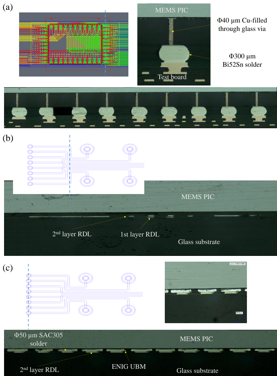
Fig. 3.27. Cross-sectional images of Test Vehicle 2b, highlighting assembly alignments at various sections (a) through via, (b) 2-layer RDL and (c) device bumps.
