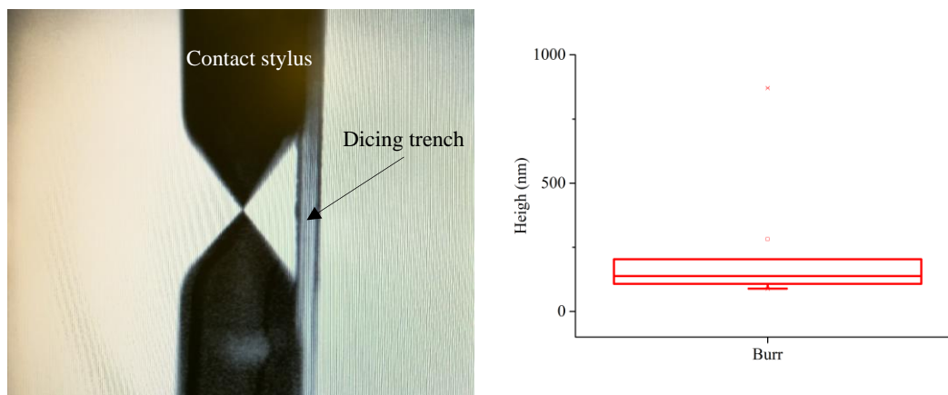
Fig. 5.25. Surface profiling of dicing burr. Graph shows the distribution of burr heights across different dicing trenches.
