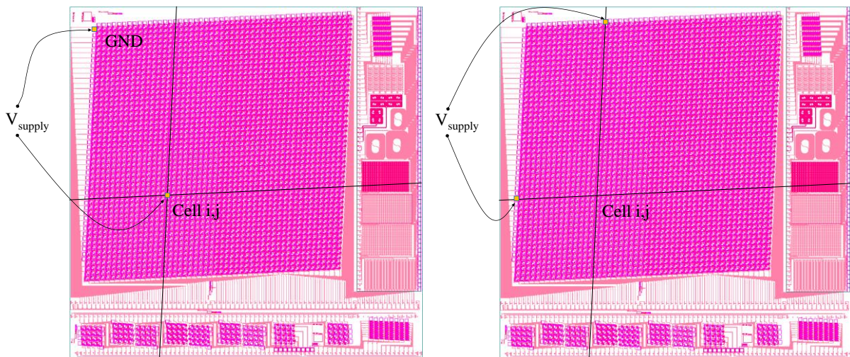
Fig. 3.1. Illustration of individual (left) versus row/column (right) addressing approaches on silicon photonic MEMS switch. Individual addressing requires 2500 electrical ports while row/column addressing requires only 100 electrical ports.
