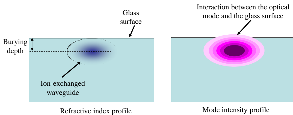
Fig. 5.9. Illustrations of the refractive index and mode intensity profiles of buried glass waveguides.
