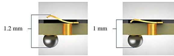
Fig. 3.8. Illustration of the off-the-shelf contact interposer before and after compression.
