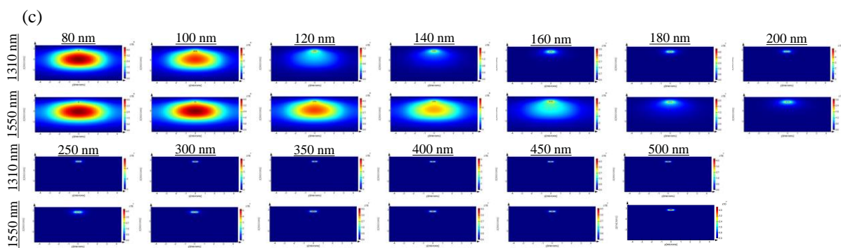
Fig. 5.1. (a) Simulation model, (b) TE-/TM-mode at start/end of taper and (c) TE-mode transfer at various taper width.
