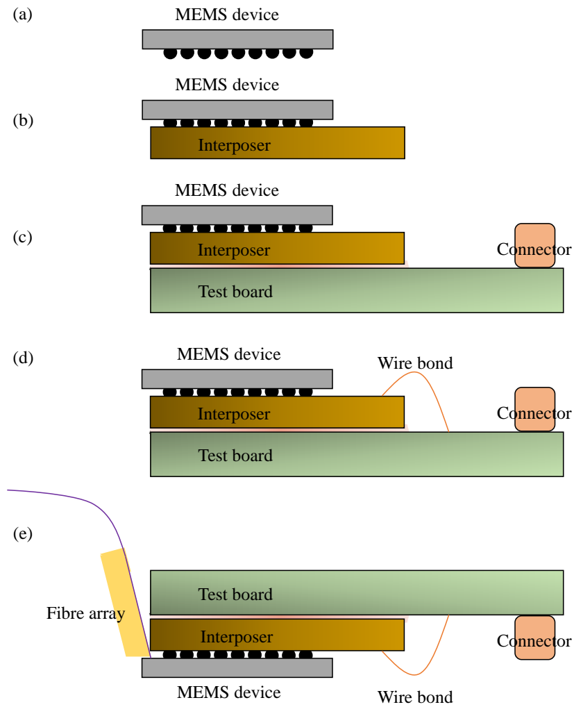
Fig. 2.3. Proposed packaging and assembly process flow for the silicon photonic MEMS device. (a) Solder bump formation on MEMS device, (b) flip-chip MEMS device onto interposer, (c) attach flip-chip assembly onto test board, (d) wire bond from interposer to test board, (e) optical assembly.
