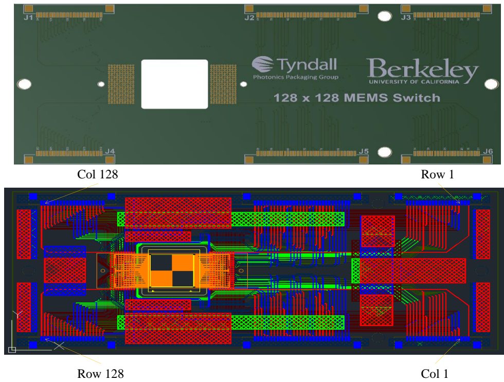
Fig. 3.10. Test board and overall electrical routing design (from MEMS switch device, through ceramic interposer and finally test board) for Test Vehicle 2a.
