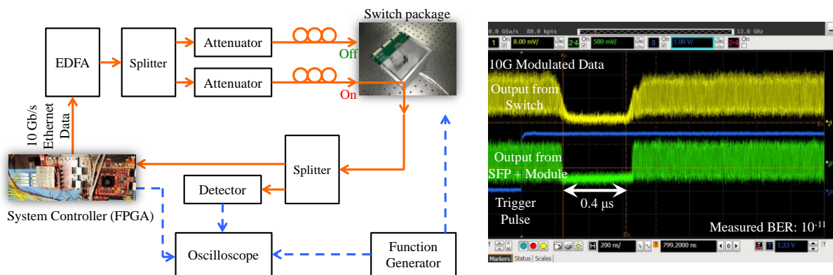
Fig. 2.11. Block diagram of system level characterization (left) and switching performance with 10 Gb/s data stream (right). Figures from UC San Diego.
