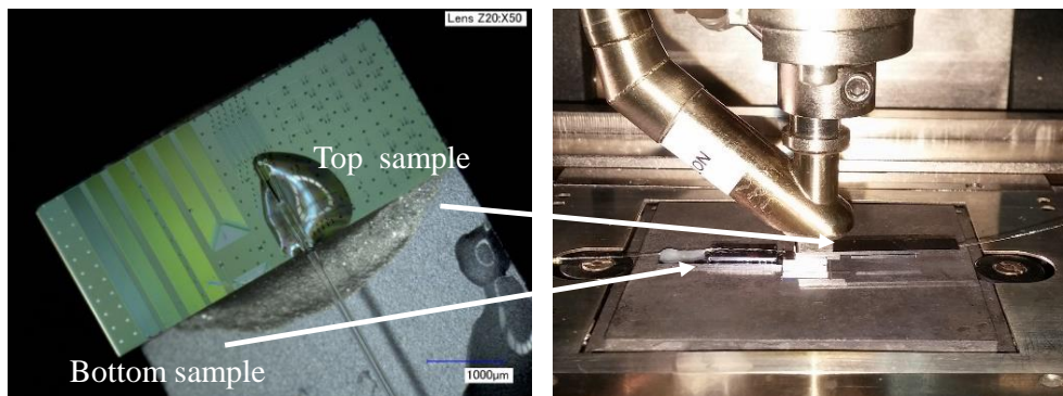
Fig. 4.7. Test samples with non-uniform gratings used in gratings-to-gratings coupling experiments. One sample was vertically stacked and aligned on top of another during flip chip assembly.
