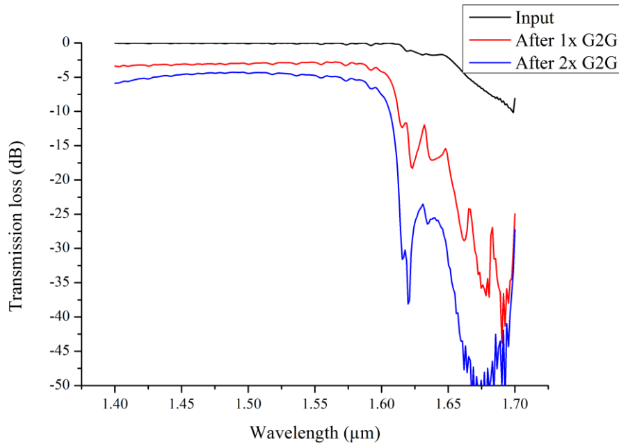
Fig. 4.19. Evolution of transmission losses and bandwidth after one and two pairs of vertically stacked gratings designed on 220 nm SOI.
