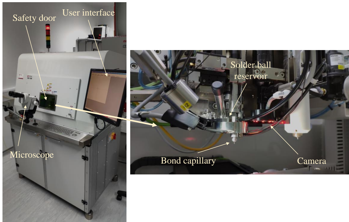
Fig. A3. Solder jetting system by Pactech (SB 2 -SM), used to form solder bumps on device bond pads. The system can currently process only \Phi 50 \mu\text{m} SAC 305 solder spheres. Operation can be automated with the help of bond map. Bond pad metallization preferably to be Au finishing for better wetting with Sn from SAC 305.
