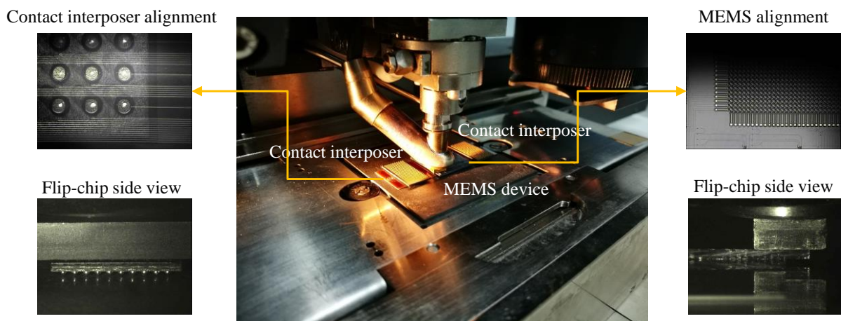
Fig. 3.18. Flip chip processing of the secondary contact interposer and 128 x 128 silicon photonic MEMS switch on AlN interposer.
