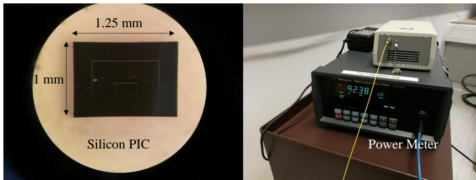
Fig. 5.23. Contact area reduction to reduce the assembly gap appears to be in the right direction with nW coupling power observed.
