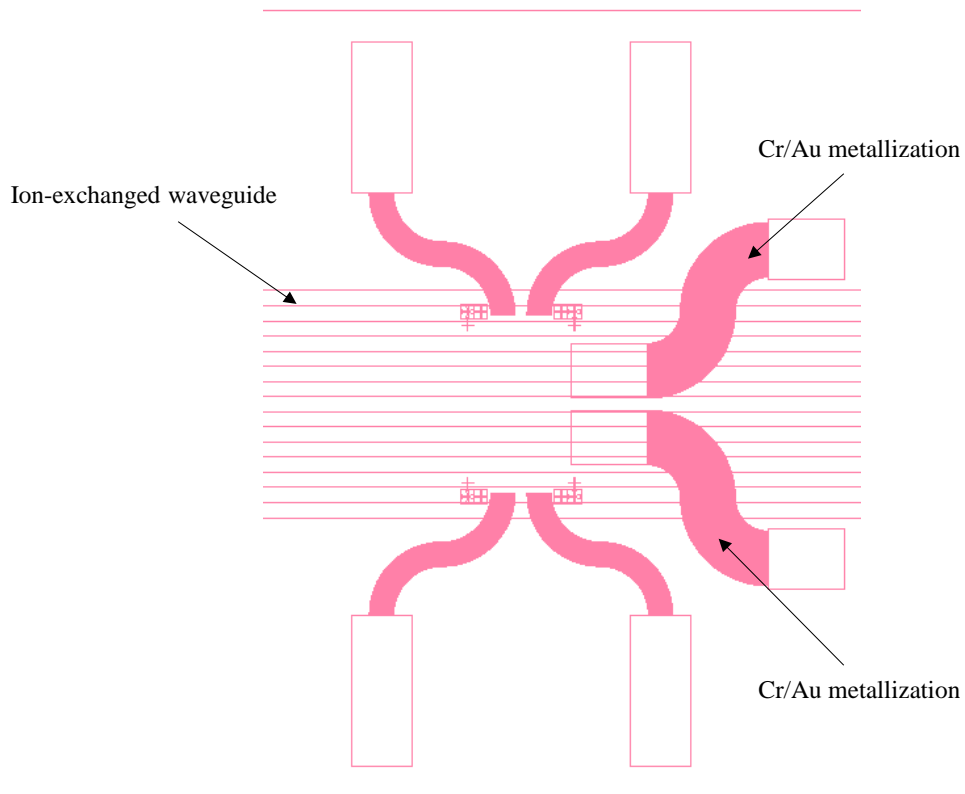
Fig. 5.13. Initial design of glass interposer with Cr/Au metallization on top of ion-exchanged waveguides.
