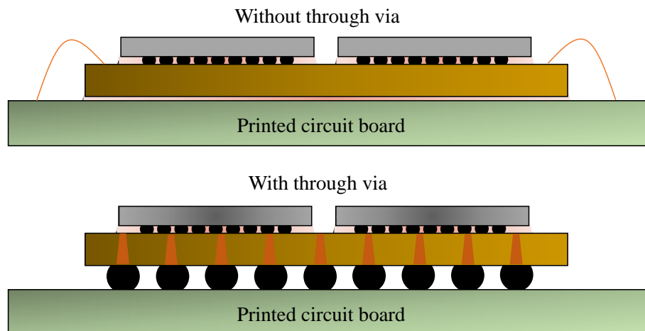
Fig. 1.3. Schematic of generic interposer (without and with through via) used for electrical interfacing between device and system board.
