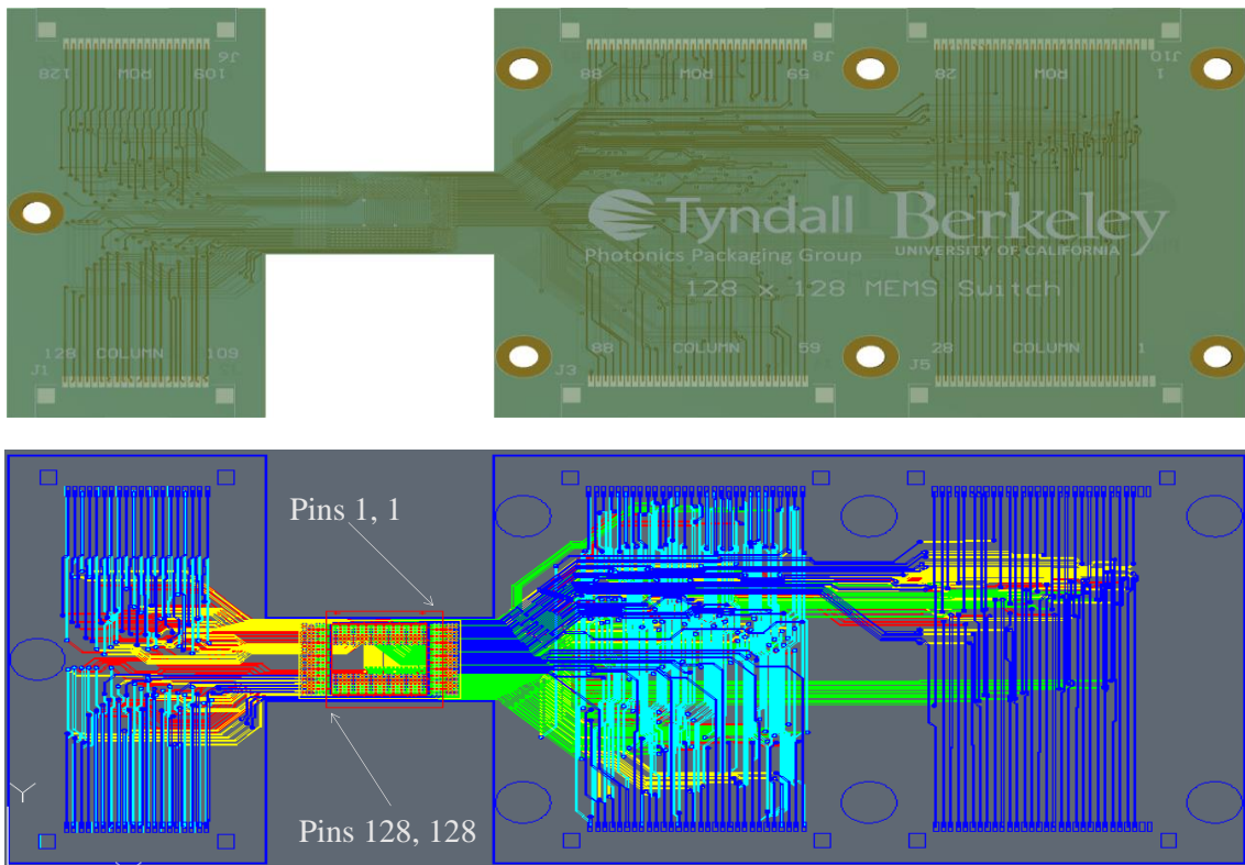
Fig. 3.12. Test board and overall electrical routing design (from MEMS switch device, through glass interposer and finally test board) for Test Vehicle 2b.
