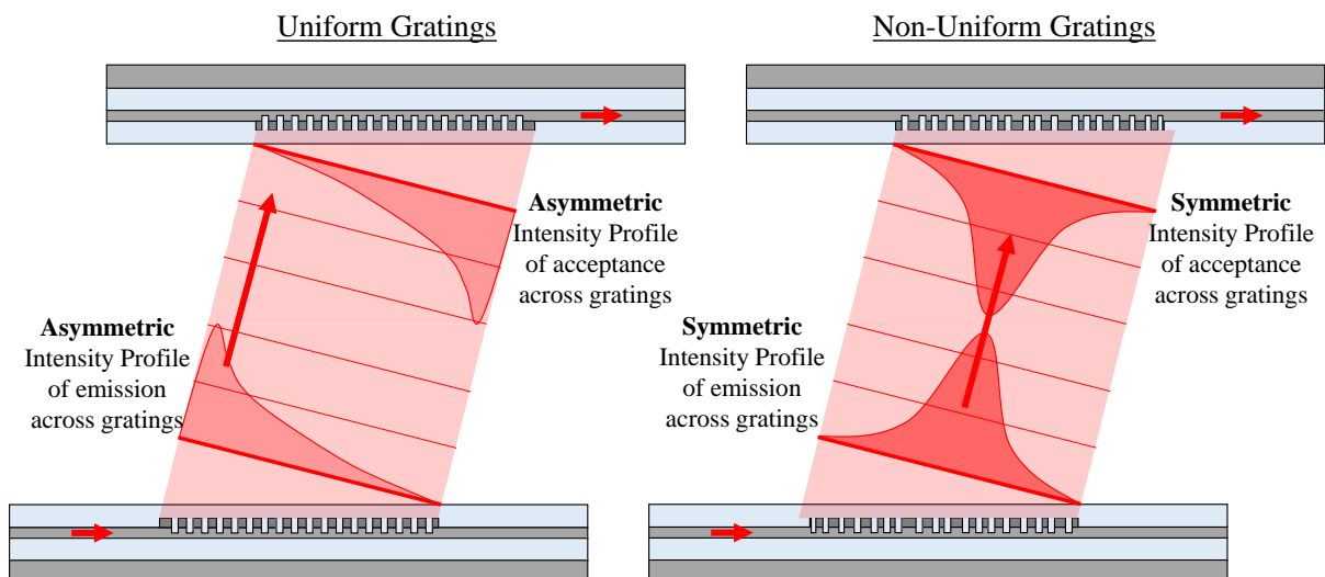
Fig. 4.5. Difference of mode profile between uniform and non-uniform gratings affecting coupling between them.
