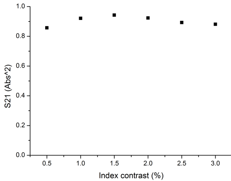
Fig. 5.3. Case (b), effect of index contrast. Index contrast should be low to maintain single mode transmission even though the coupling is weaker.
