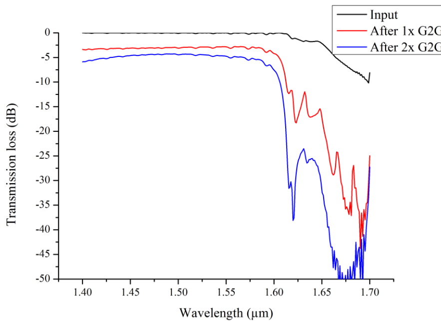
Fig. 4.19. Evolution of transmission losses and bandwidth after one and two pairs of vertically stacked gratings designed on 220 nm SOI.
