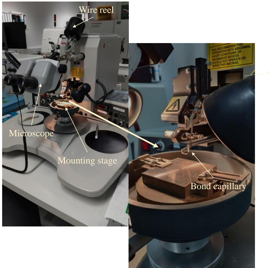
Fig. A2. Manual wire bonder by K&S used for Au stud bumping on device bond pads and wire bonding to connect device to interposer or test board. Typical wire diameter used on the system is 0.8 and 1.0 mil.
