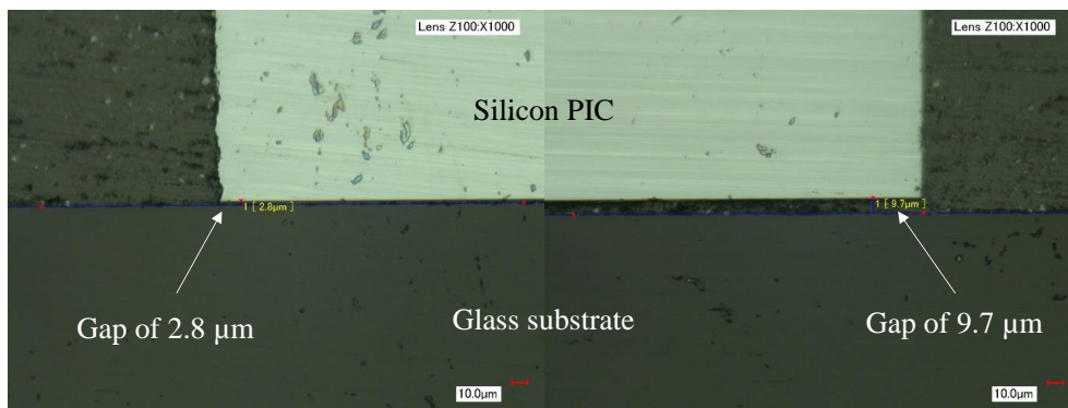
Fig. 5.22. Cross-section of the assembly shows that a gap ranging from 2.8 \mu\text{m} to 9.7 \mu\text{m} exists between silicon PIC and glass substrate.
