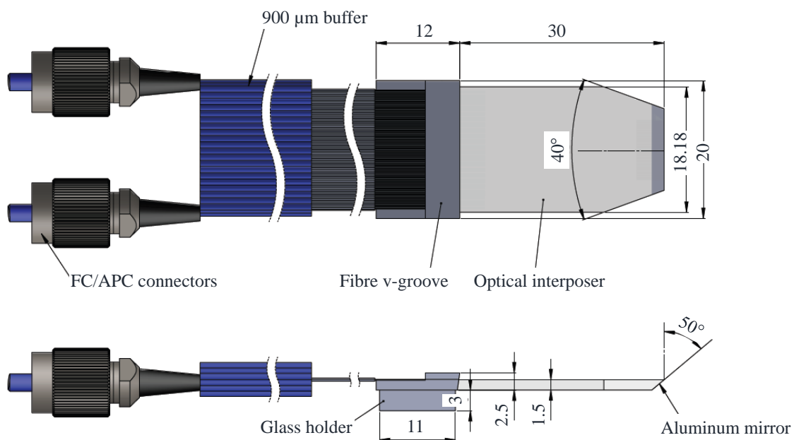
Fig. 3.14. Design of the planar optical interposer with pitch reducing optical waveguides buried underneath the glass surface. Figure from TEEM Photonics based on author's design specifications.
