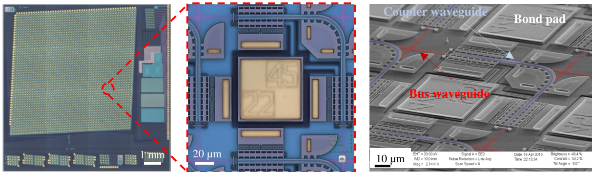
Fig. 2.2. Overview of the 50 x 50 switching device (left) used in packaging demonstration and a switch unit cell under optical (middle) and scanning electron microscope (SEM) (right).
