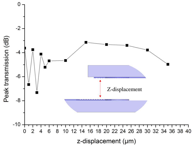
Fig. 4.12. Peak transmission variation with z-displacement. Oscillations can be seen between 0-10 \mu\text{m} displacements.
