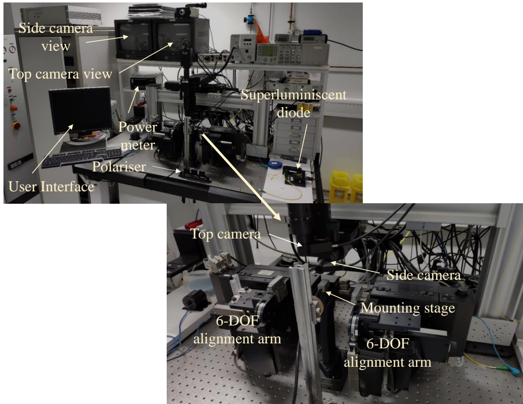
Fig. A1. Auto-aligner by Newport Corp. used for fibre alignment from 1-channel all the way to 136-channels as demonstrated in this thesis. The system consist of two 6-degree of freedom alignment arms, one top and one side view camera to assist with active alignment process. Suitable for vertical or planar fibre coupling, with the help of specially designed fibre array gripper. Travel distances of the alignment arms, top and side cameras have to be carefully considered during the design stage to prevent obstructions.
