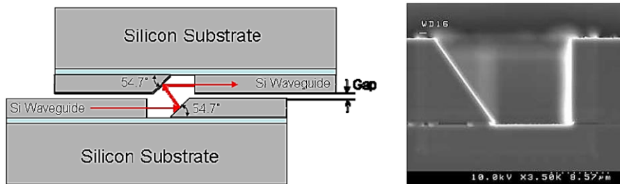
Fig. 1.16. Chip-to-chip optical proximity communication approach using silicon mirror from [38].
