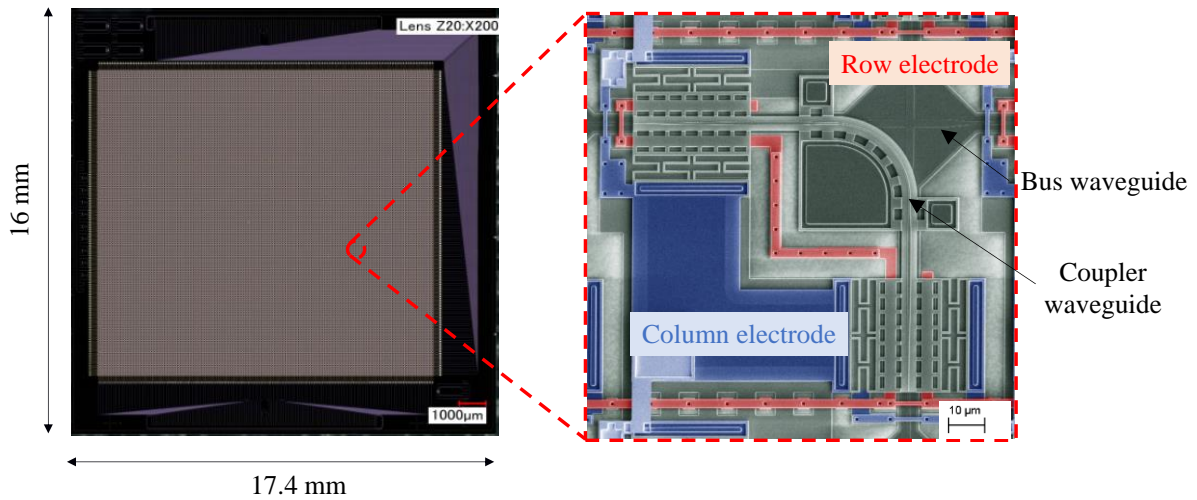
Fig. 3.4. Test device, 128 x 128 silicon photonic MEMS switch used for packaging demonstration and its MEMS switch unit cell.
