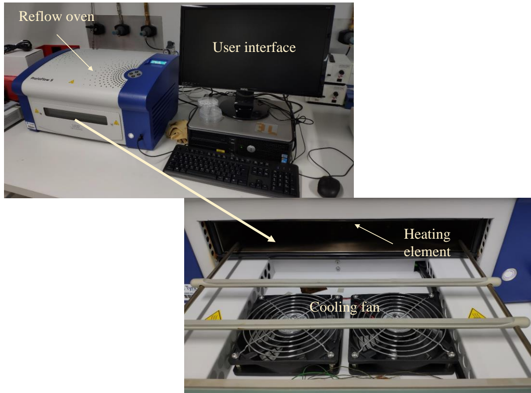
Fig. A5. Inert ( N_2 ) reflow oven by LPKF (Protoflow-S) used for board level reflow. Reflow temperature can reach 320 °C thus suitable for AuSn assembly. Can be used as curing oven for underfill and die attach as well.
