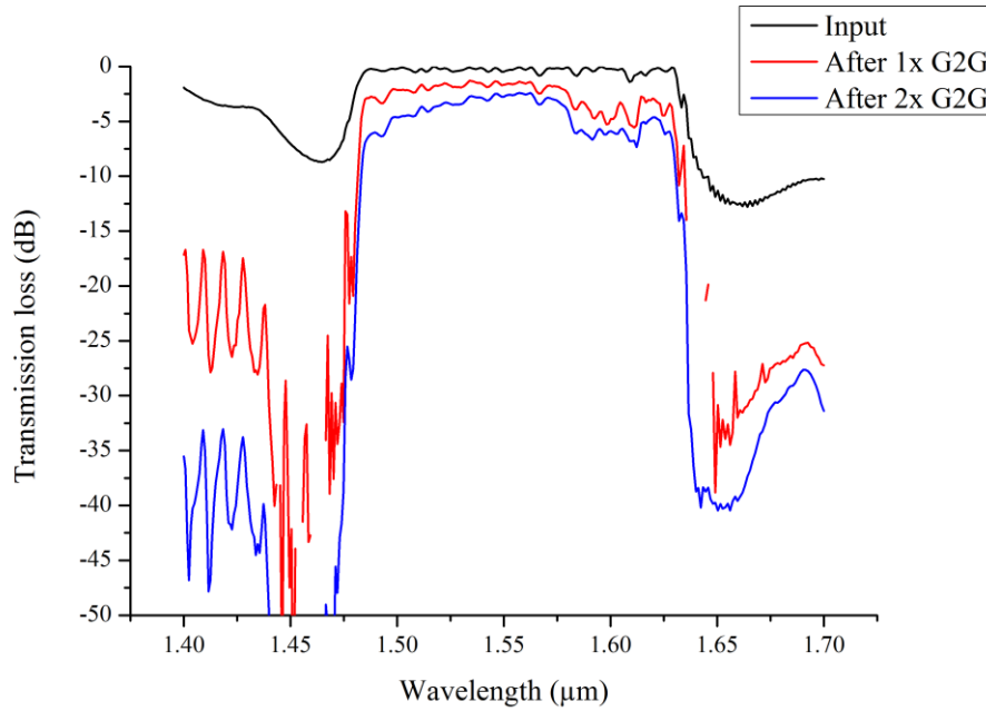
Fig. 4.20. Evolution of transmission losses and bandwidth after one and two pairs of vertically stacked gratings designed on 340 nm SOI.
