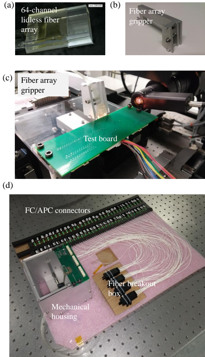
Fig. 2.9. (a) Lidless FA and (b) the FA gripper used during (c) active alignment. (d) The fully assembled optical switch package completed with mechanical housing.
