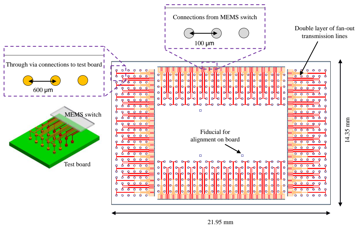
Fig. 3.11. Through glass interposer design consisting of two layers of redistribution lines (orange and red colour) and 512 through glass vias.
