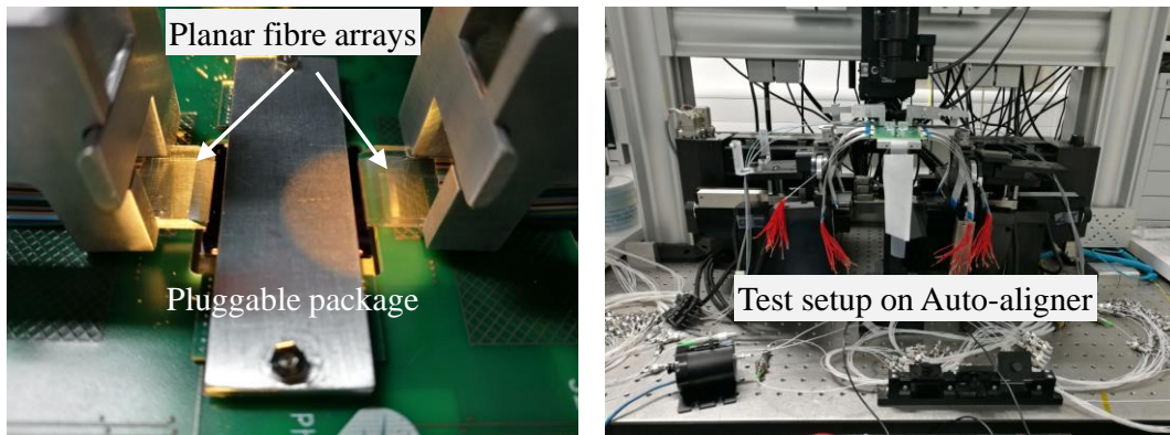
Fig. 3.29. Optical assembly test run on Auto-aligner using Test Vehicle 2a.
