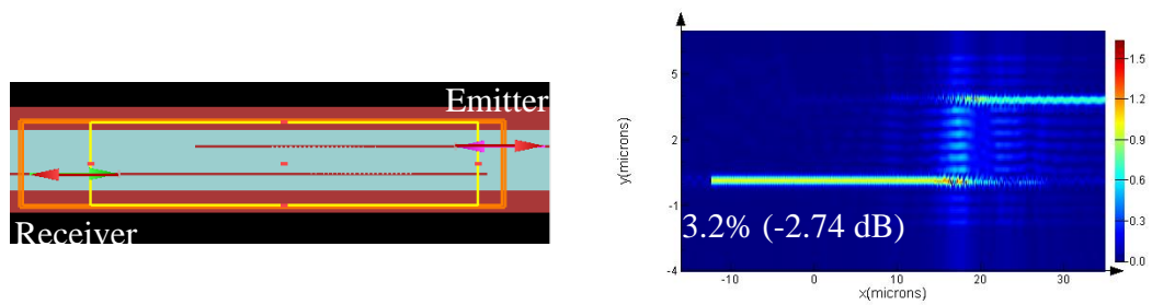
Fig. 4.4. 2D-FDTD simulation showing interaction between two vertically stacked non-uniform gratings at zero gap.
