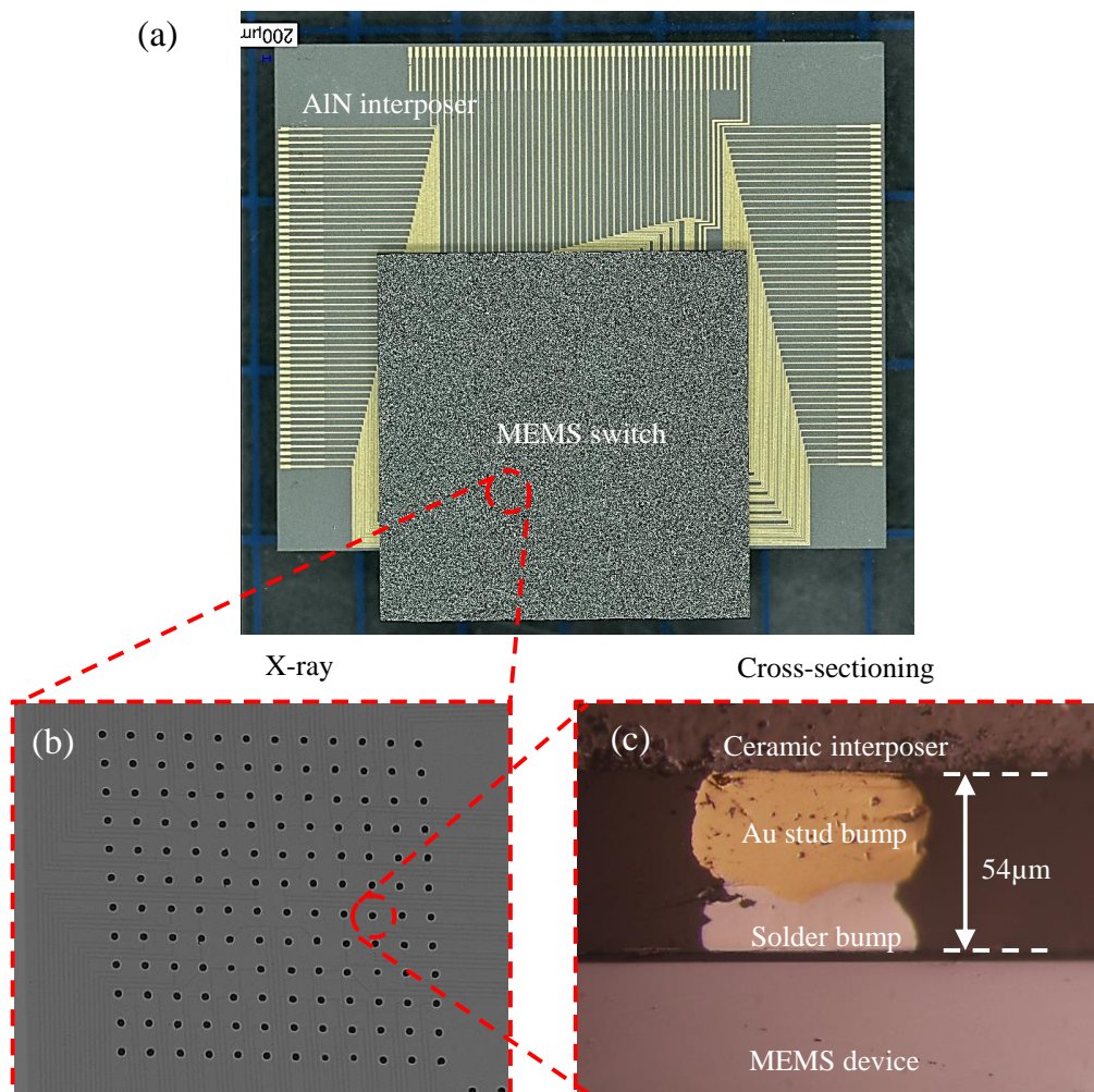
Fig. 2.8. (a) Overall assembly, (b) X-ray of flip chip assembly and (c) mechanical cross-section showing Au stud and solder bump alignment.
