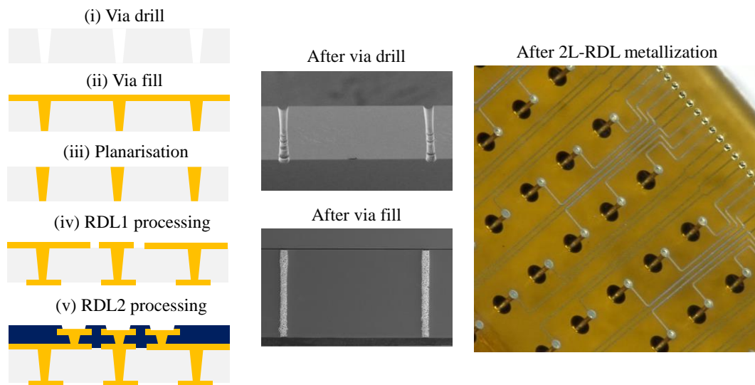
Fig. 3.21: Fabrication process flow (left), cross-sectional SEM images of drilled and filled via (middle) and after RDL metallization (right) of the through glass via interposer.
