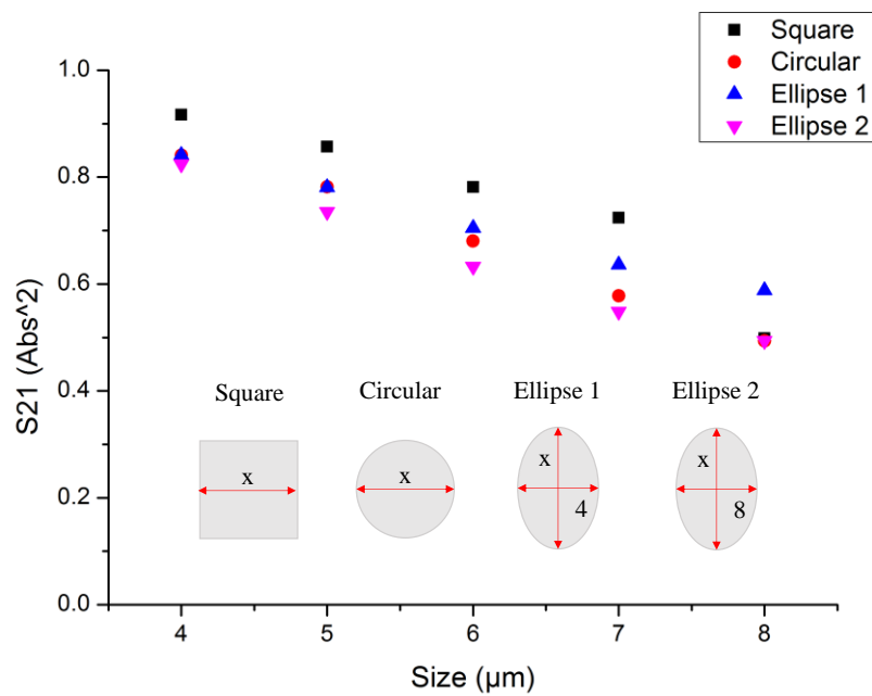
Fig. 5.4. Case (c), effect of glass waveguide size and shape. A square glass waveguide would improve coupling.
