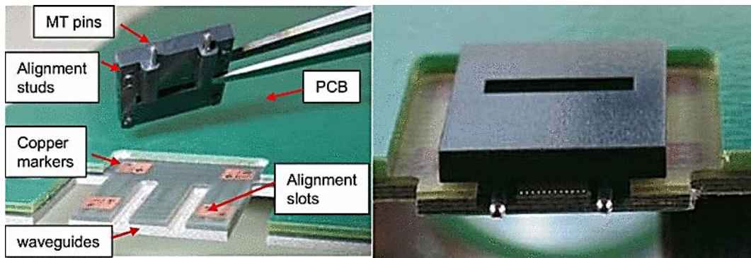
Fig. 1.9. Butt coupling concept of polymer waveguide within organic substrate from [31].
