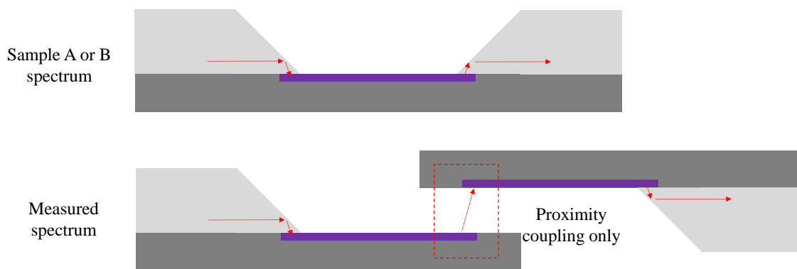
Fig. 4.9. Schematic depicting the various spectrums mentioned in Fig. 4.10.
