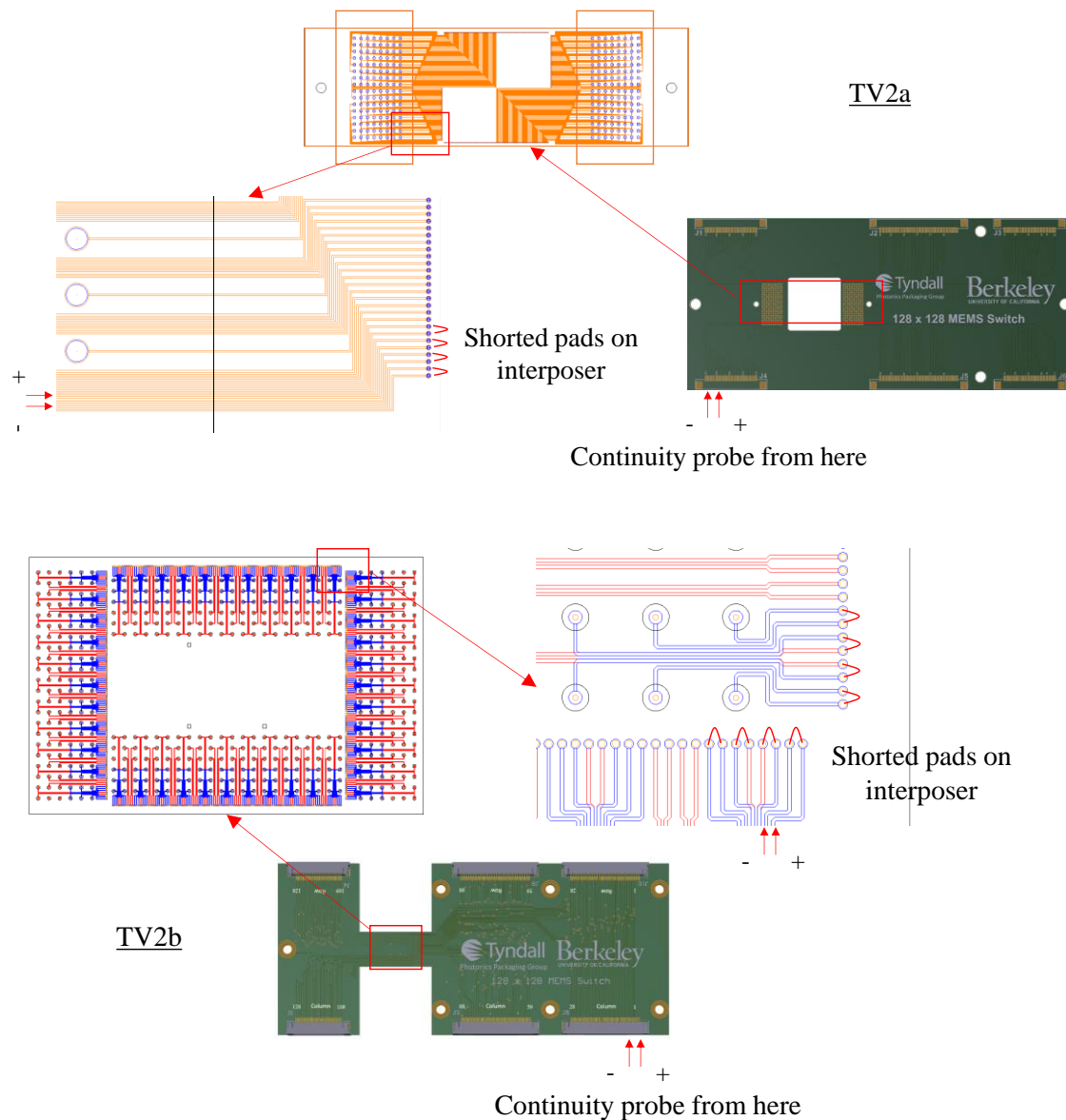
Fig. 3.25. Continuity measurement approaches on TV2a – pluggable (top) and TV2b - glass interposer (bottom) package assemblies.
