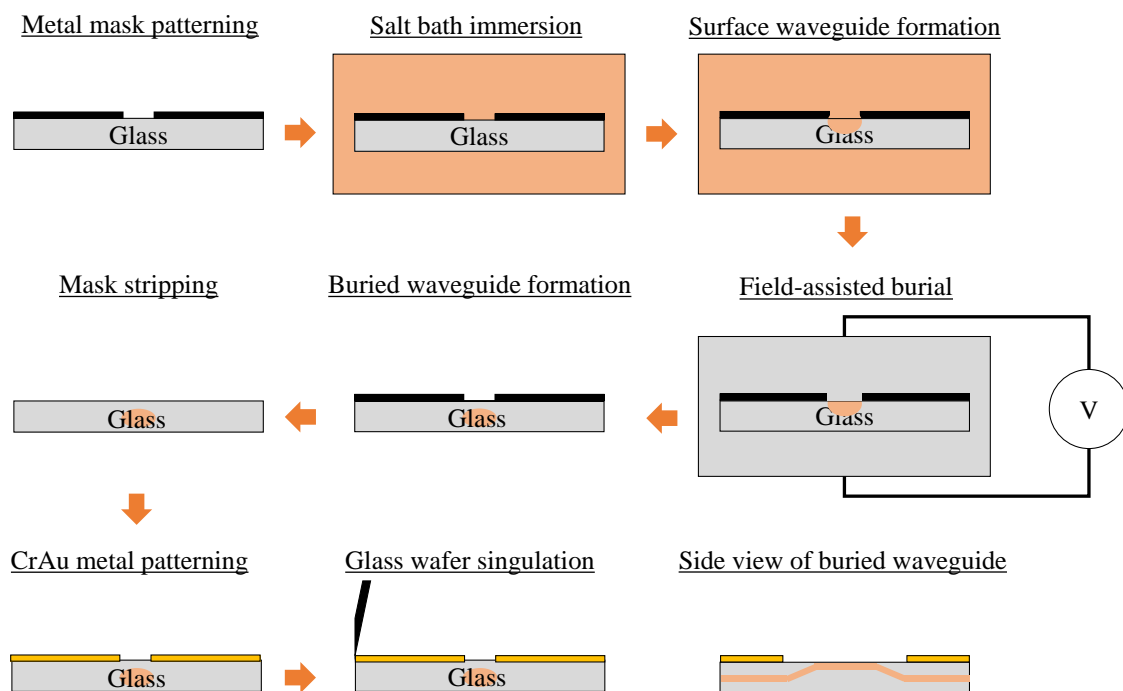
Fig. 5.10. Fabrication process flow of buried glass waveguide.
