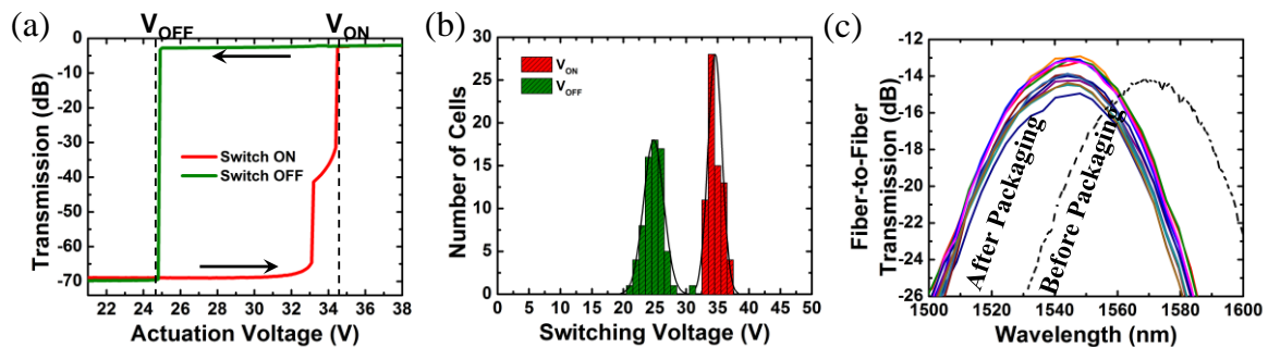
Fig. 2.10. (a) Measured transmission as a function of bias voltage of a switch cell, (b) switching voltage distribution of 70 MEMS switch cells and (c) fibre-to-fibre transmissions of various switch path. Figures from UC Berkeley.
