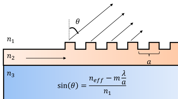
Fig. 1.5. Generic surface grating structure and its formula, where m is order of diffraction, \theta is angle of diffraction, \lambda is wavelength, a is grating period, n_1 , n_2 , n_3 are refractive indexes of layers 1, 2 and 3, n_{eff} is the average of index value of the thick and thin region of the grating.
