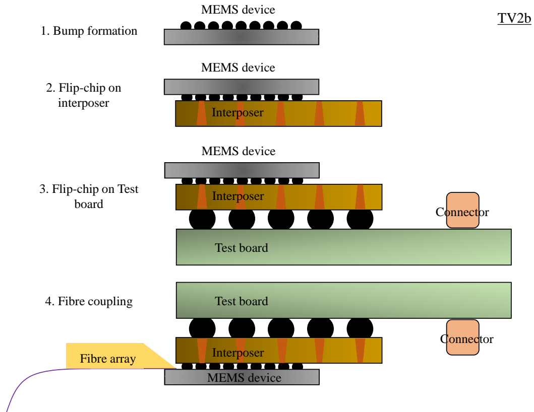
Fig. 3.6. Proposed Test Vehicle 2b (through glass via) packaging and assembly process flow for the silicon photonic MEMS device. (a) Solder bump formation on MEMS device, (b) flip-chip MEMS device onto interposer, (c) flip-chip assembly onto test board, (d) optical assembly.
