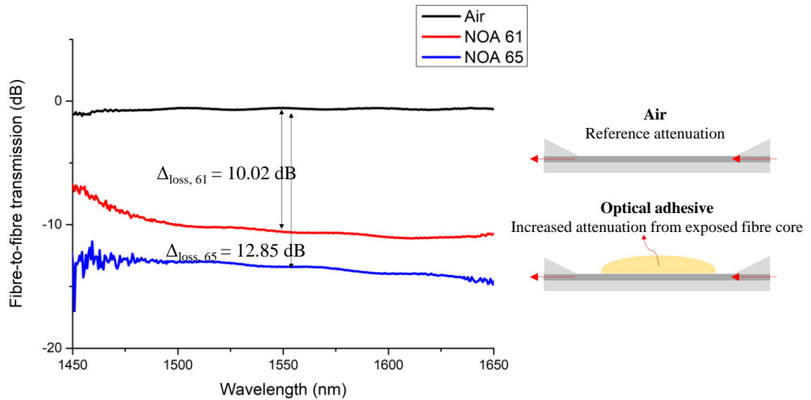
Fig. 5.18. Attenuation response of side-polished single mode fibre (SMF-28) with air ( n = 1 ), optical resin NOA 61 ( n = 1.56 ) and NOA 65 ( n = 1.524 ).
