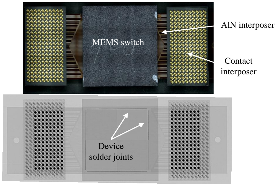
Fig. 3.19. Assembled pluggable MEMS switch package (top) and x-ray image of the assembly (bottom).
