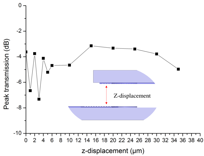
Fig. 4.12. Peak transmission variation with z-displacement. Oscillations can be seen between 0-10 μm displacements.
