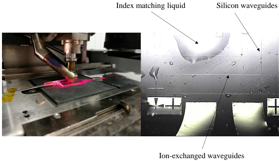
Fig. 5.21. First silicon device/glass substrate alignment and evanescent coupling test using Fineplacer Lambda.
