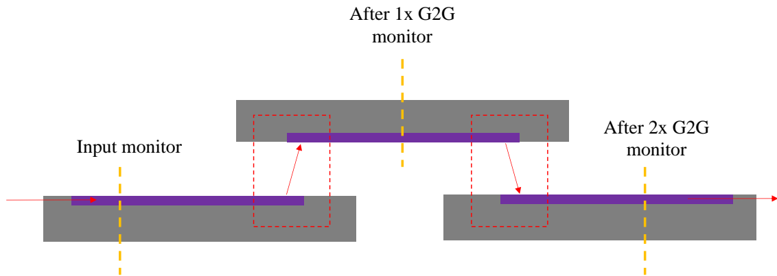
Fig. 4.18. Schematic illustrating the three spectrums found in both Figs. 4.19 and 4.20. The simulations were performed to observe the transmission losses, bandwidth and shape as a signal passed through the first grating-pair (input) and second grating-pair (output).
