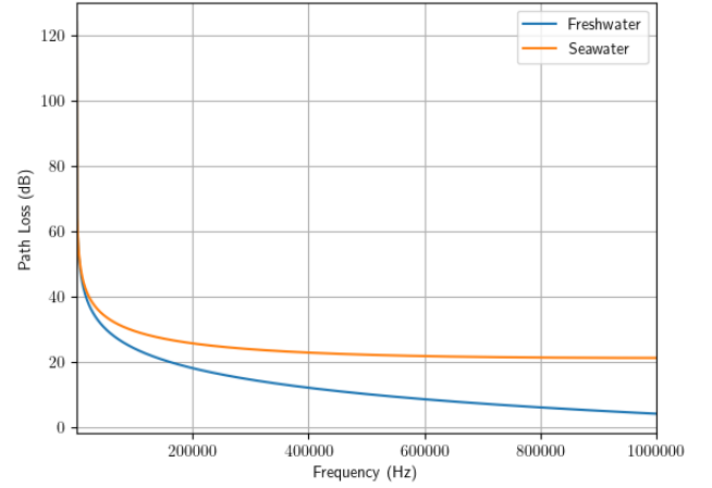
Figure 5. Path loss for an inductively coupled system at range z = 50\text{ cm} .
