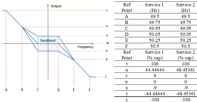
Fig. 4 Enhance frequency response envelope [18].
