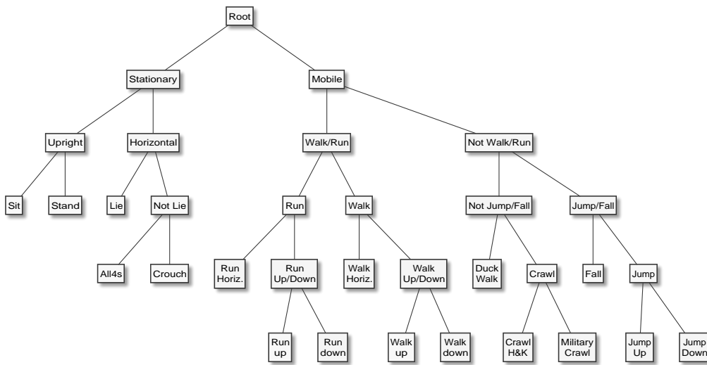
Figure A1. Expert hierarchy 1 (EH1).
