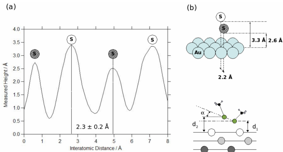
Fig. 4 (a) STM acquired height variation of two sulfur atoms forming a dimer. The data was acquired from the images such as those in Fig. 3(b). (b) Schematic representation of the S-S dimer on the Au{111} surface. The distances shown are measured from the surface plane and only one sulfur atom (Au-bridge site) is bound to the Au lattice. (c) Side-view of (b) showing S-S dimer position on Au{111}. (d_2 - d_1) represents the height displacement of the dimerizing S atom.
