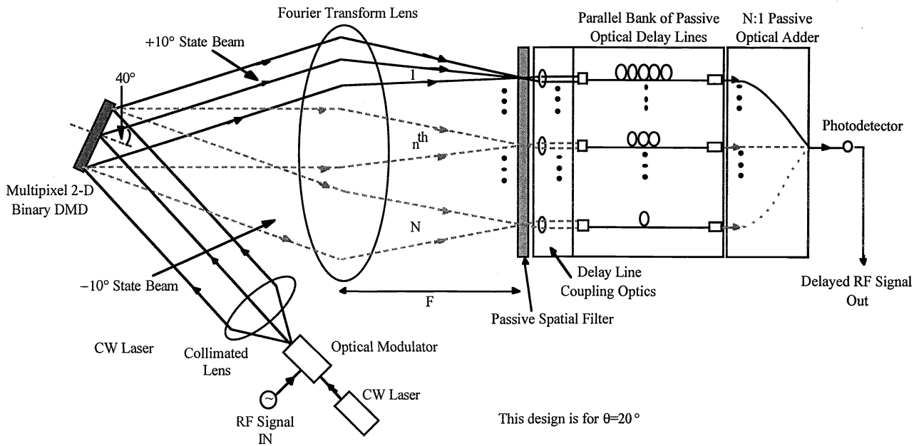
F: Focal length of Fourier Transform Lens, 1: All DMD Pixels at +10° state, n^{\text{th}} : Some DMD Pixels at +10° state Some at -10° state N: All DMD Pixels at -10° state
