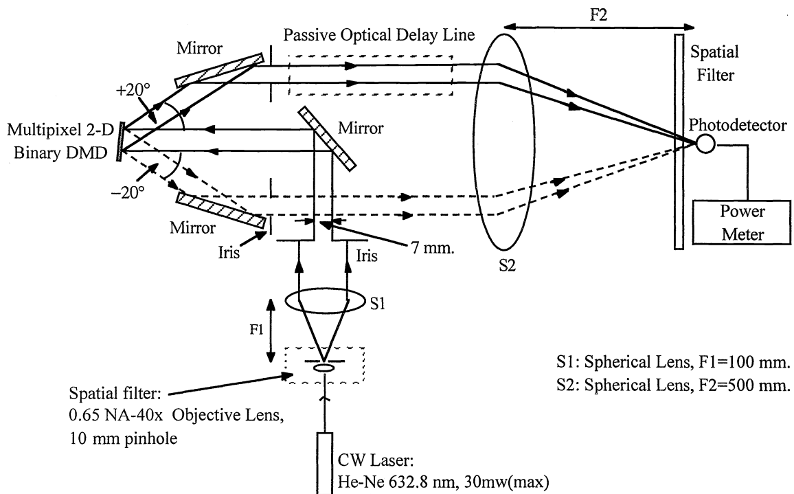
Fig.6: Shows the Laboratory Experimental Setup of our Basic Single Channel DMD Ray-Optics PDL Design.
