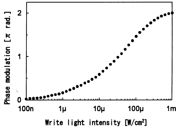
Fig. 4. Manufacturer Provided Experimental Phase Response at 633 nm Read Light versus 633 nm Write Light Intensity for Hamamatsu PAL LC SLM. [14]
