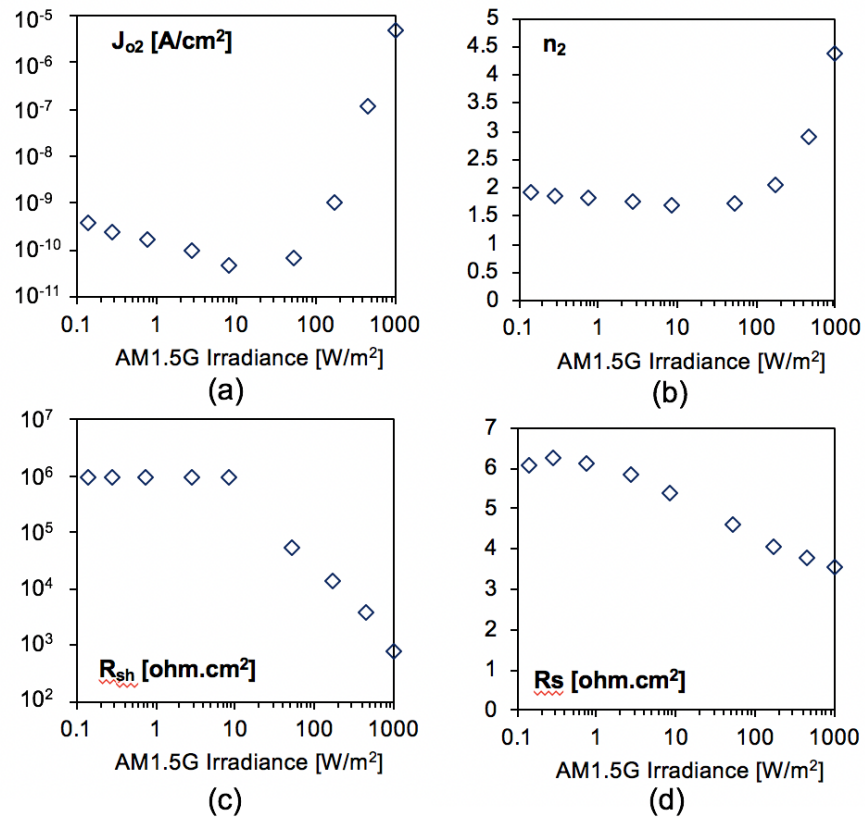
Figure S1: The fitted double diode equation parameters including (a) the reverse saturation current density, J_{o2} , (b) the ideality, (c) shunt resistance, and (d) series resistance.
