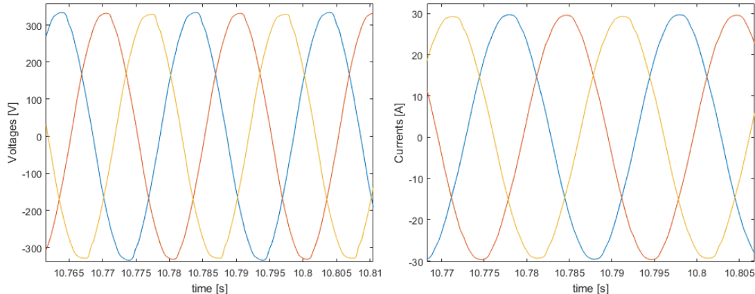
Figure 6: Load voltages and currents during HIL testing
