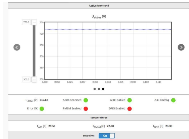
Figure 8: Voltage of the dc bus of the generator connected inverter showing some ripple
