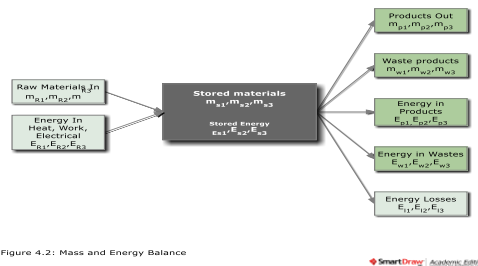
Figure 4: Mass and Energy Balance
