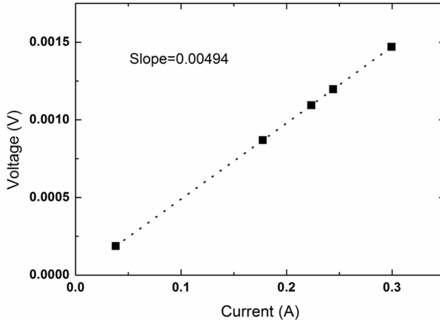
Figure 7. Sheet resistance curve for 1 x 1 \text{cm}^2 square size and 1.02 \mu\text{m} thick Cu film.
