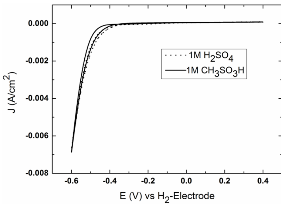
Figure 2. CVs of 1M CH 3 SO 3 H (solid line) and 1M H 2 SO 4 (dotted line) on a GC disc electrode (Conditioning/initial potential: 0.4 V, 20 s; scan rate: 0.01 V/s).
