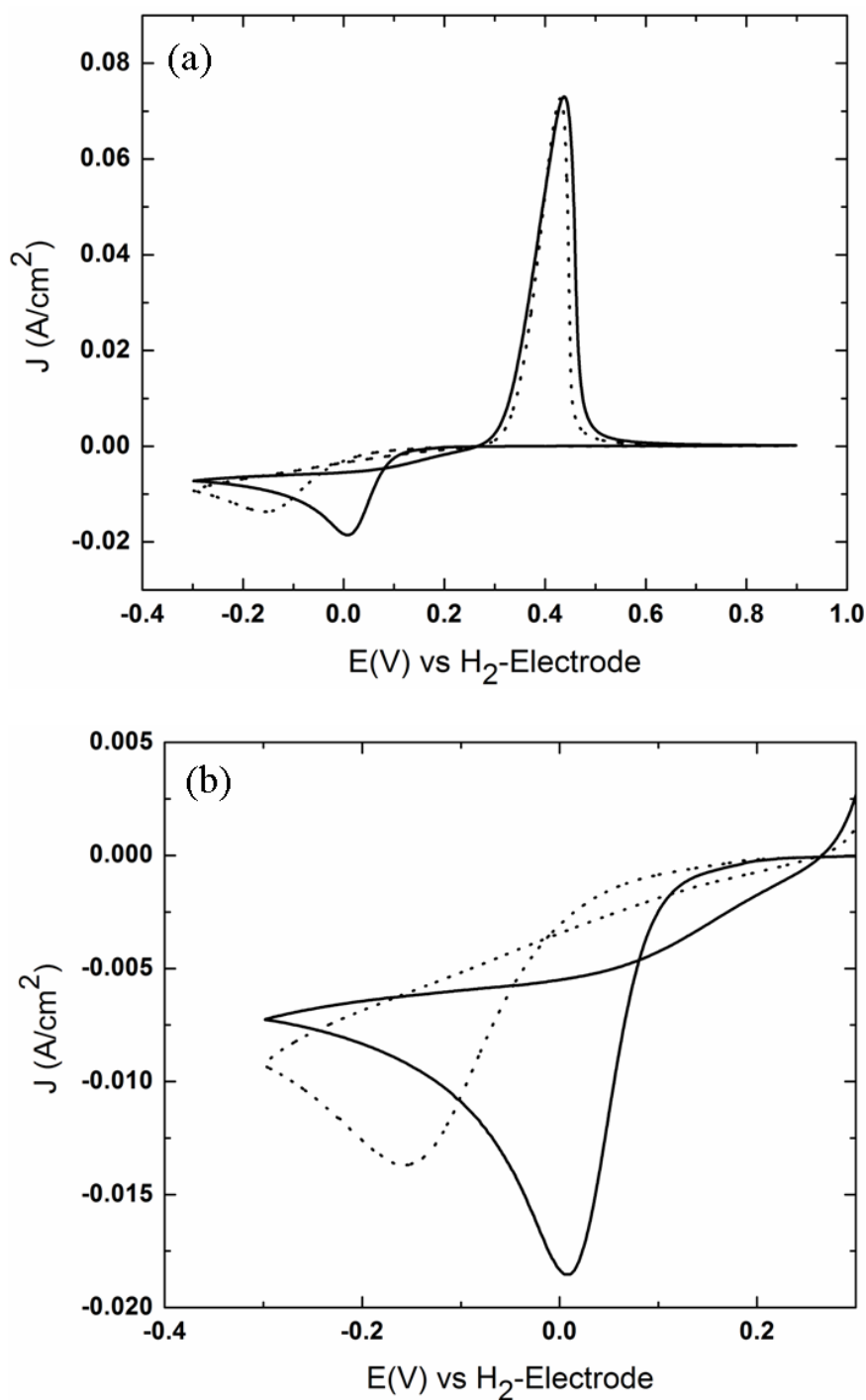
Figure 3. (a) CVs of Cu deposition from methanesulphonate (solid line) and sulphate (dotted line) bath on a GC disc electrode and (b) close-up view of the nucleation loops of copper deposition (Conditioning/initial potential: 0.4 V, 20 s; scan rate: 0.05 V/s).
