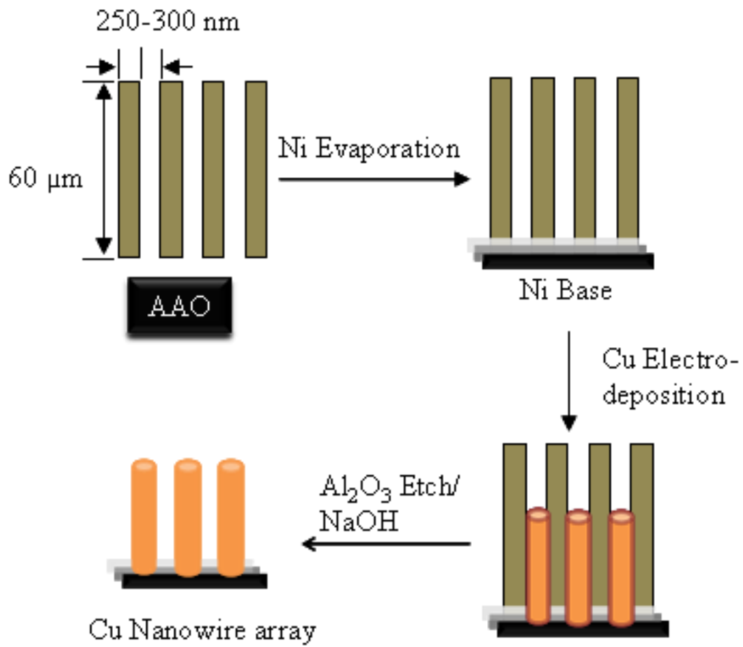
Figure 1. Schematic illustration of the synthesis process of the high aspect ratio Cu nanorod arrays.
