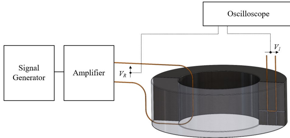
Figure 97. Measurements setup for magnetic flux distribution test.
