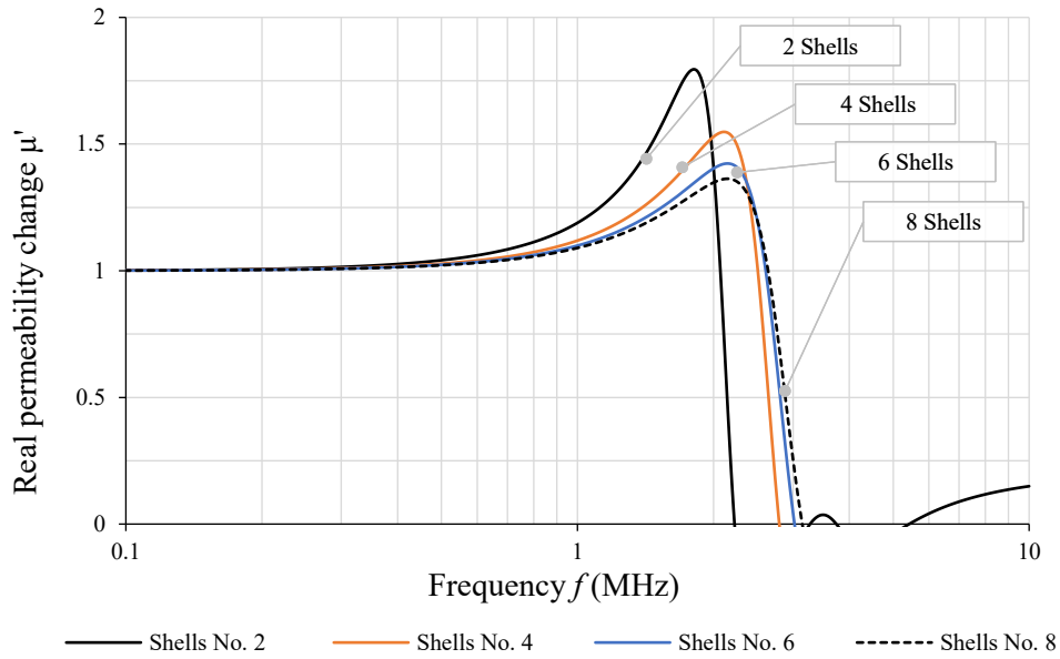
Figure 77. Calculated normalized permeability vs. frequency for T50 3F36 ferrite core for variable shell number.
