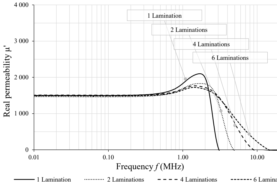
Figure 119. 3F36 ferrite real permeability vs. frequency for various lamination thicknesses.
