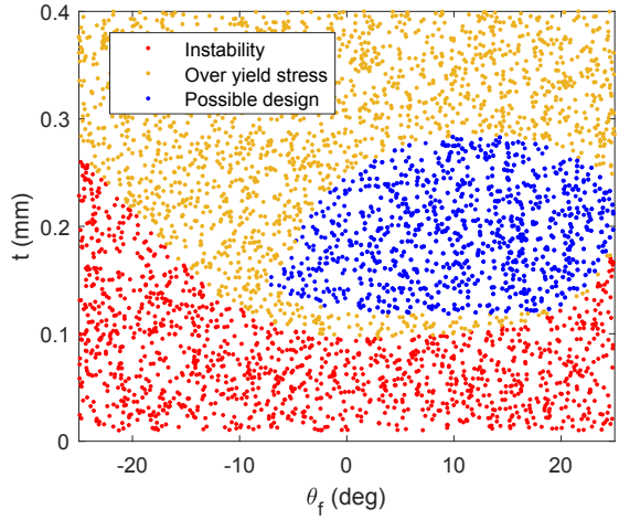
Fig. 10. Design sets for nominal grasping task with flexure yield stress \sigma_y = 690 MPa.
