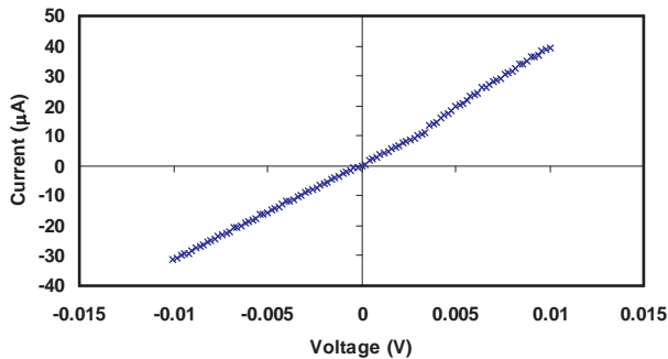
Figure 11. Current vs. voltage curve of the 110 nm line width connected with four 110 μm x 80 μm pads. The features were filled with electrodeposited Cu.
