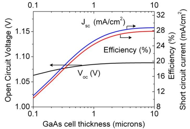
Figure 4: GaAs solar cell electrical characteristics as a function of cell thickness at T = 300 K, 1000 W/m 2 AM1.5d
