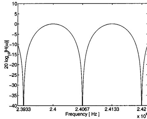
Fig. 8. Magnitude of frequency response of a two-ray multipath channel.
