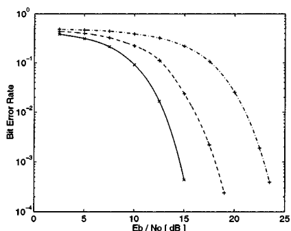
Fig. 15. Performance degradation in an FM-DCSK system caused by channel profile A in the indoor office application. The dashed and dash-dot curves show the best and worst results when the FM-DCSK center frequency is varied. For comparison, the noise performance without multipath (solid curve with “x” marks) is also plotted.
