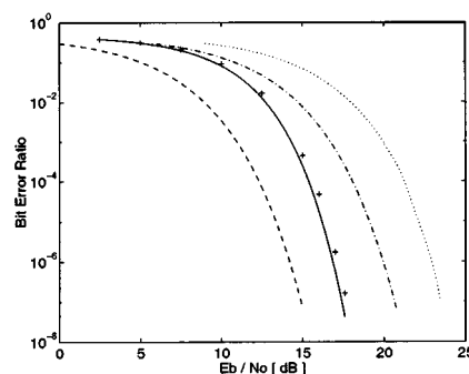
Fig. 6. Noise performance of noncoherent FSK (dashed curve), FM-DCSK and GFSK modulation schemes. For FM-DCSK both the theoretical (solid curve) and simulated (“+” marks) results are plotted. For GFSK the performance is given for two modulation indices: \beta = 0.31 (dash-dot curve) and \beta = 0.22 (dotted curve).
