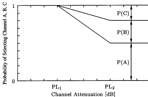
Fig. 14. Probabilities of selecting channel profiles A , B and C as a function of channel attenuation in the JTC multipath channel model.
