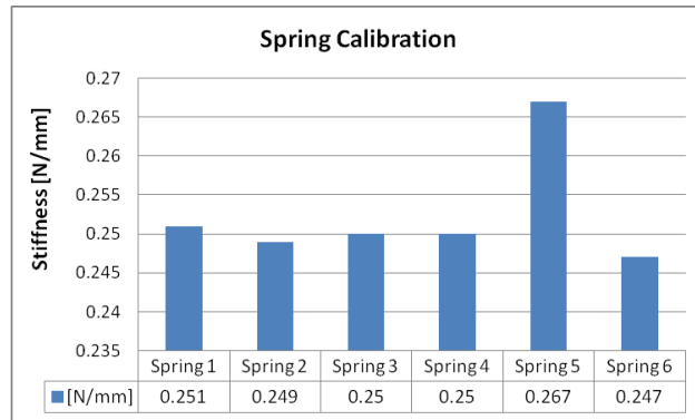
Figure 3 – Calibration of Spring Stiffness.
