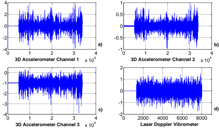
Figure 5 – Time Domain Response from 3D accelerometer: a) Channel 1; b) Channel 2; and c) Channel 3 and d) Laser Doppler Vibrometer (LDV) for sudden change of stiffness.
