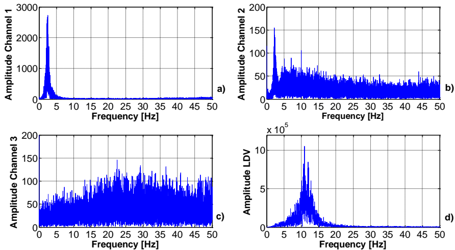
Figure 6 – Frequency Response from 3D accelerometer: a) Channel 1; b) Channel 2; and c) Channel 3 and d) Laser Doppler Vibrometer (LDV) for sudden change of stiffness.
