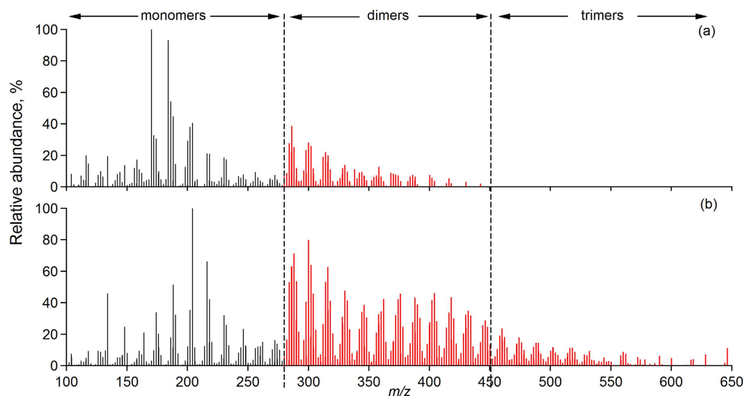
Figure 1. Mass spectra of secondary organic aerosol (SOA) collected at the remote boreal forest site in Hyttiälä, Finland. (a) SOA from samples collected in summer 2011 show only a small number of components in the oligomeric mass region (ions above m/z 280) and no components above m/z 450 where terpene-trimers are observed (see Fig. 2a–c). (b) SOA from samples collected in summer 2014 with clear features in the oligomeric, high molecular mass range up to m/z 600. Red lines correspond to ions in the oligomeric region which intensities have been multiplied by a factor of 5.
