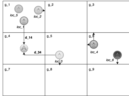
Figure 1: Geohashing
