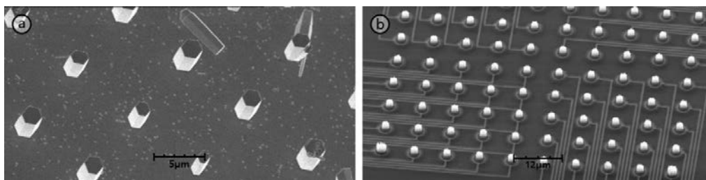
Fig. 1: a - array of single crystalline ZnO nanorods grown by hydrothermal method; b - array of singly bottom contacted ZnO nanorod bunches before polymer encapsulation
