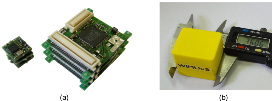
Figure 1. (a) The Tyndall modular Wireless Sensor Network 10mm and 25mm Platform, (b) The Tyndall Smart Wireless Inertial Measurement Unit
