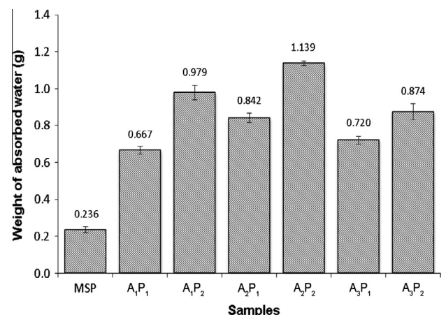
Fig. 5. Mean weight of absorbed water for samples (MSP, A 1 P 1 , A 1 P 2 , A 2 P 1 , A 2 P 2 , A 3 P 1 and A 3 P 2 ) after 10 min.
