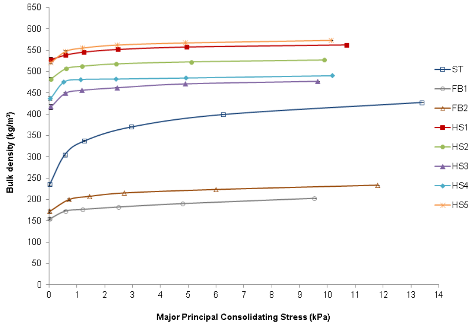
Fig.6-6 Bulk density as a function of major principal consolidating stress for the powders (ST, FB & HS)
