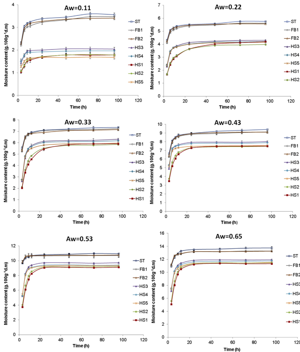
Fig. 4. Kinetics of water vapour adsorption for the powders (ST, FB & HS) at six different hygroscopic environments ( a_w : 0.11; 0.22; 0.33; 0.43; 0.53; 0.65).
