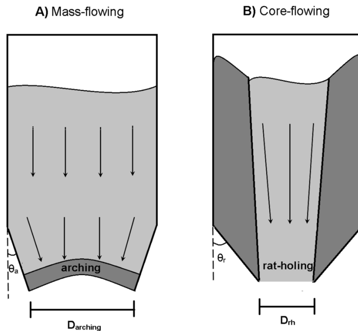
Fig.6-1 Schematically illustration of arching and rat-holing problems in hoppers during A : mass-flowing discharge pattern and B : core-flowing discharge pattern, respectively ( D_{\text{arching}} : minimum outlet diameter to prevent arching; \theta_r : critical hopper
