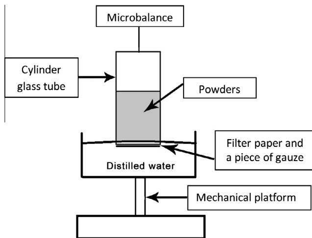
Fig. 2. Scheme of modified Washburn method to quantify the wettability of MPI powders by measuring the weight of adsorbed water (24 °C) in 2 g powders after 10 min.
