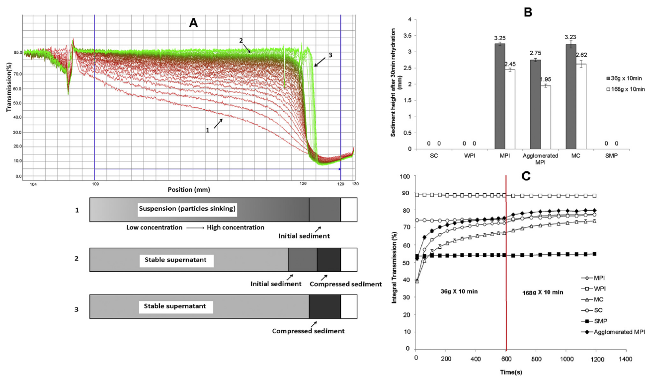
Fig. 7. ABC. A: A schematic illustration explaining the sedimentation behaviour of MPI suspension was showed by the transmission (%) of NIR light through the sample cells by centrifugation time. Profiles were measured every 10 s for first 10 min with 36g centrifugation and every 60 s for next 10 min with 168g centrifugation. Each measurement profile showed the distinct regions corresponding the different positions along the sample cell. The different transmissions represented the regions of dispersed particles and undissolved primary particles, which respectively formed stable supernatant, initial sediment and compressed sediment after centrifugation. Representative profiles based on different time (1: 10 s, 2: 10 min, 3: 20 min) were showed as examples. B: The sediment formed by 1.5% (w/v) sample suspension, which were rehydrated by 400 rpm stirring condition for 30 min at 25 °C distilled water, after 36g and 168g centrifugation for both 10 min. The height of sediment was determined by the regions of low transmission subtracted the steady-state value that caused by cell bottom (from 129 mm). C: Integral transmission was calculated by the software of SepView 4.1 (L.U.M. GmbH, Berlin, Germany). Each integral transmission value (%) represented the overall transmission through the sample cell (from 109 mm to 129 mm) by a function of centrifugation time.
