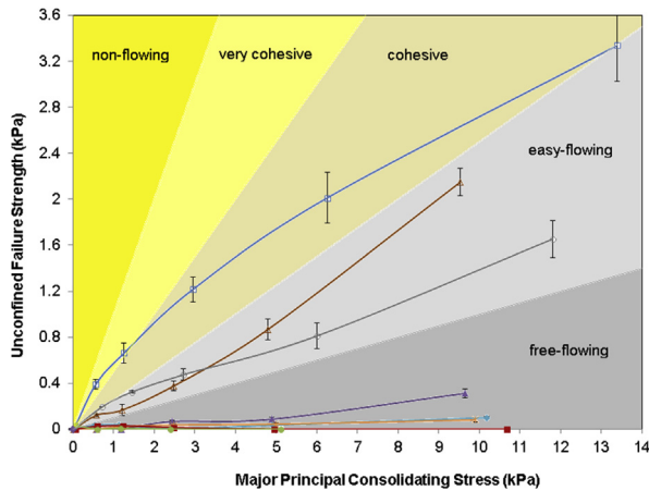
Fig. 5. Flow function curves for unconfined failure strength as a function of major principle consolidation stress for the powders (ST, FB & HS).
