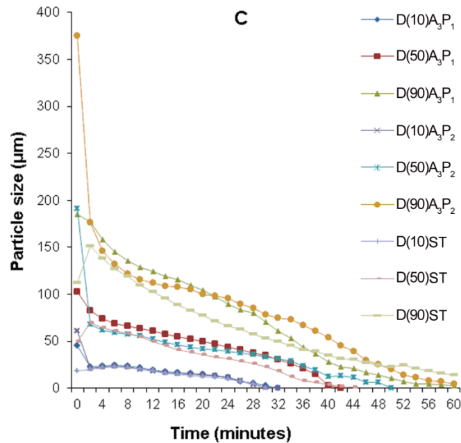
Fig.4-6 ABC Particle size measurement of dispersed particles versus time (every 2 minutes) in 25 \pm 2 °C water at mixing condition of 2000rpm (A= water binding agglomerates and ST; B= lactose solution binding agglomerates and ST; C= sucrose solution binding agglomerates and ST.).
