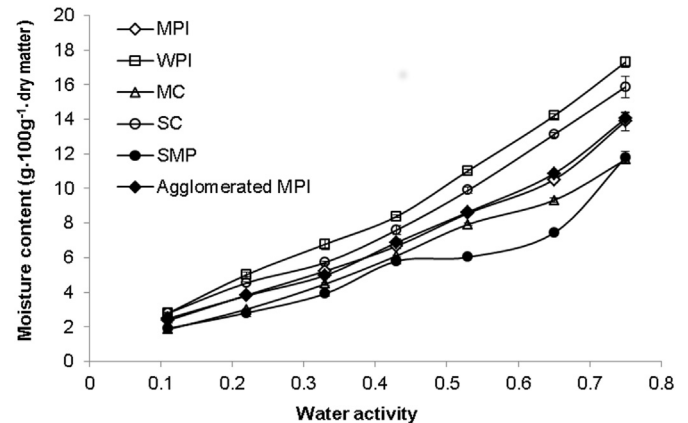
Fig. 3. Water vapour adsorption isotherms of dairy powders (MPI, WPI, MC, SC, SMP and Agglomerated MPI) at 25 °C environment.
