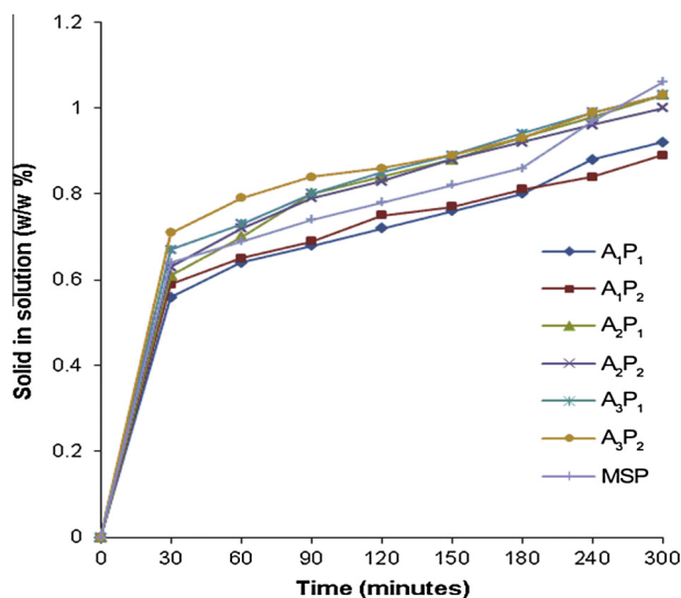
Fig. 7. Solubilisation as measured by dissolved solids concentration (w/w %) versus time (every 30 min) after 10 min 3000 g centrifugation.
