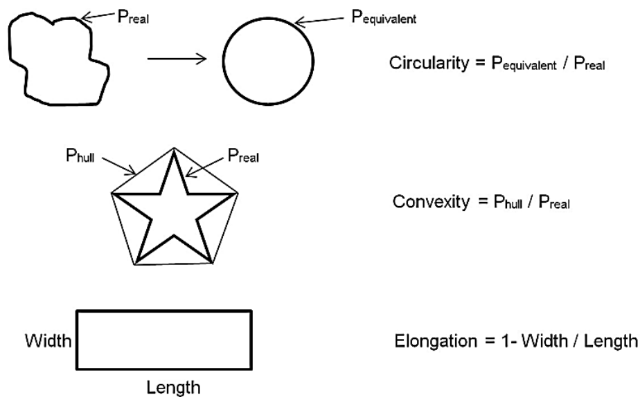
Fig.4-1 Definition of the shapes factors: Circularity, Convexity and Elongation measured by Malvern Morphology G3.
