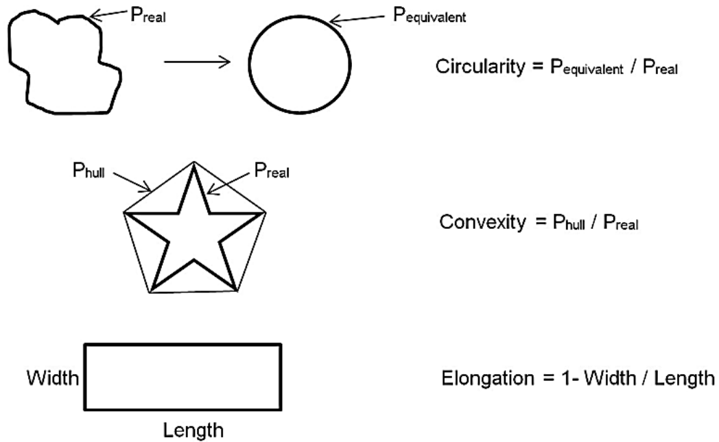
Fig.1-6 Representation of the shapes factors: Circularity, Convexity and Elongation (Ji et al., 2015)
