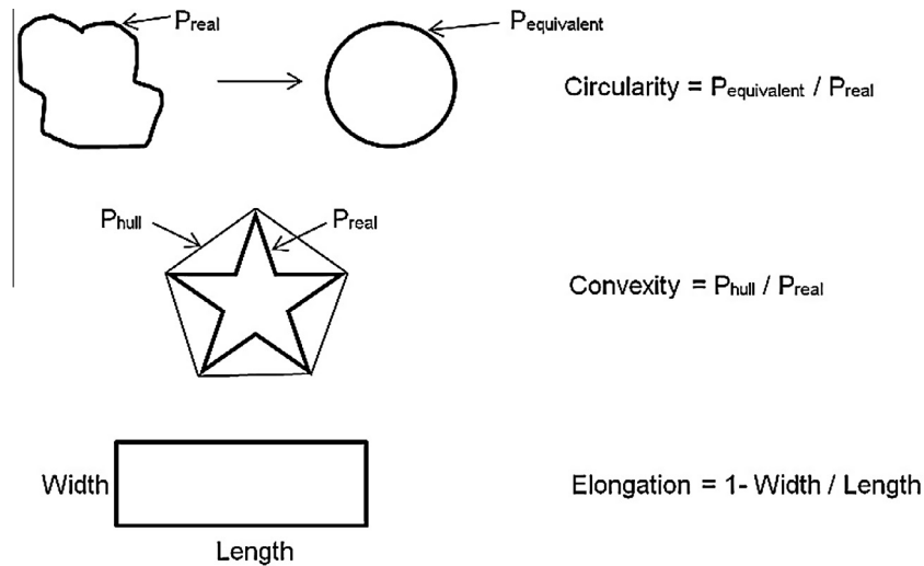
Fig. 1. Definition of the shapes factors: circularity, convexity and elongation measured by Malvern Morphology G3.
