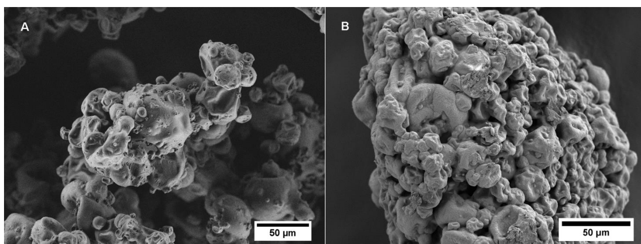
Fig.6-2 SEM Images of MPI granules produced from fluidised bed and high shear mixer granulation, A: Fluidised bed (FB); B: High shear mixer (HS).
