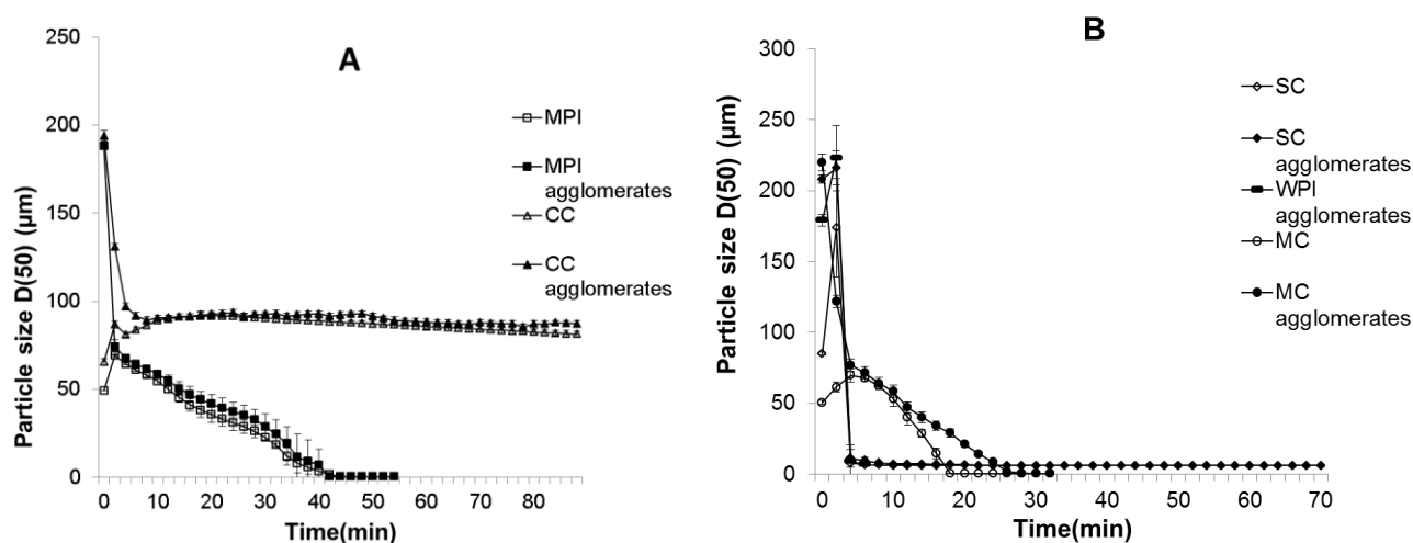
Fig.3-4AB A: Particle size D (50) measurements of dispersed particles of MPI, CC and their agglomerates for every 2 minutes in 25 \pm 2^\circ\text{C} water. B: Particle size D (50) measurements of SC, MC and their agglomerates. (WPI quickly dispersed into water and Mastersizer cannot detect its particle size. Even agglomerated WPI can only be measured for the first 4 minutes)
