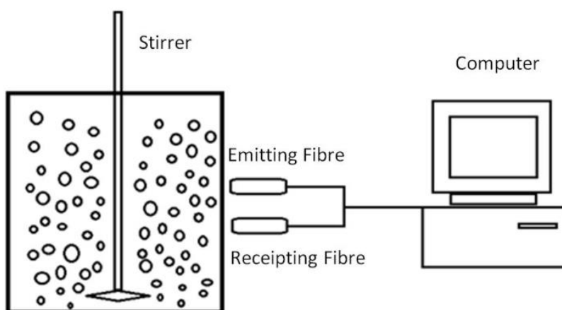
Fig.4-3 Scheme of Light scattering method to quantify the solubilise ability of MPI powders to monitor the particle size of dispersed particles every 2 minutes in 25 \pm 2^\circ\text{C} water at mixing condition of 2000rpm.
