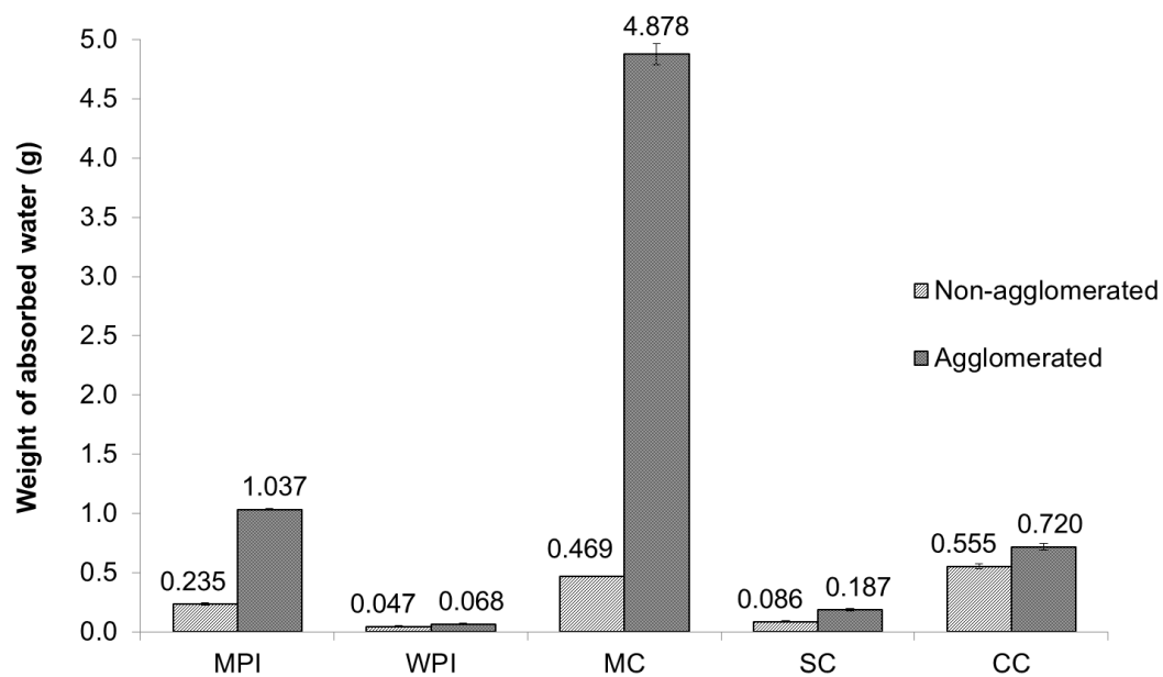
Fig.3-2 Weight of adsorbed water for samples (MPI, WPI, MC, SC, CC and their agglomerates) by capillary rise wetting after 10 minutes.
