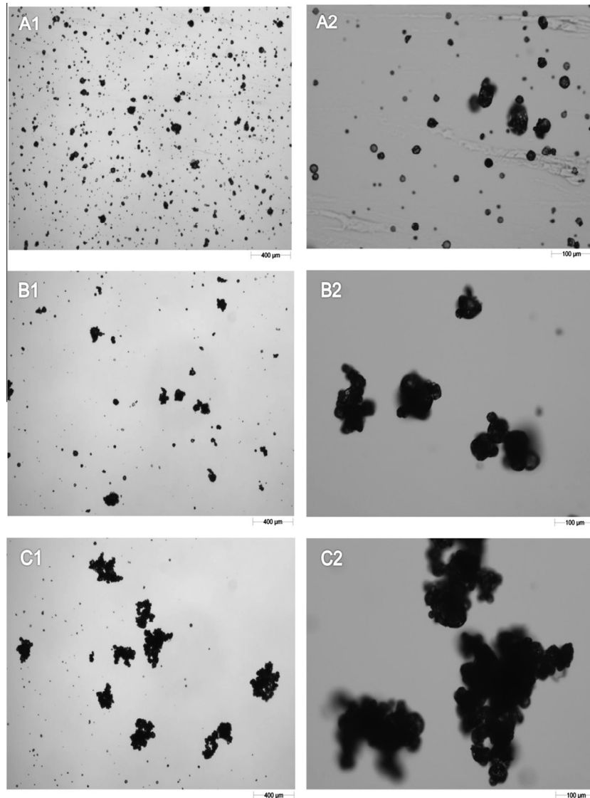
Fig. 4. Comparison of images obtained by Malvern Morphology G3. ( \times 25 , scale = 400 \mu\text{m} ; \times 100 , scale = 100 \mu\text{m} ) (A1 & A2: MPI standard powders; B1 & B2: small size fractions of agglomerates binding with water; C1 & C2: large size fraction of agglomerates binding with water.).
