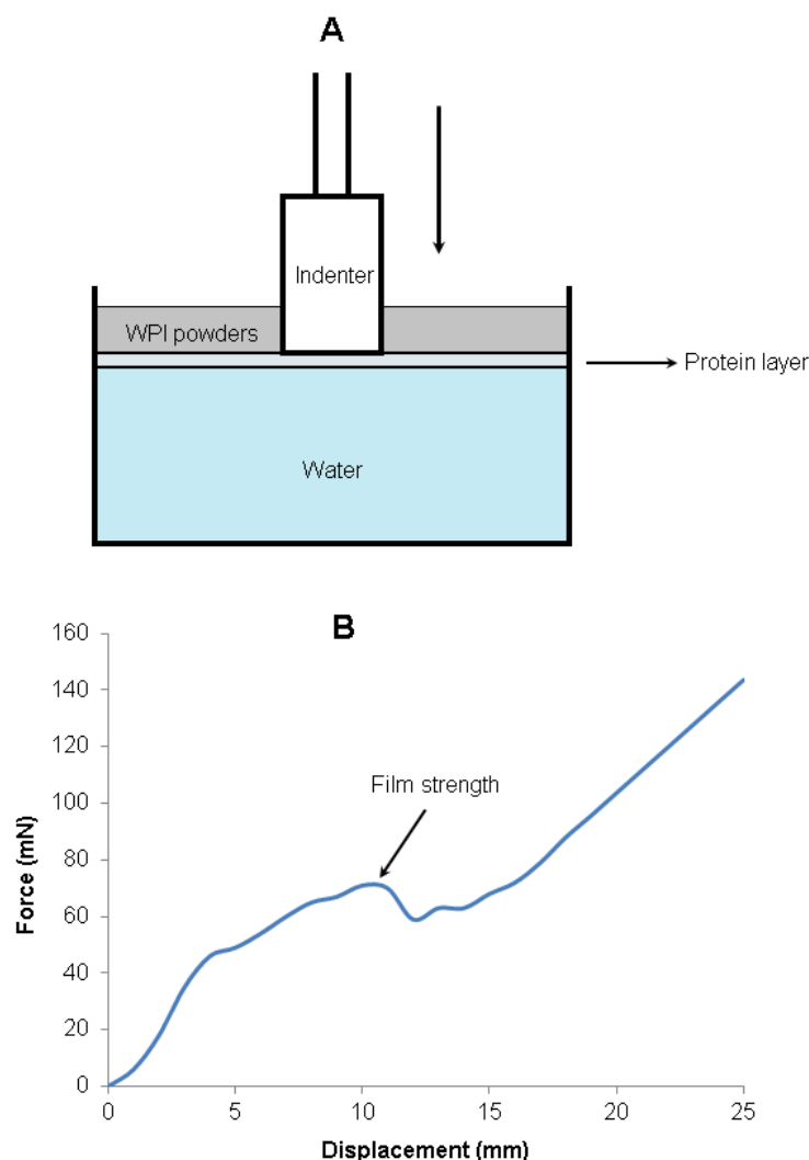
Fig.7-1 Scheme of force-displacement test for the film strength ( A : plunger was moving axially through WPI powders; B : example result of the force-displacement test for standard WPI powder). The noticeable peak appeared in B is the force required to break through the films, which was used as the index of the film strength.
