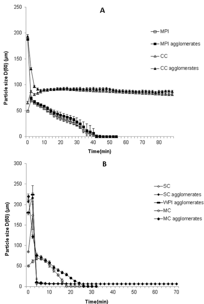
Fig. 4. A: Particle size D (50) measurements of dispersed particles of MPI, CC and their agglomerates for every 2 min in 25 \pm 2 °C water. B: Particle size D (50) measurements of SC, MC and their agglomerates. (WPI quickly dispersed into water and Mastersizer cannot detect its particle size. Even agglomerated WPI can only be measured for the first 4 min).
