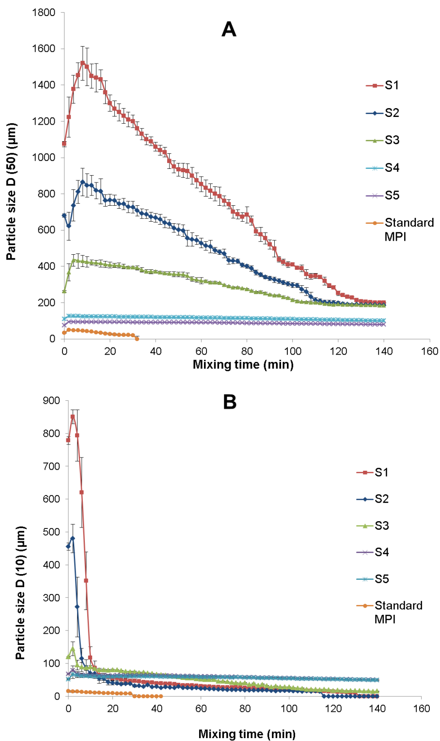
Fig.5-4 Particle size measurements of dispersed particles of the agglomerated granules S1, S2, S3, S4, S5 and standard MPI, as a function of mixing time (every 2 minutes) A: D (50); B: D (10).
