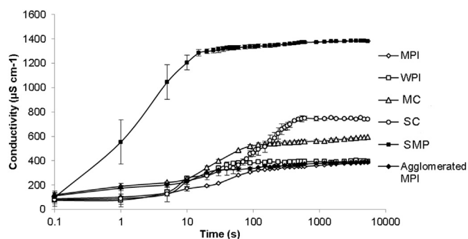
Fig. 8. The change of conductivity by a function of mixing time for the 2% (w/v) concentration sample suspension, with 500 rpm stirring condition at 25 °C. (Distilled water was used in suspension, which had conductivity value of 67 \mu\text{S cm}^{-1} .)
