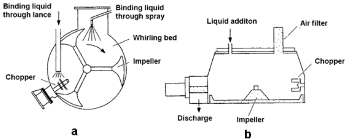
Fig. 1-2 (a) Horizontal and (b) vertical high-shear mixer granulators (Reynolds et al., 2006)
