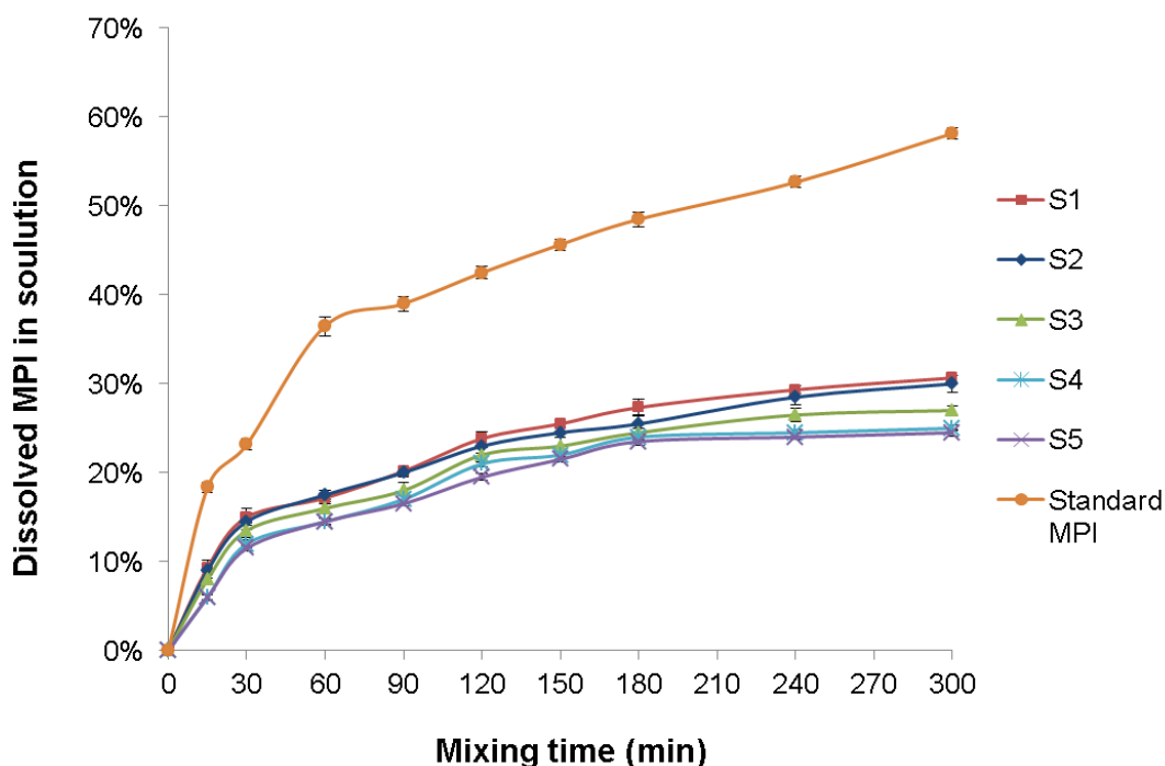
Fig.5-5. Solubilisation as measured by dissolved MPI percentage (%) versus different mixing time.
