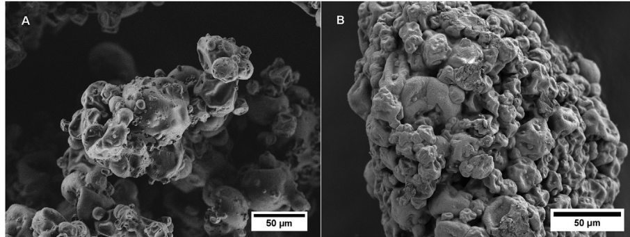
Fig. 2. SEM Images of MPI granules produced from fluidised bed and high shear mixer granulation, A: Fluidised bed (FB); B: High shear mixer (HS).
