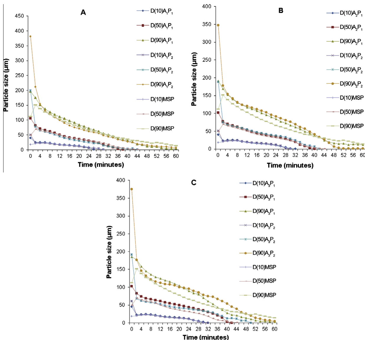
Fig. 6. Particle size measurement of dispersed particles versus time (every 2 min) in 25 \pm 2 °C water at mixing condition of 2000 rpm (A = water binding agglomerates and MSP; B = lactose solution binding agglomerates and MSP; C = sucrose solution binding agglomerates and MSP.).
