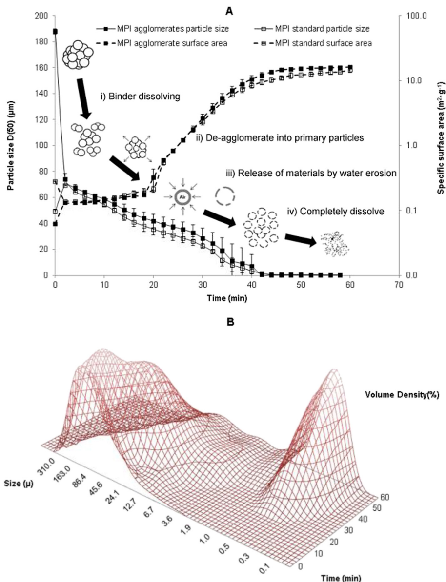
Fig. 5. A: Schematic of MPI and agglomerated MPI particles rehydration in water, based on the change of particle size D (50) and specific surface area as a function of time. B: Volume density (%) based size distributions of dispersing MPI particles measured as a function of time. It showed the volume concentration of both undissolved and dissolved powder particles.
