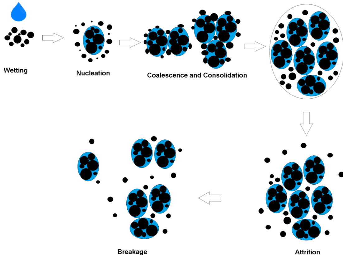
Fig.1-5 Different rate processes in agglomeration (a) wetting and nucleation; (b) Coalescence and consolidation; (c) breakage and attrition
