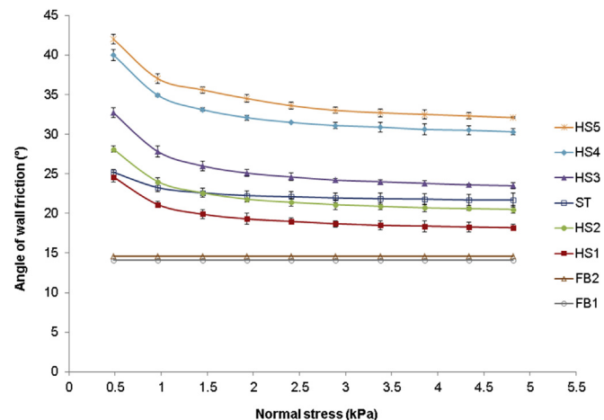
Fig. 7. The angles of wall friction as a function of normal stress for the powders (ST, FB & HS).
