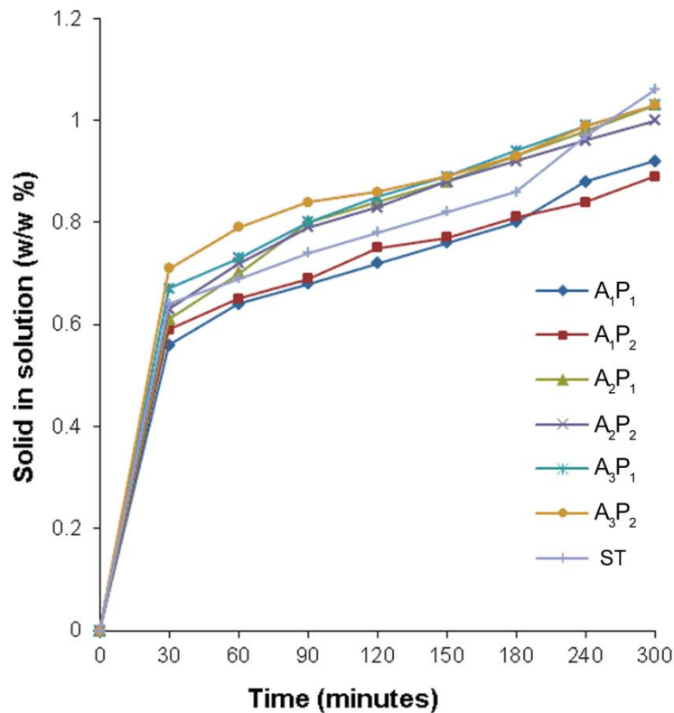
Fig.4-7 Solubilisation as measured by dissolved solids concentration (w/w %) versus time (every 30 minutes) after 10 minutes 3000g centrifugation
