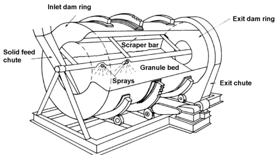
Fig.1-3 The rolling drum granulator (Litster and Ennis, 2013)
