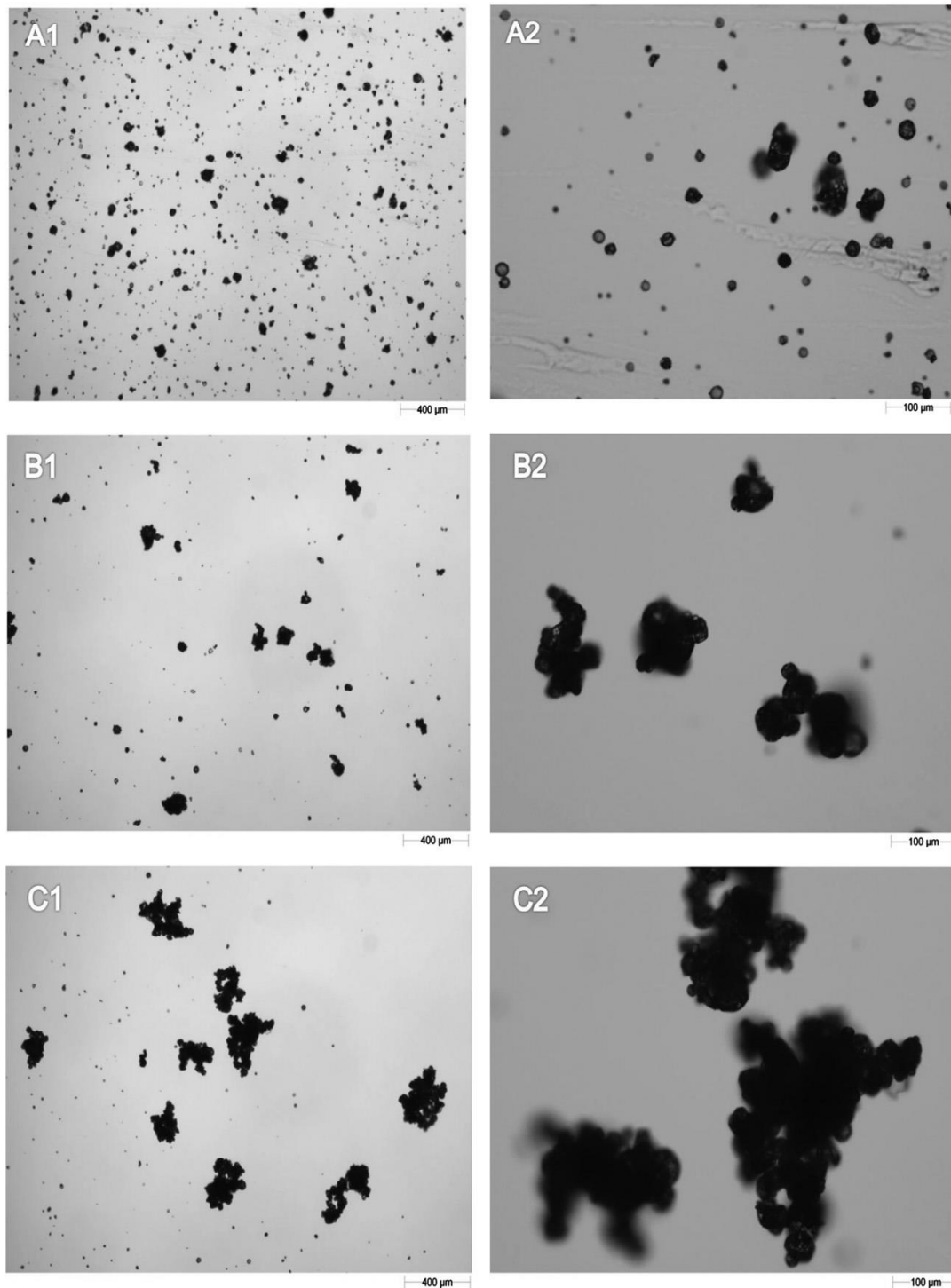
Fig.4-4 Comparison of images obtained by Malvern Morphology G3. (x25, scale =400μm; x100, scale = 100 μm) (A1 & A2: MPI standard powders; B1 & B2: small size fractions of agglomerates binding with water; C1 & C2: large size fraction of agglomerates binding with water.)
