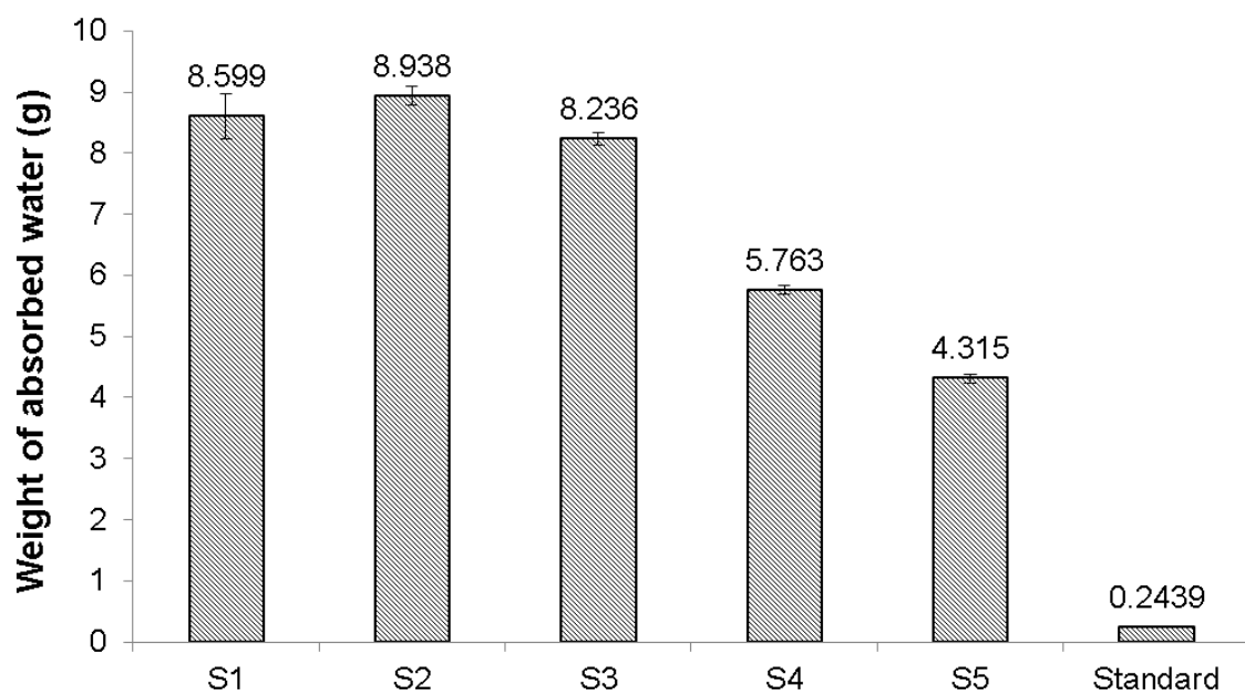
Fig.5-2 Mean weight of absorbed water for samples (the agglomerated MPI granules S1, S2, S3, S4, S5 and standard MPI) after 10 minutes
