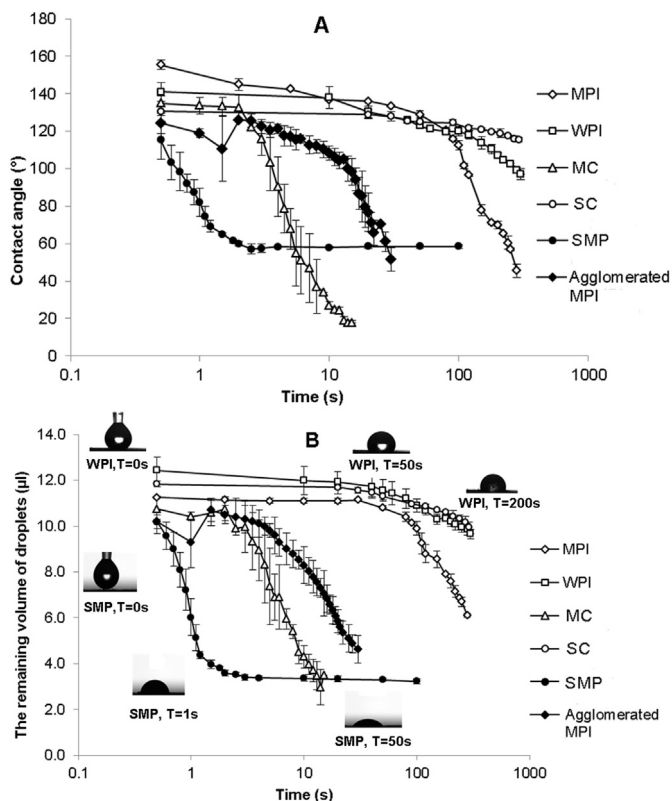
Fig. 4. AB. A: The change of contact angle ( ^\circ ) as a function of time using the sessile drop technique in approx. 20^\circ\text{C} temperature. B: The change in the volume of droplet ( \mu\text{L} ) above the solids as a function of time during the wetting process in approx. 20^\circ\text{C} temperature. The initial volume of water droplet was approx. 12\ \mu\text{L} .
