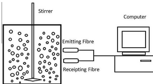
Fig. 3. Scheme of Light scattering method to quantify the solubilise ability of MPI powders to monitor the particle size of dispersed particles every 2 min in 25 ± 2 °C water at mixing condition of 2000 rpm.
