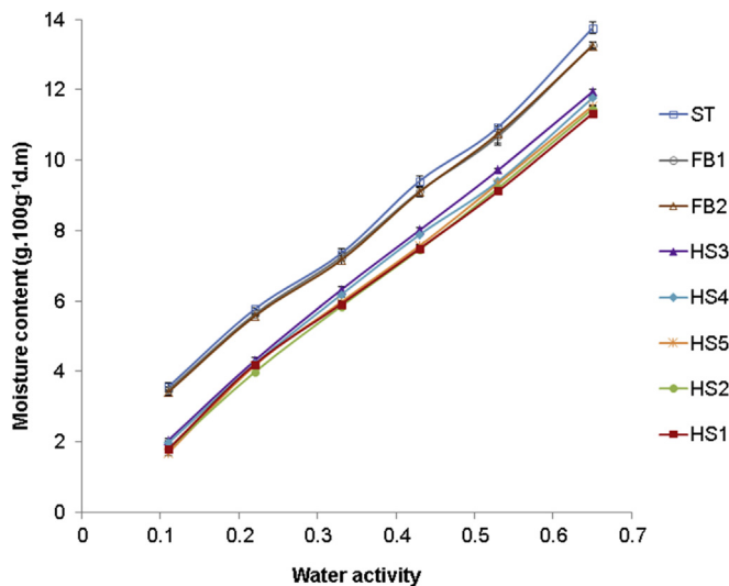
Fig. 3. Water vapours adsorption isotherms of powders (ST, FB & HS) at 25 °C environment.
