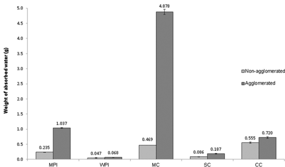
Fig. 2. Weight of adsorbed water for samples (MPI, WPI, MC, SC, CC and their agglomerates) by capillary rise wetting after 10 min.
