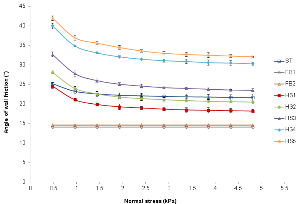
Fig.6-7 The angles of wall friction as a function of normal stress for the powders (ST, FB & HS)
