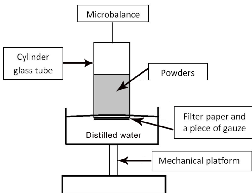
Fig.4-2 Scheme of modified Washburn method to quantify the wettability of MPI powders by measuring the weight of adsorbed water (24°C) in 2g powders after 10 minutes.
