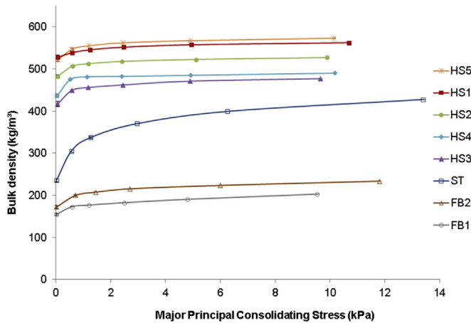
Fig. 6. Bulk density as a function of major principal consolidating stress for the powders (ST, FB & HS).
