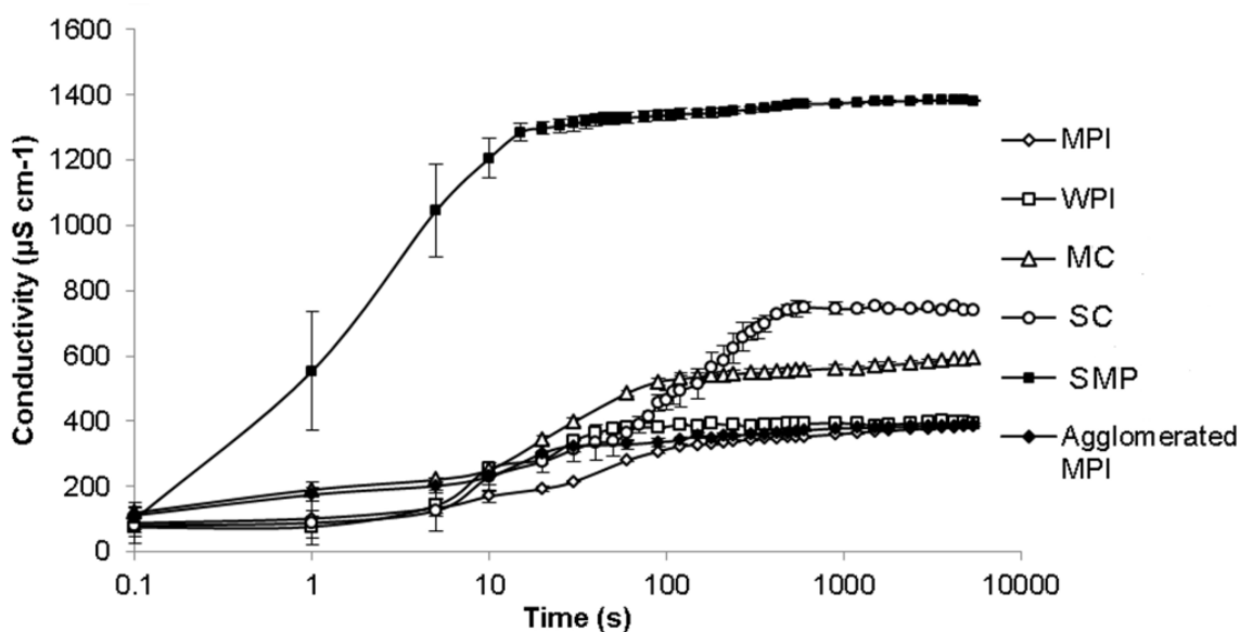
Fig.2-8. The change of conductivity by a function of mixing time for the 2% (w/v) concentration sample suspension, with 500 rpm stirring condition at 25 °C. (Distilled water was used in suspension, which had conductivity value of 67 \mu\text{S}\cdot\text{cm}^{-1} .)
