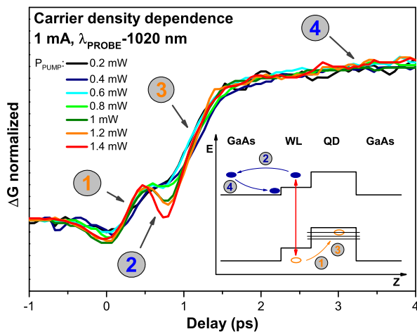
FIG. 4. Normalized first few ps of gain dynamics for increasing pump power level. Inset: schematic of various carrier transport/relaxation processes corresponding to gain changes labeled on main graph.
